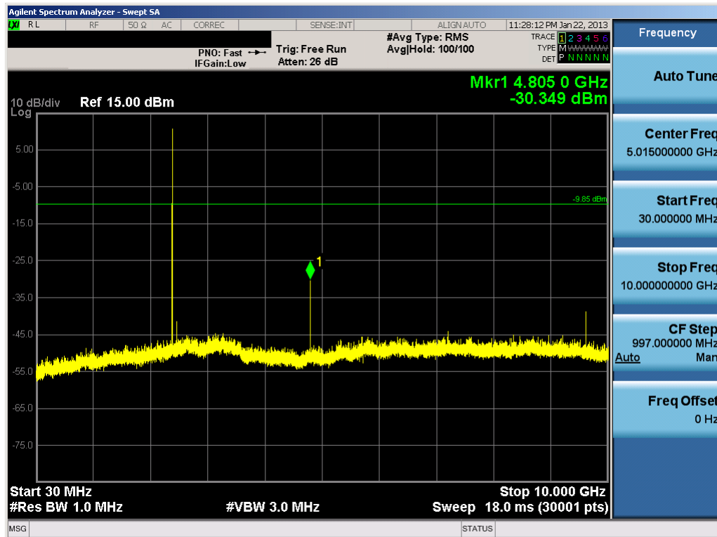
Plot 6-36. Conducted Spurious Plot (Bluetooth, 2Mbps – Ch. 0)
