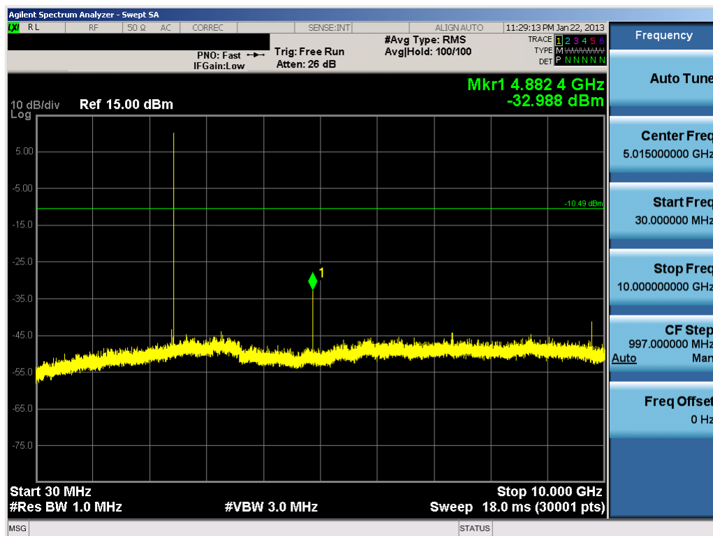
Plot 6-38. Conducted Spurious Plot (Bluetooth, 2Mbps – Ch. 39)
