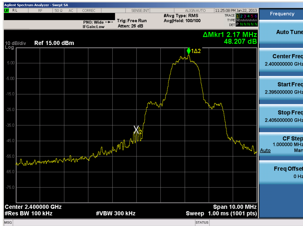
Plot 6-28. Band Edge Plot (Bluetooth with Hopping Disabled, 2Mbps – Ch. 0)
