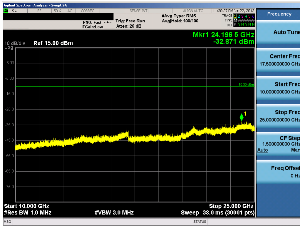
Plot 6-41. Conducted Spurious Plot (Bluetooth, 2Mbps – Ch. 78)
