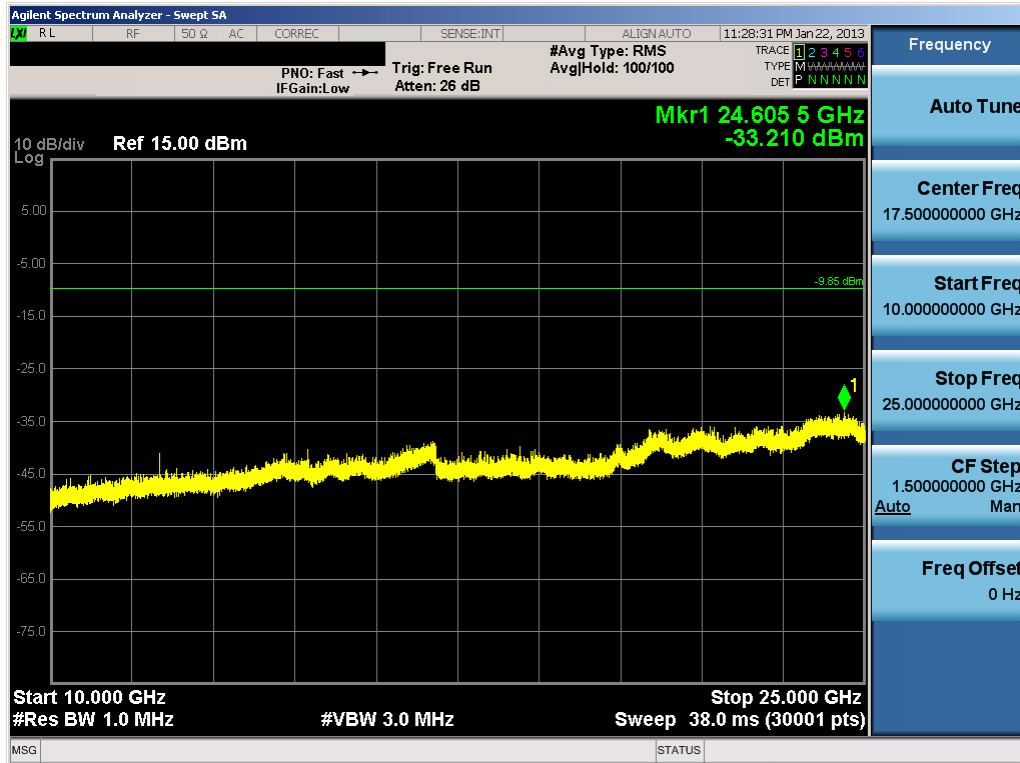
Plot 6-37. Conducted Spurious Plot (Bluetooth, 2Mbps – Ch. 0)
