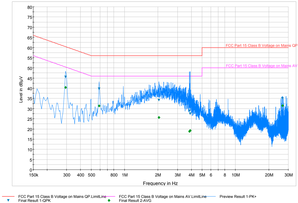
Plot 6-44. Line-Conducted Test Plot (L1)
