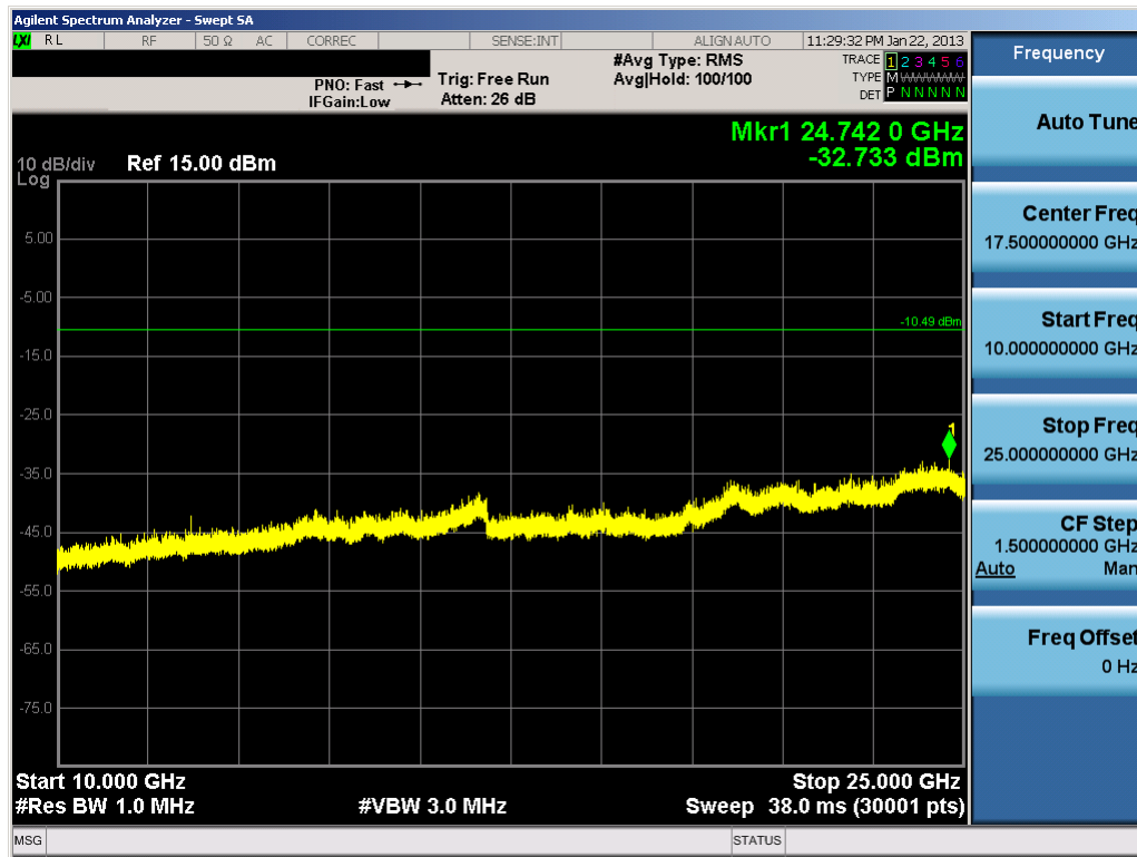
Plot 6-39. Conducted Spurious Plot (Bluetooth, 2Mbps – Ch. 39)
