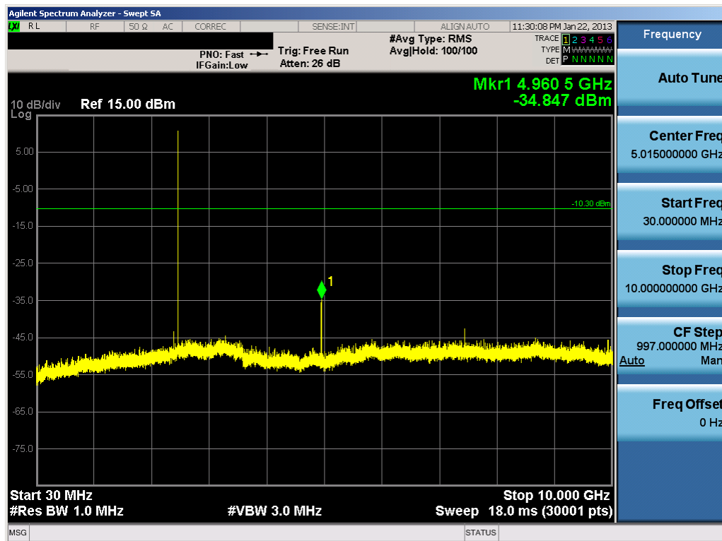
Plot 6-40. Conducted Spurious Plot (Bluetooth, 2Mbps – Ch. 78)
