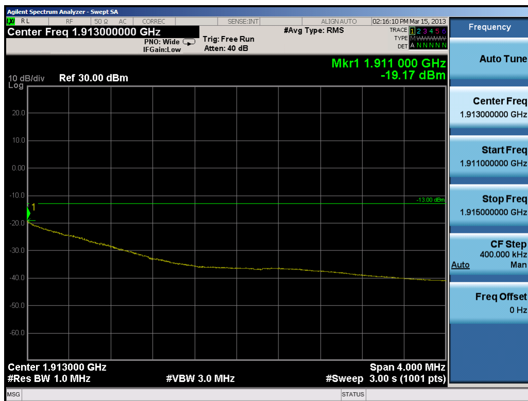
Plot 7-35. 4MHz Span Plot (PCS CDMA Mode – Ch. 1175)
