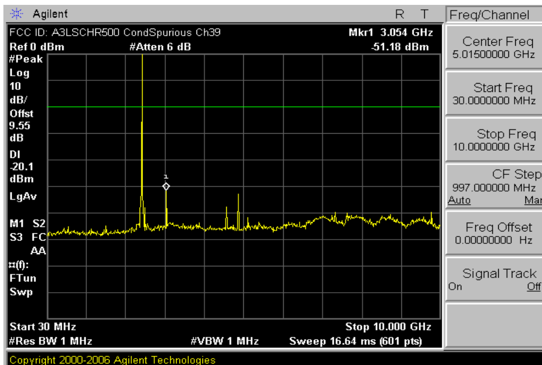
Plot 6-12. Conducted Spurious Plot (Bluetooth – Ch. 39)
