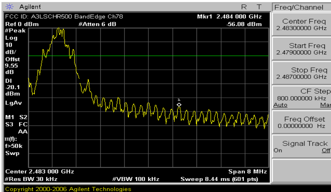
Plot 6-5. Band Edge Plot (Bluetooth – Ch. 78)
