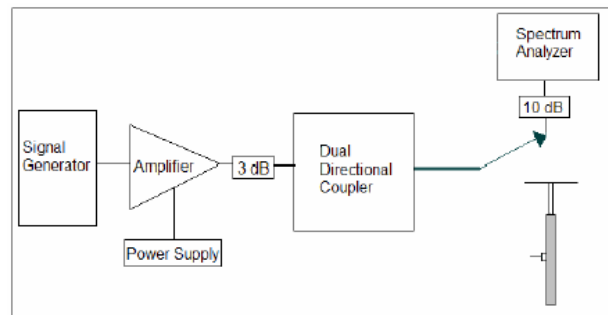
Figure 8.2 Setup to Peak Power using Spectrum Analyzer
