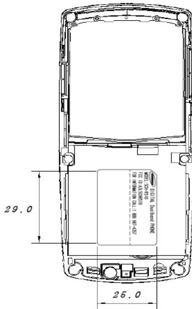
Figure A-2. FCC ID Label Location
