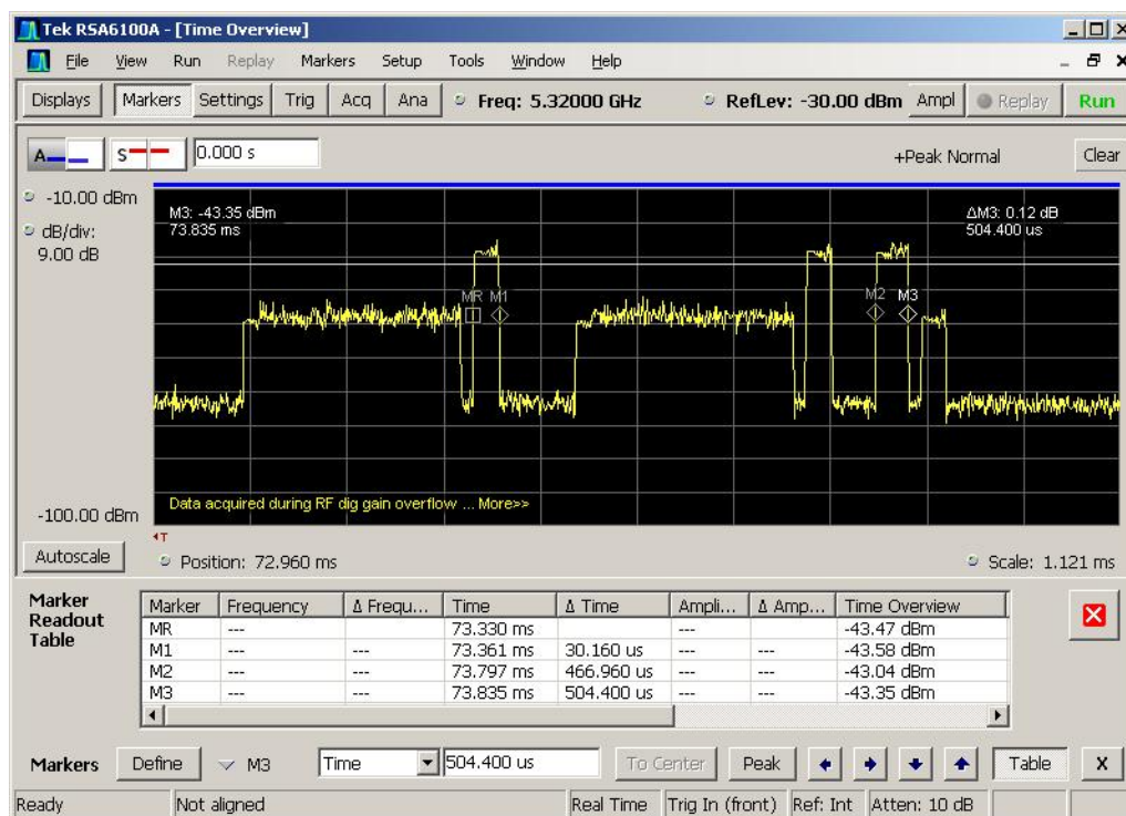
Figure 6-6. Pulse Width After 200ms
