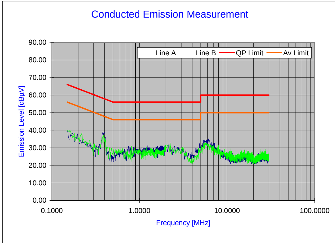
Plot 6-24. Line Conducted Plot with Bluetooth
