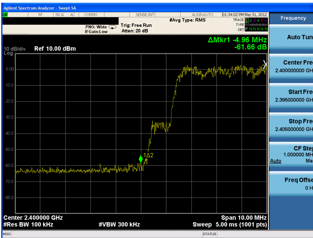
Plot 6-12. Band Edge Plot (Bluetooth with Hopping Enabled, 1Mbps)
