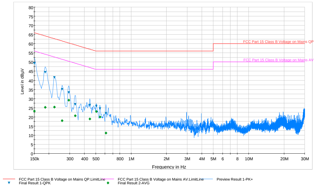
Plot 7-1. Line Conducted Plot (L1)
