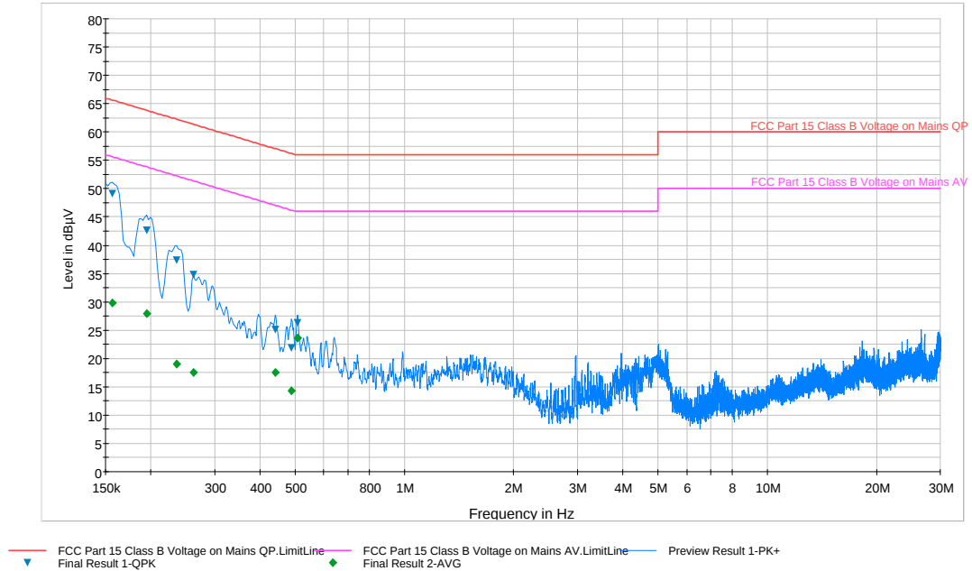
Plot 7-2. Line Conducted Plot (LN)
