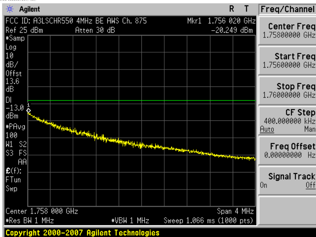
Plot 7-11. 4MHz Span Plot (AWS CDMA Mode – Ch. 875)
