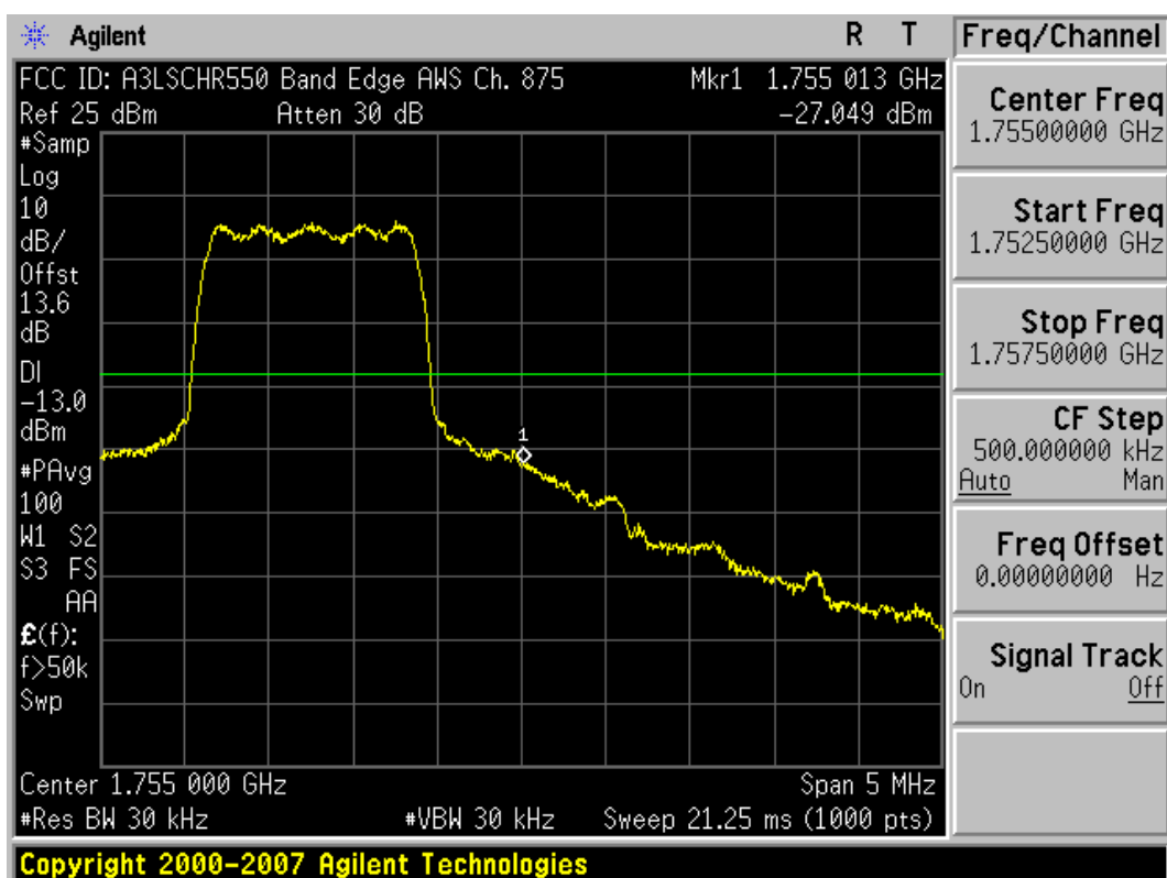
Plot 7-10. Band Edge Plot (AWS CDMA Mode – Ch. 875)
