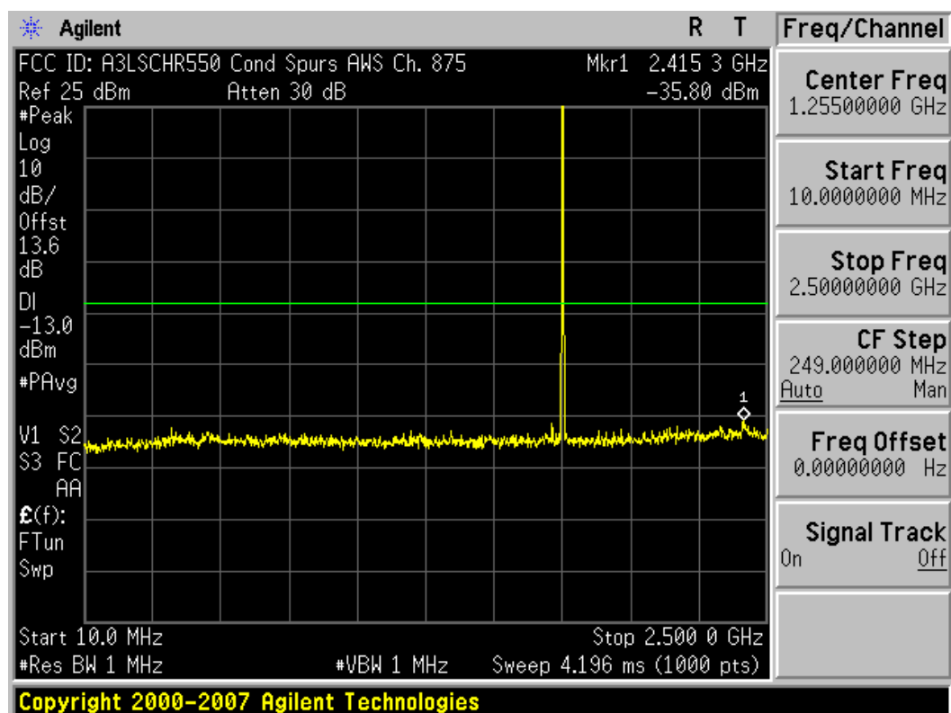
Plot 7-8. Conducted Spurious Plot (AWS CDMA Mode – Ch. 875)
