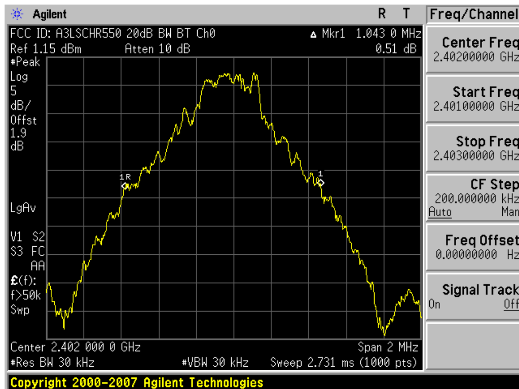
Plot 6-1. 20dB Bandwidth Plot (Bluetooth 2.0 – Ch. 0)
