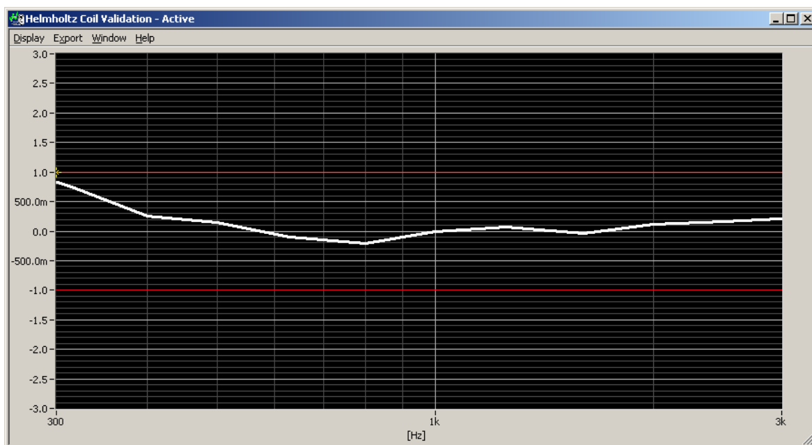
Figure 6-3 Helmholtz Coil Validation for Frequency Response
