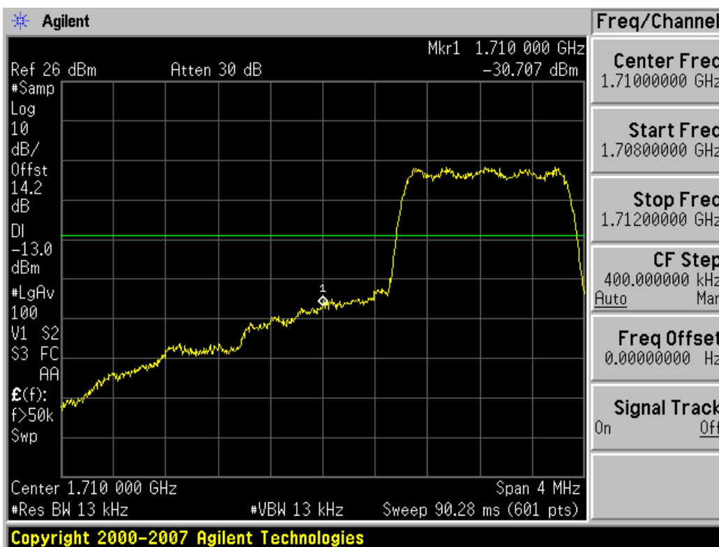
Plot 7-14. Band Edge Plot (AWS CDMA Mode – Ch. 25)
