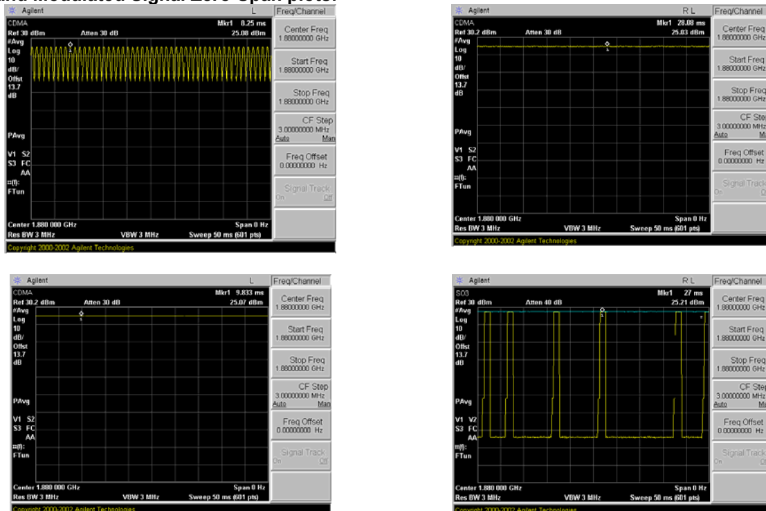
Figure 8-4 Zero-Span Plots
