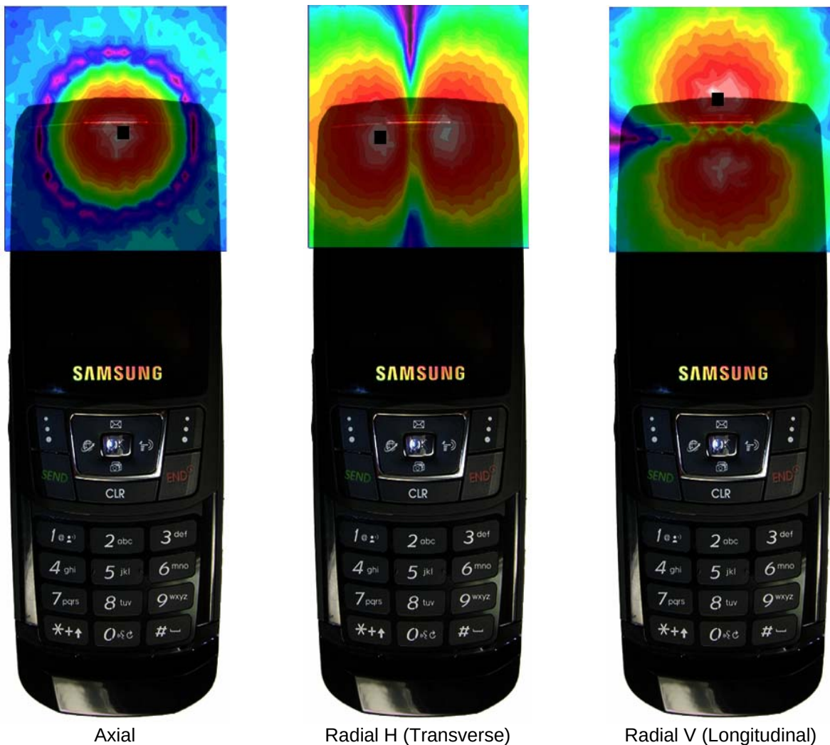
Figure 13-3 T-Coil Scan Overlay Magnetic Field Distributions
