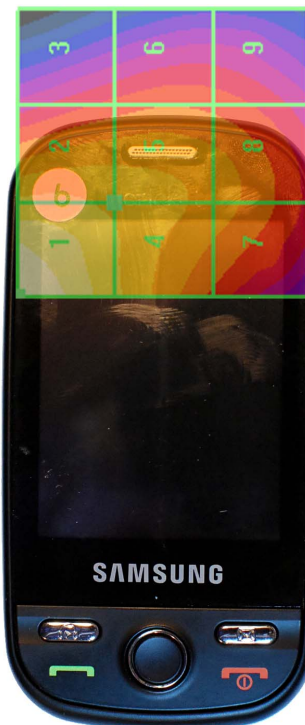
Figure 17-5 H-Field WD Scan overlay
