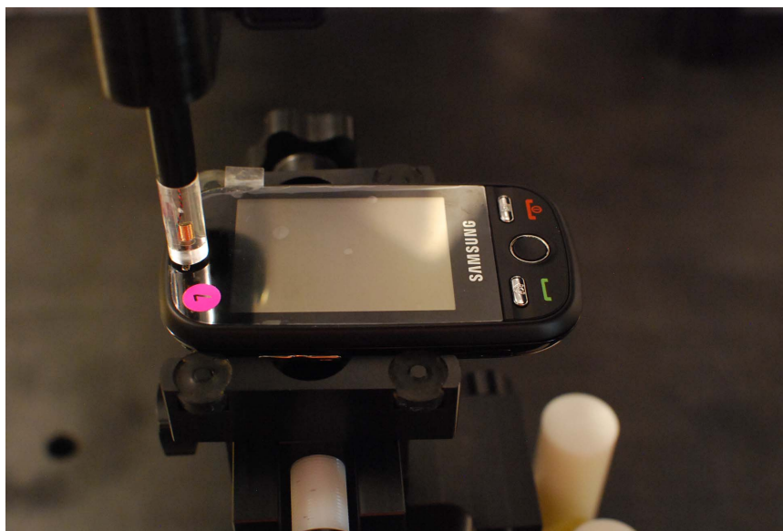
Figure 13-2 Test Setup for Wireless Device
