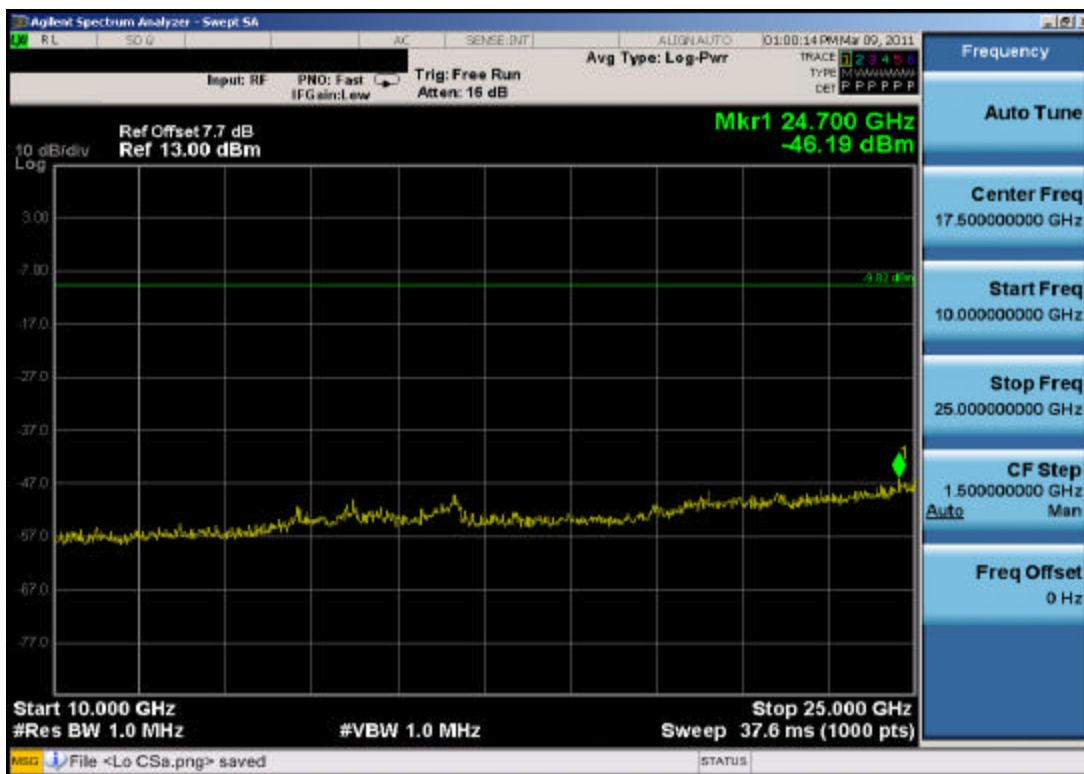
Plot 6-19. Conducted Spurious Plot (Bluetooth, 2Mbps – Ch. 0)
