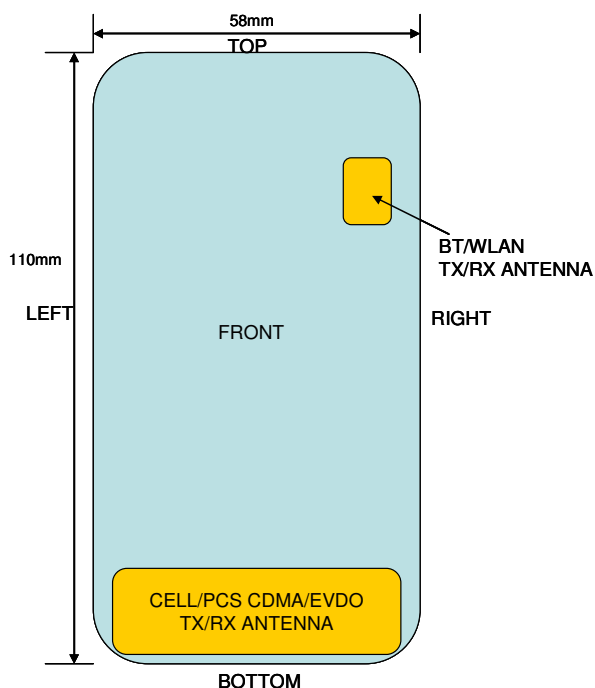
Figure 13-1 Identification of Sides for SAR Testing
