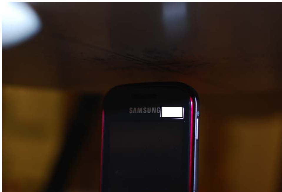
SAR Test Setup Photo 7 – Body Top at 1.0 cm
