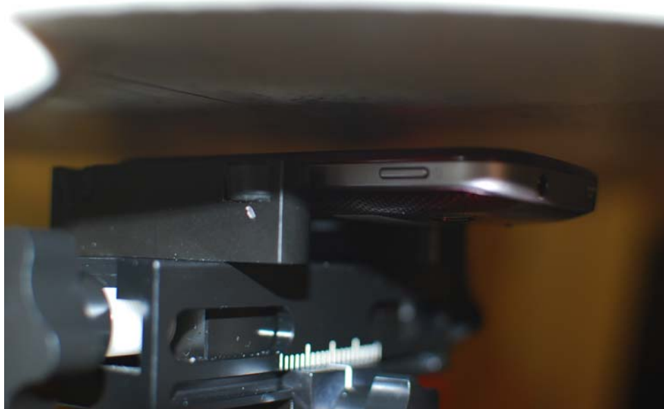
SAR Test Setup Photo 6 – Body Front at 1.0 cm
