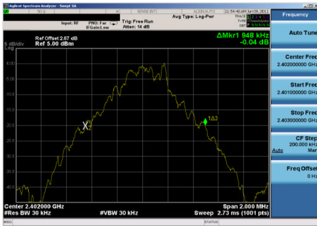
Plot 6-1. 20dB Bandwidth Plot (Bluetooth, 1Mbps – Ch. 0)
