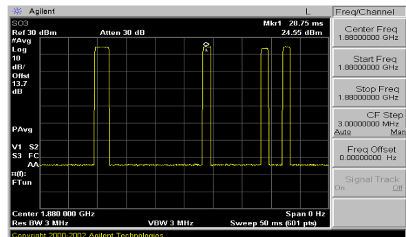
Figure 8-4 Zero-Span Plots
