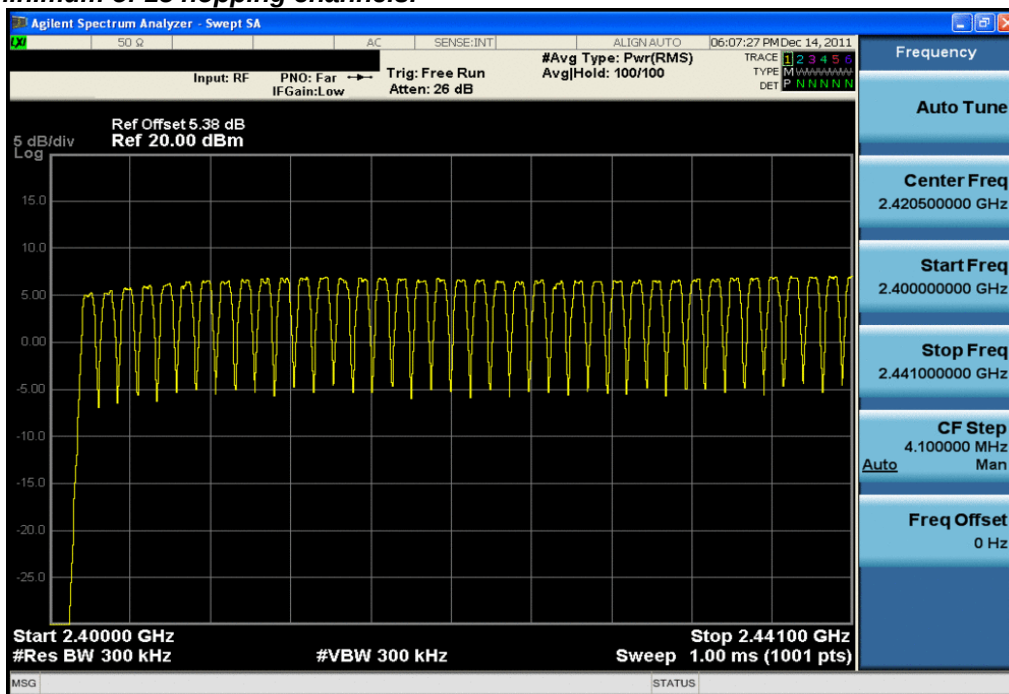
Plot 6-14. Low End Spectrum Channel Hopping Plot (Bluetooth)
