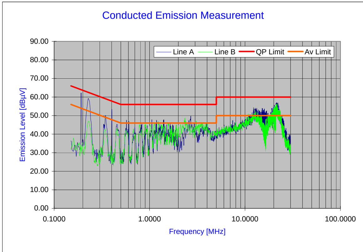
Plot 6-22. Line Conducted Plot with Bluetooth
