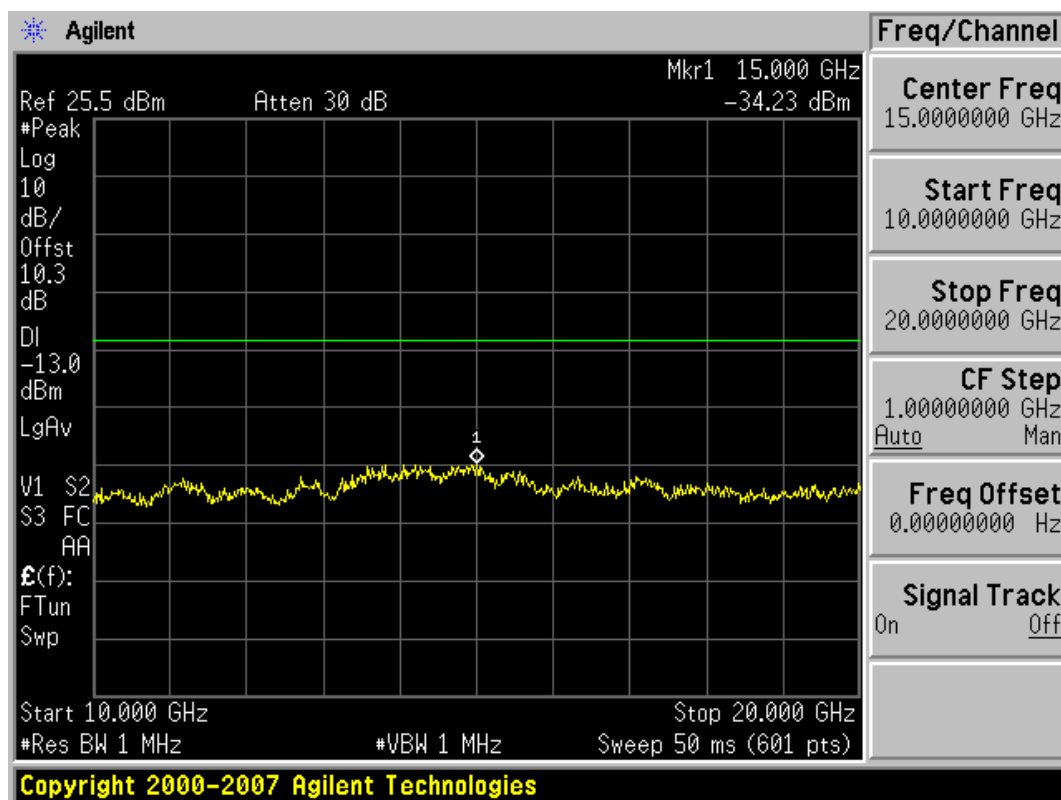
Plot 7-10. Conducted Spurious Plot (AWS CDMA Mode – Ch. 875)
