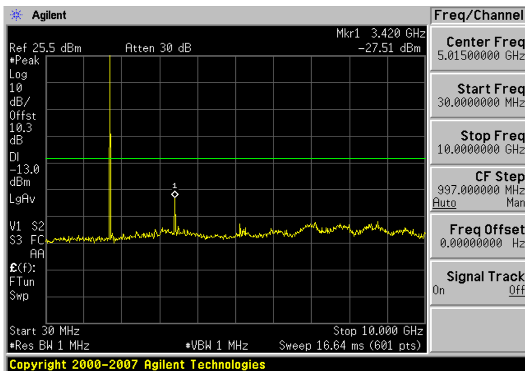
Plot 7-1. Conducted Spurious Plot (AWS CDMA Mode – Ch. 25)
