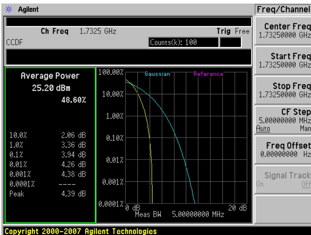
Plot 7-8. Peak-Average Ratio Plot (AWS CDMA Mode – Ch. 450)
