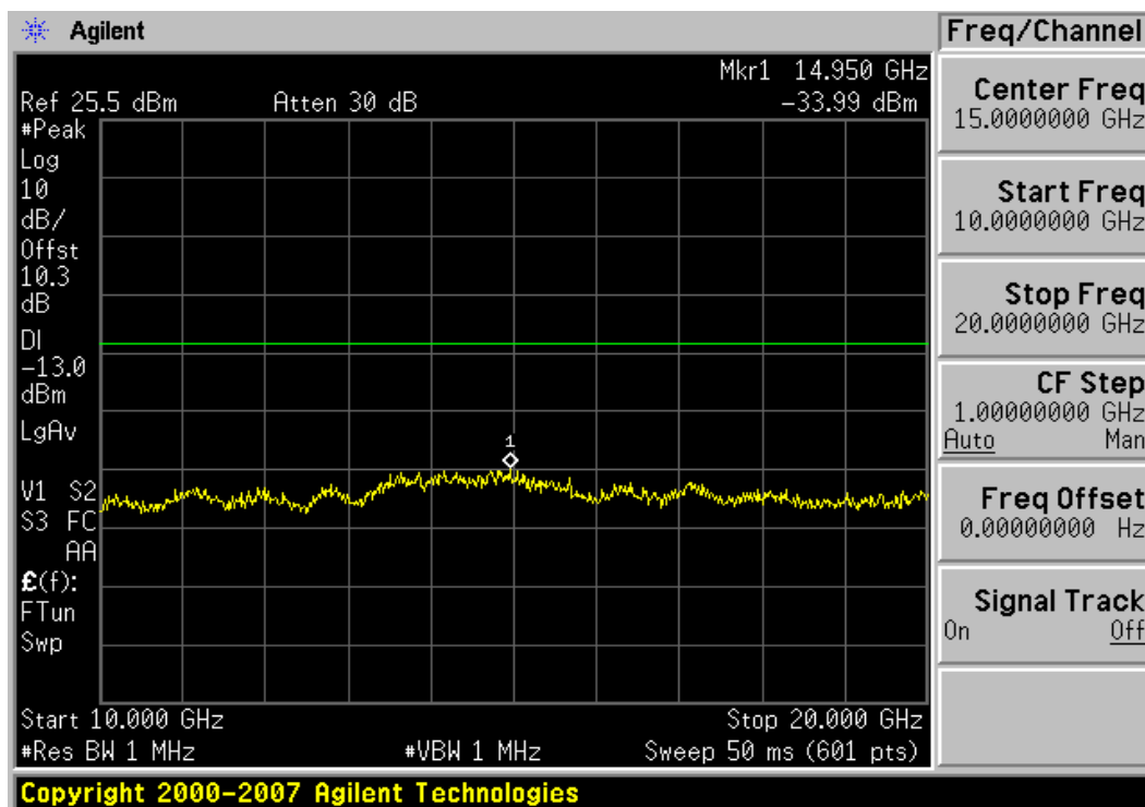
Plot 7-2. Conducted Spurious Plot (AWS CDMA Mode – Ch. 25)
