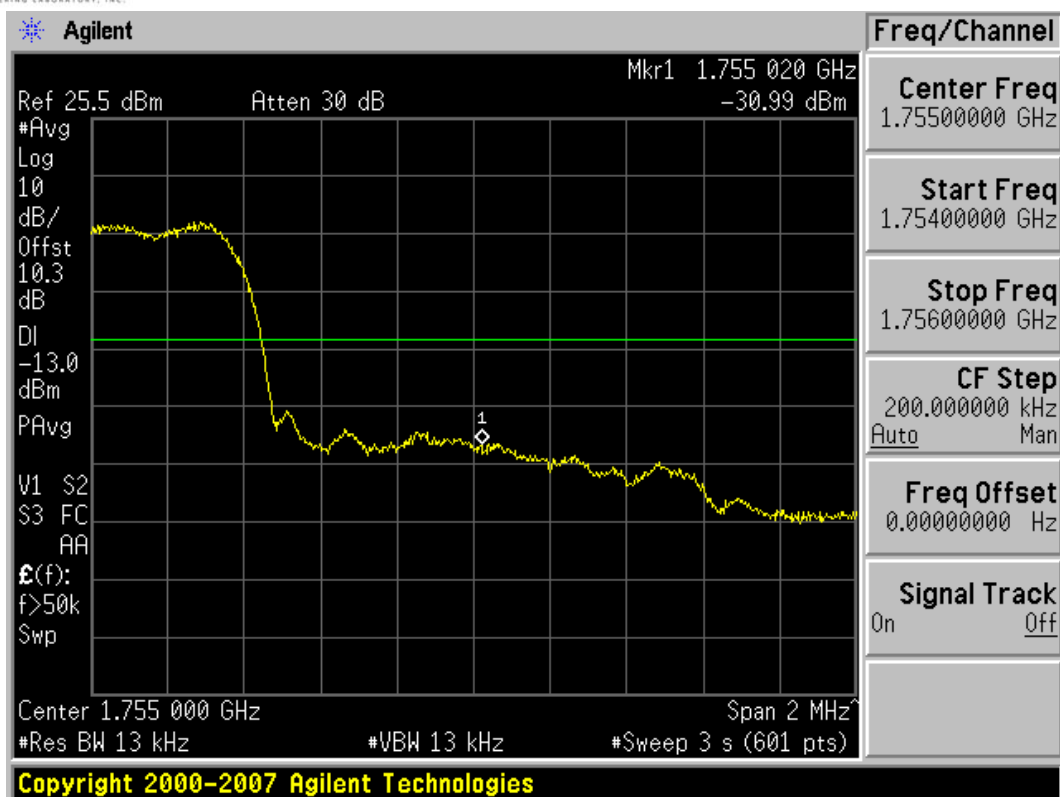
Plot 7-11. Band Edge Plot (AWS CDMA Mode – Ch. 875)
