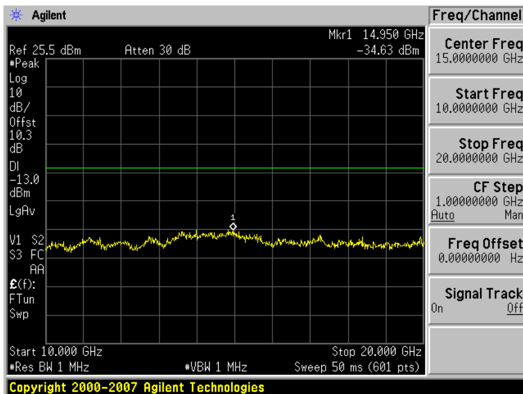
Plot 7-6. Conducted Spurious Plot (AWS CDMA Mode – Ch. 450)
