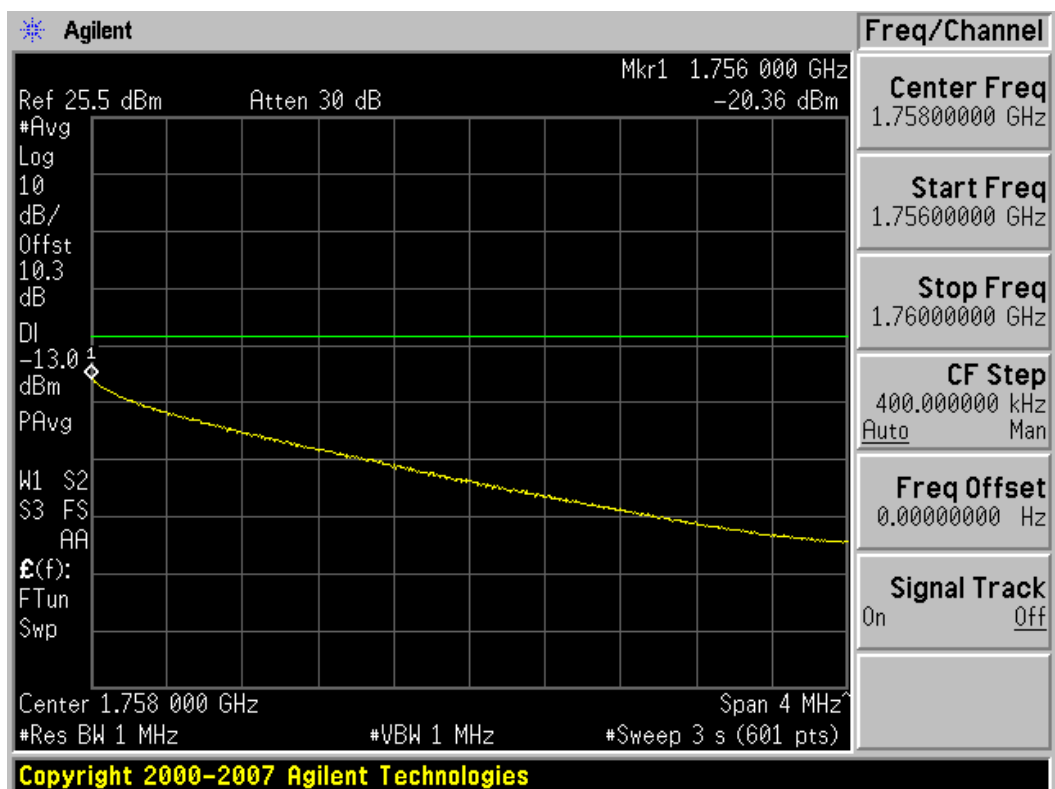
Plot 7-12. 4MHz Span Plot (AWS CDMA Mode – Ch. 875)
