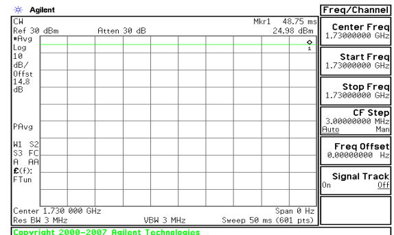
Figure 8-4 Zero-Span Plots
