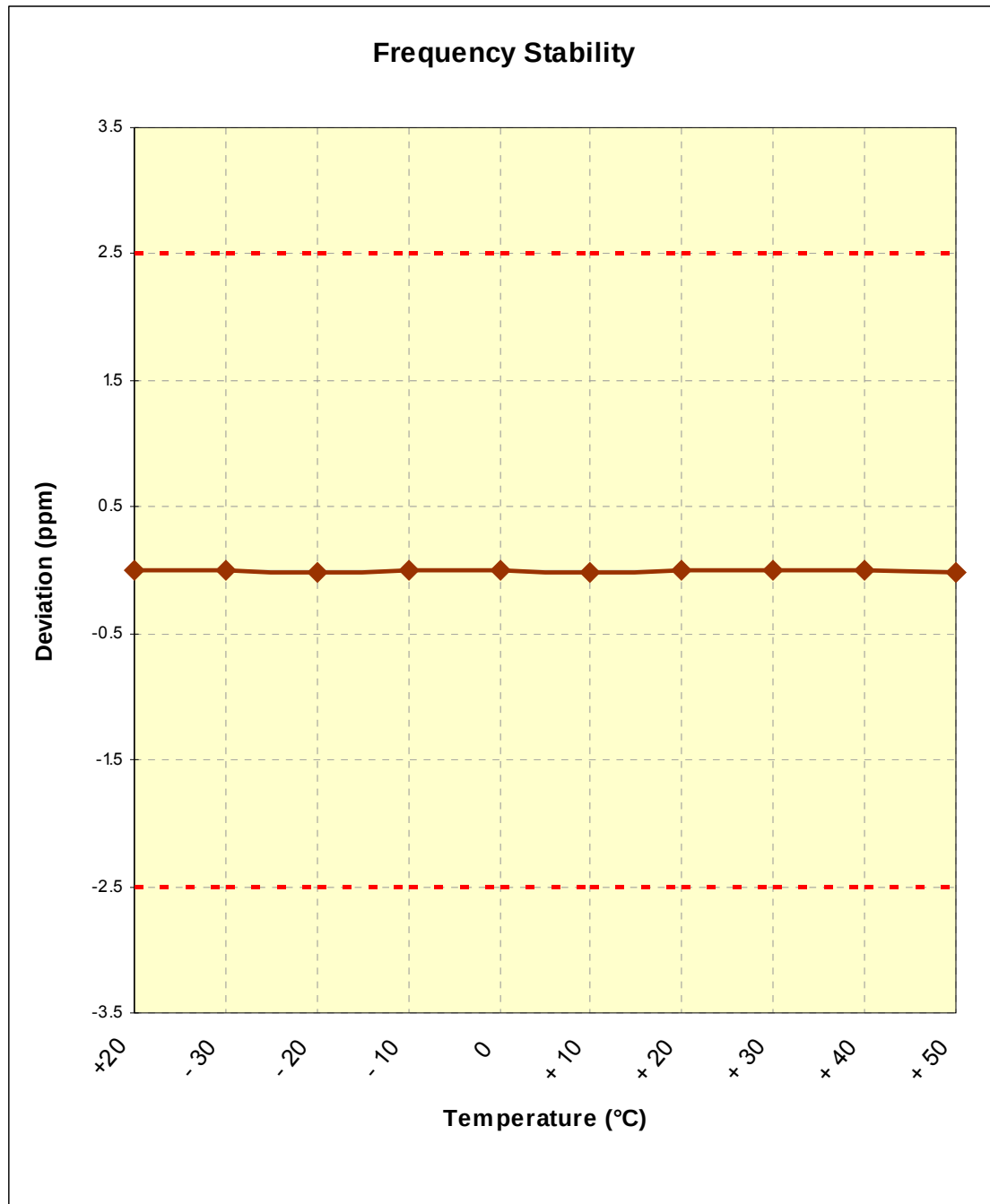
Figure 6-3. Frequency Stability Graph (PCS CDMA Mode – Ch. 600)
