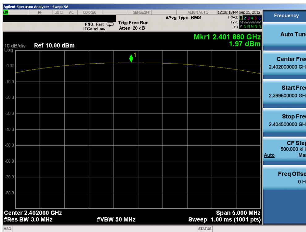
Plot 6-4. Conducted Power Plot (Bluetooth (LE) – Ch. 0)
