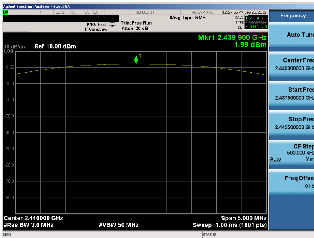
Plot 6-5. Conducted Power Plot (Bluetooth (LE) – Ch. 19)
