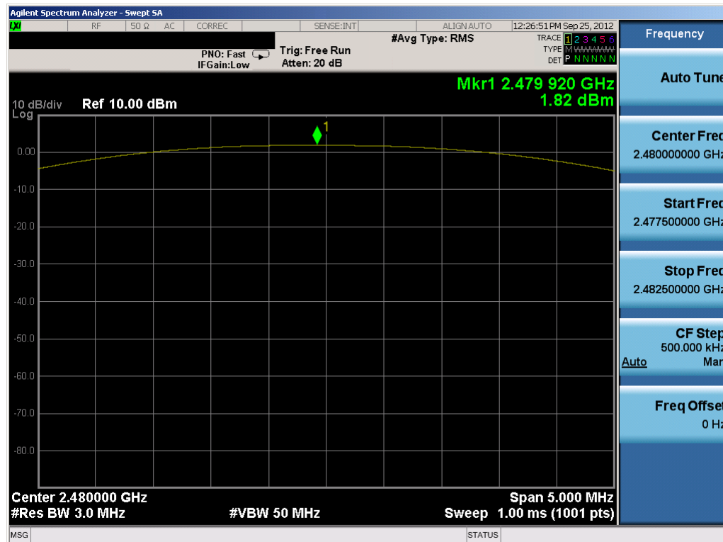
Plot 6-6. Conducted Power Plot (Bluetooth (LE) – Ch. 39)
