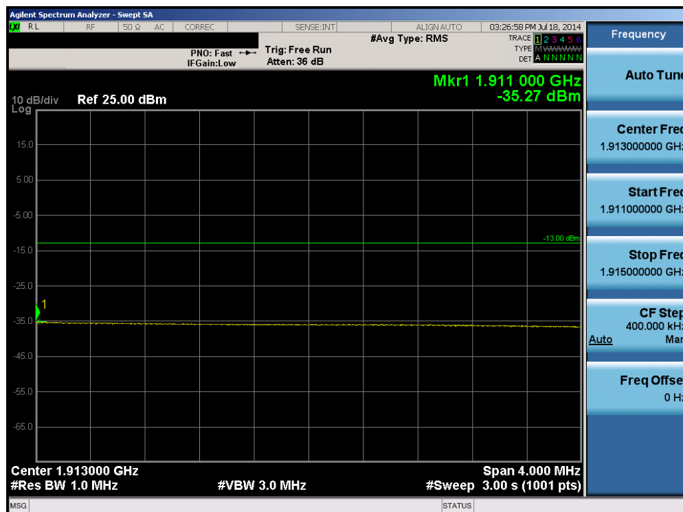
Plot 6-24. Upper Extended Band Edge Plot (Band 2 – 20.0MHz QPSK – RB Size 100)
