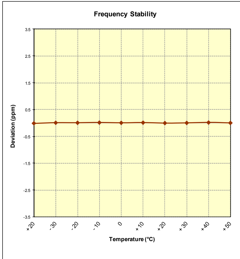
Figure 6-6. Frequency Stability Graph (Band 2)
