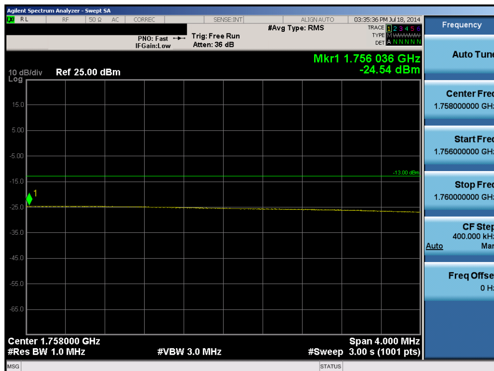
Plot 6-12. Upper Extended Band Edge Plot (Band 4 – 15.0MHz QPSK – RB Size 75)
