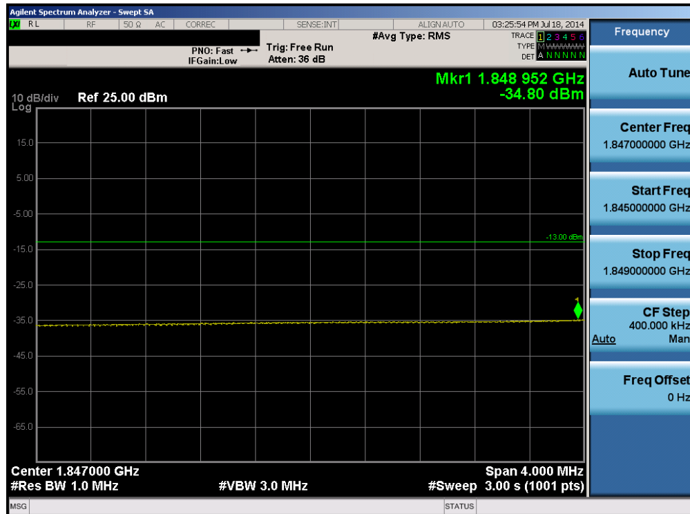
Plot 6-22. Lower Extended Band Edge Plot (Band 2 – 20.0MHz QPSK – RB Size 100)
