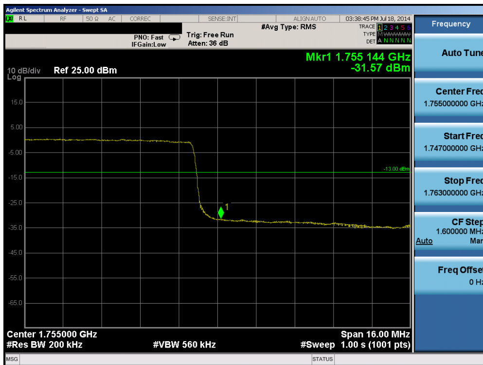
Plot 6-15. Upper Band Edge Plot (Band 4 – 20.0MHz QPSK – RB Size 100)
