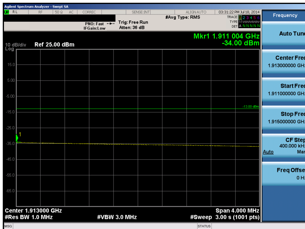
Plot 6-20. Upper Extended Band Edge Plot (Band 2 – 15.0MHz QPSK – RB Size 75)
