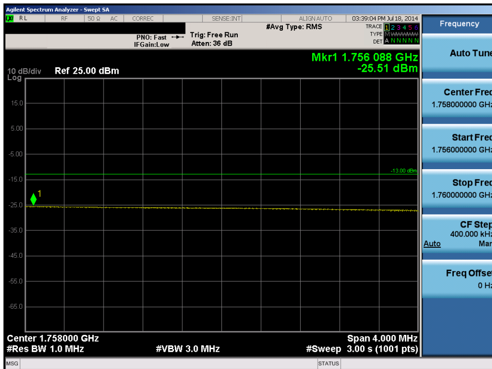
Plot 6-16. Upper Extended Band Edge Plot (Band 4 – 20.0MHz QPSK – RB Size 100)
