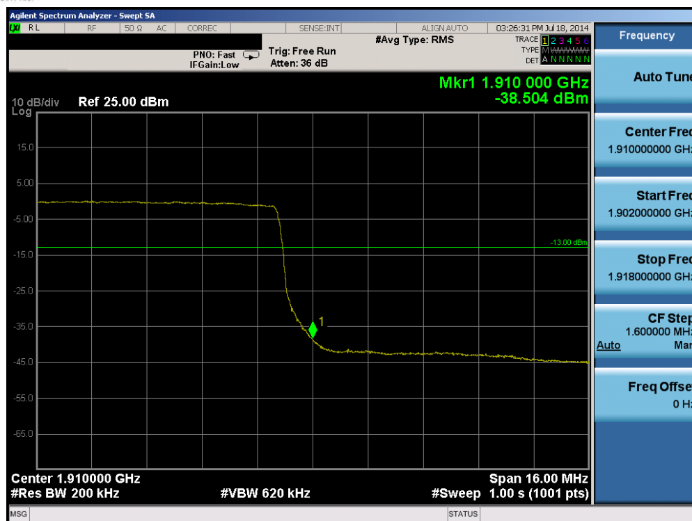
Plot 6-23. Upper Band Edge Plot (Band 2 – 20.0MHz QPSK – RB Size 100)
