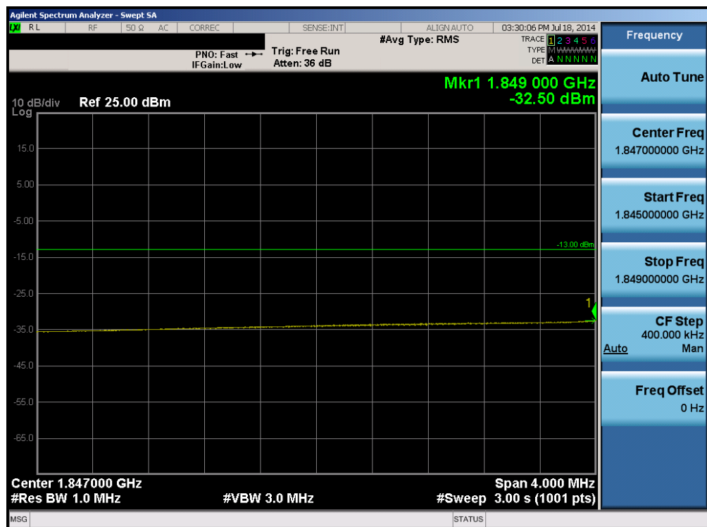
Plot 6-18. Lower Extended Band Edge Plot (Band 2 – 15.0MHz QPSK – RB Size 75)
