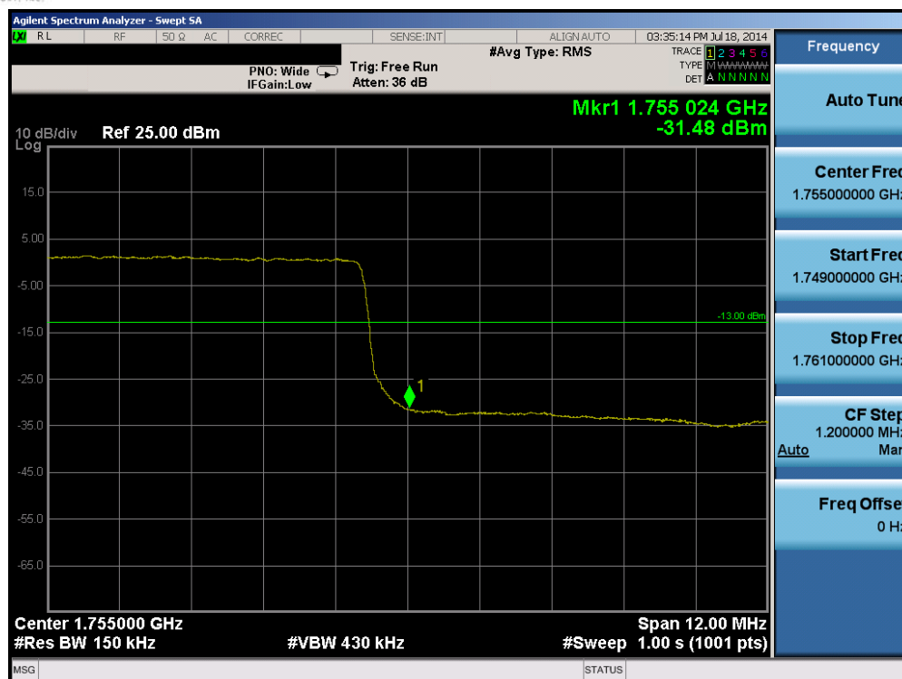
Plot 6-11. Upper Band Edge Plot (Band 4 – 15.0MHz QPSK – RB Size 75)
