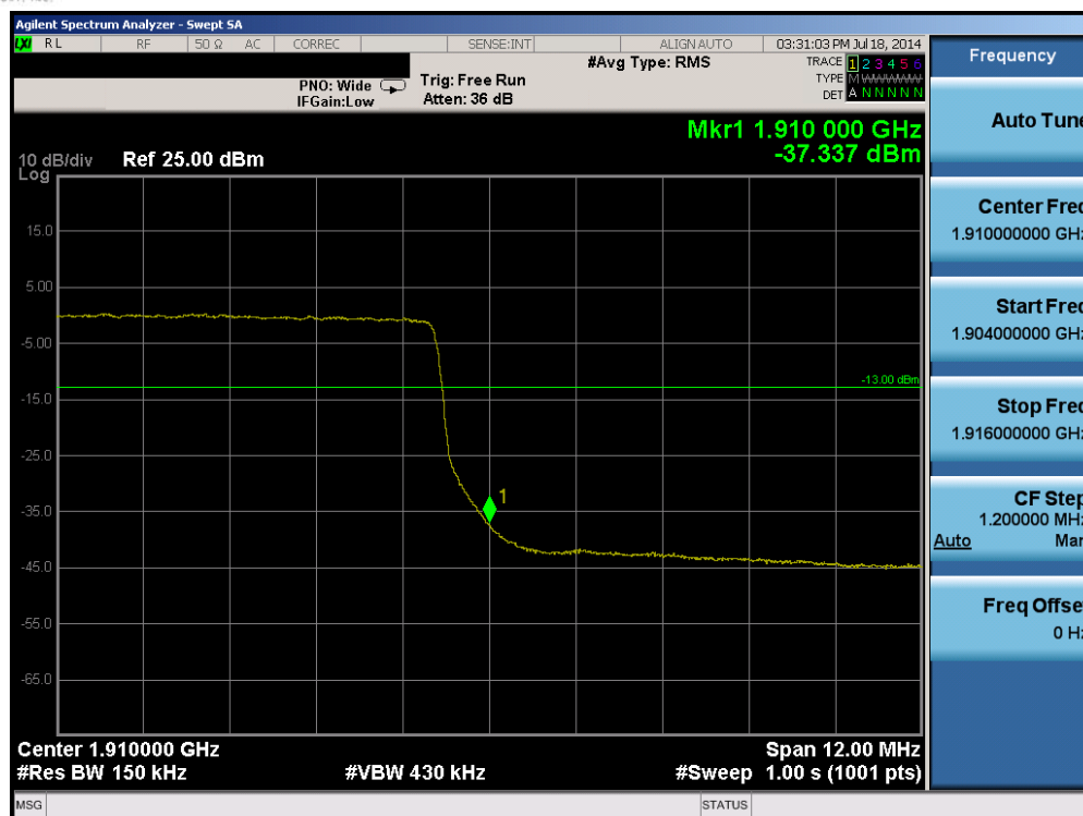
Plot 6-19. Upper Band Edge Plot (Band 2 – 15.0MHz QPSK – RB Size 75)
