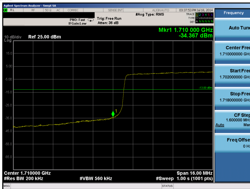
Plot 6-13. Lower Band Edge Plot (Band 4 – 20.0MHz QPSK – RB Size 100)
