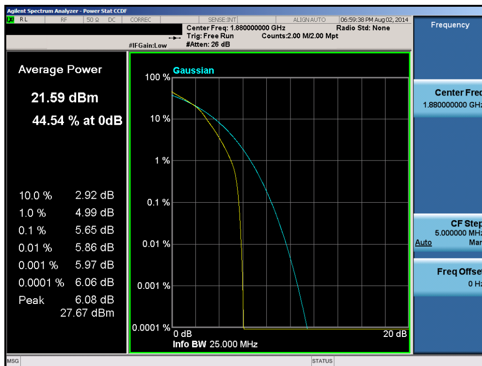
Plot 6-26. PAR Plot (Band 2 – 15.0MHz 16-QAM – RB Size 75)
