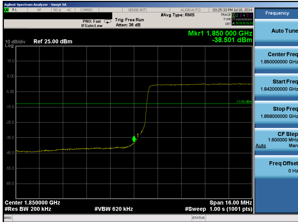
Plot 6-21. Lower Band Edge Plot (Band 2 – 20.0MHz QPSK – RB Size 100)
