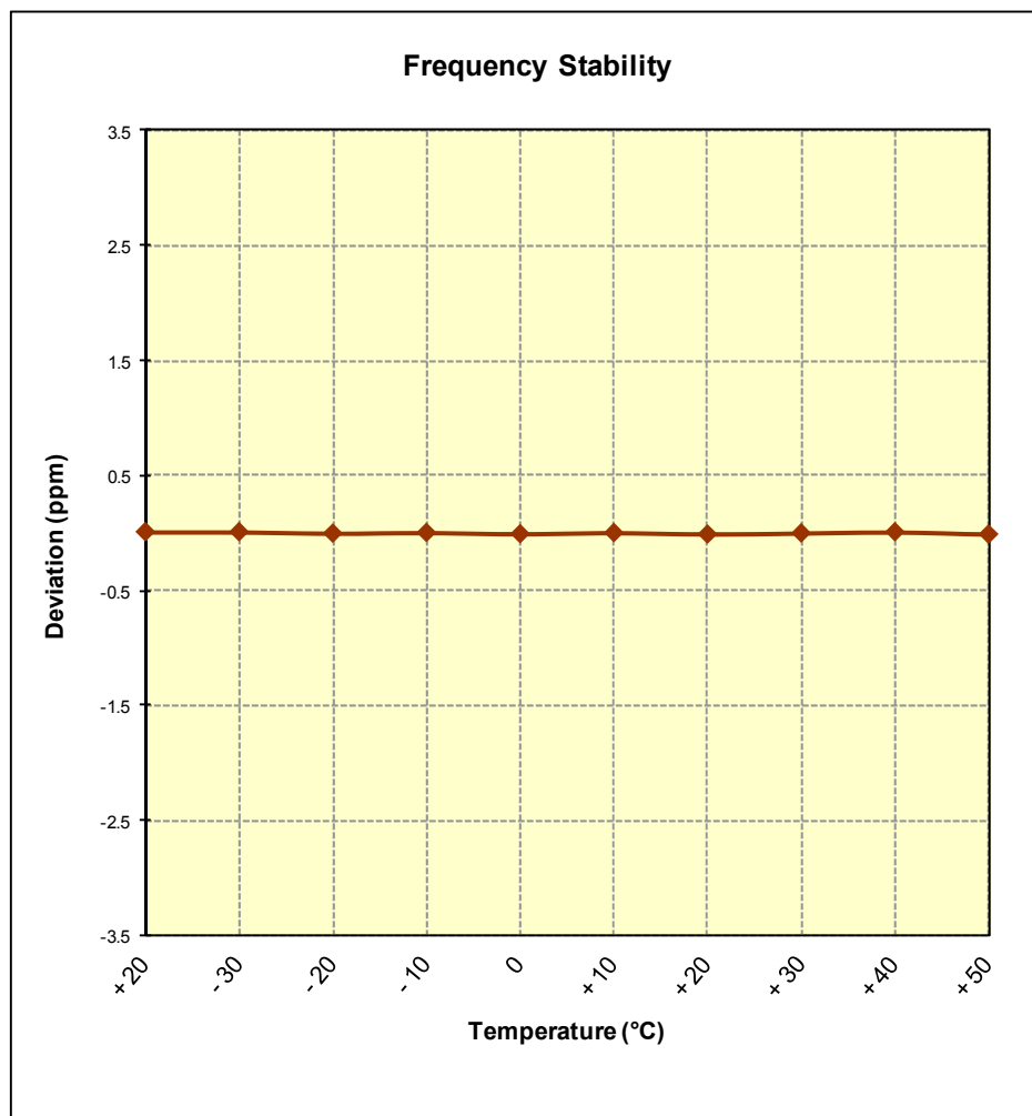
Figure 6-5. Frequency Stability Graph (Band 4)
