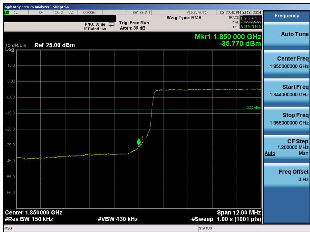
Plot 6-17. Lower Band Edge Plot (Band 2 – 15.0MHz QPSK – RB Size 75)
