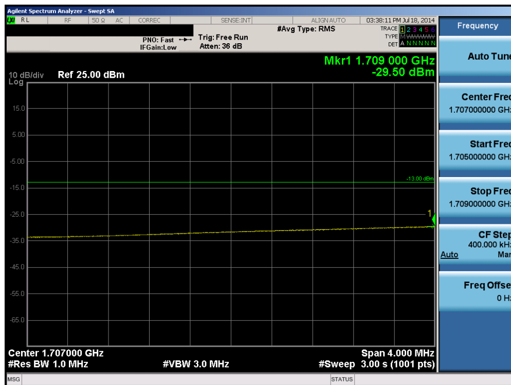
Plot 6-14. Lower Extended Band Edge Plot (Band 4 – 20.0MHz QPSK – RB Size 100)
