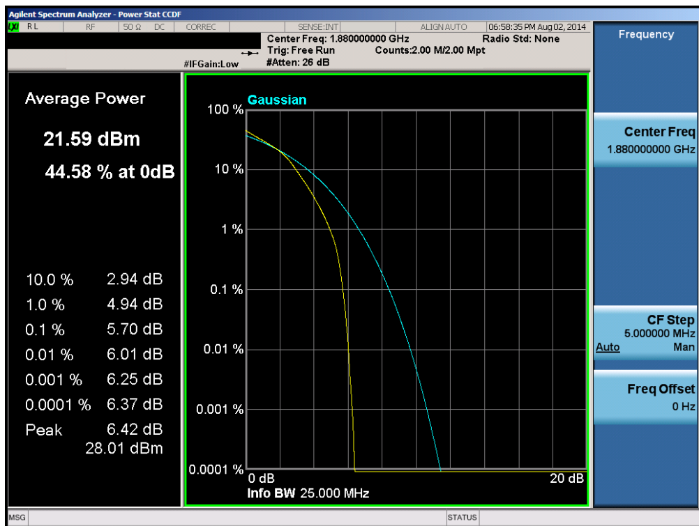
Plot 6-28. PAR Plot (Band 2 – 20.0MHz 16-QAM – RB Size 100)
