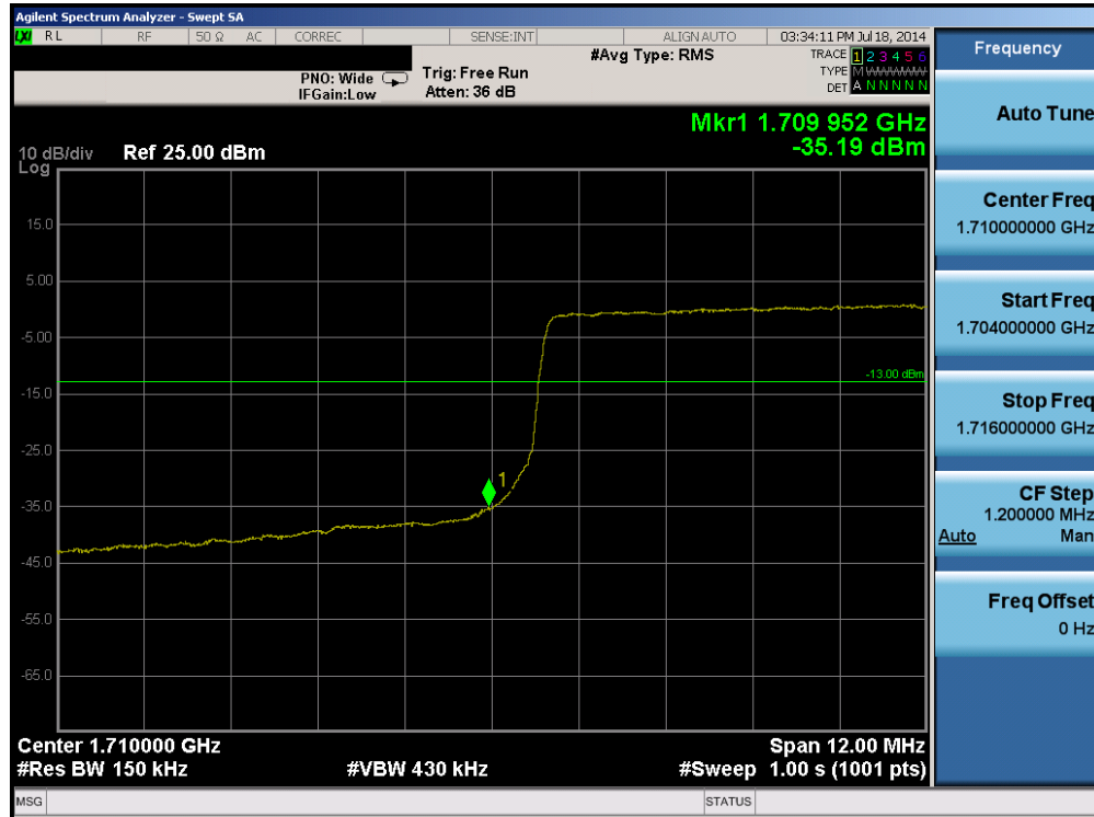
Plot 6-9. Lower Band Edge Plot (Band 4 – 15.0MHz QPSK – RB Size 75)
