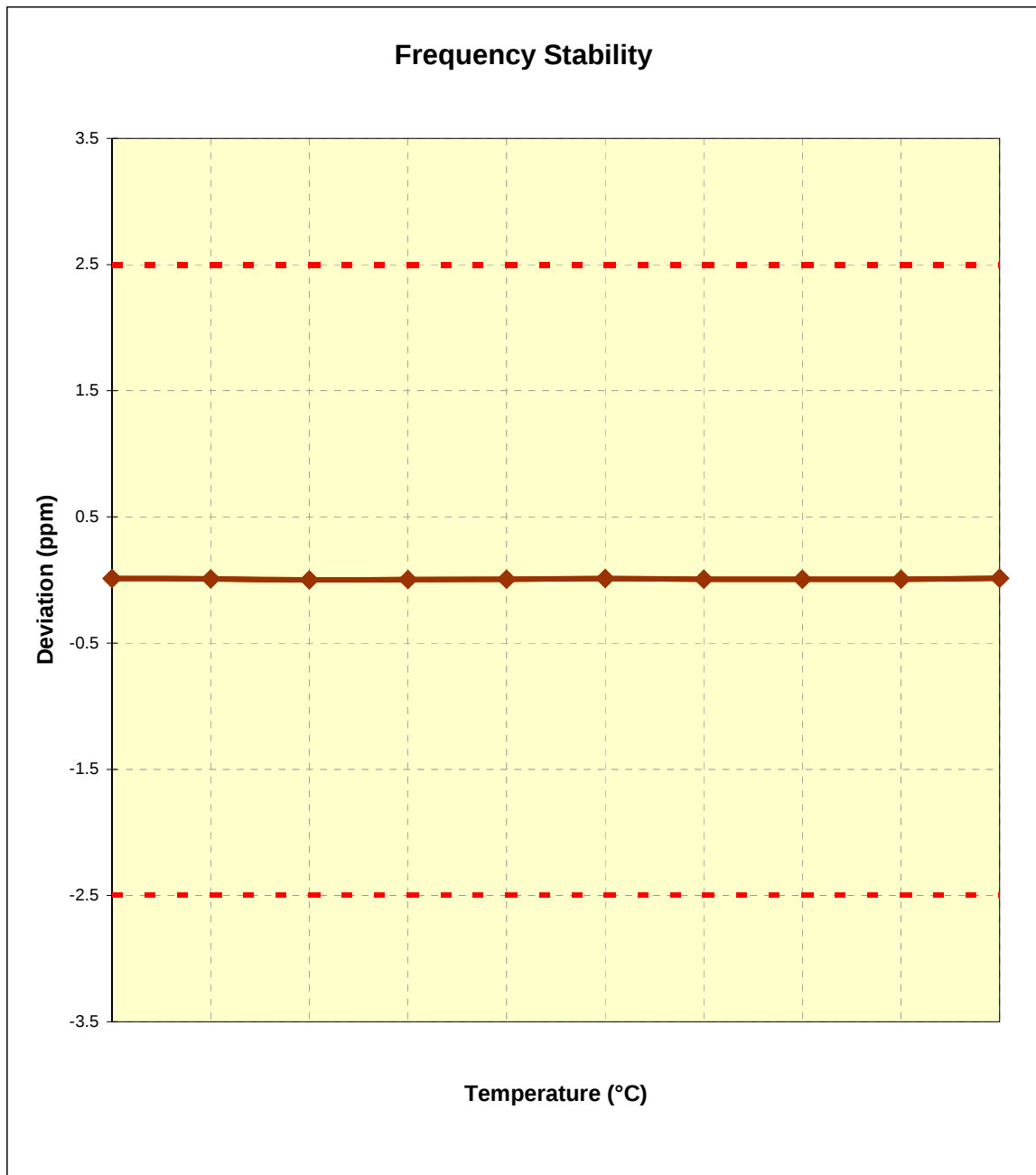
Figure 6-3. Frequency Stability Graph (PCS CDMA Mode – Ch. 600)
