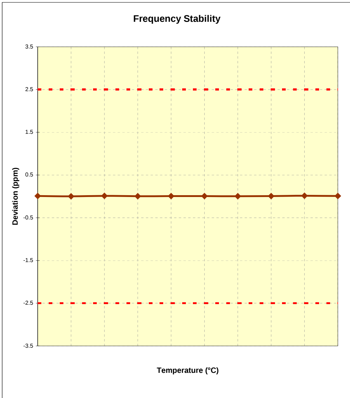
Figure 6-2. Frequency Stability Graph (AWS CDMA Mode – Ch. 450)
