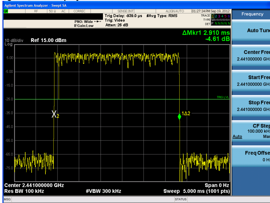
Plot 6-24. Time of Occupancy Plot (Bluetooth)
