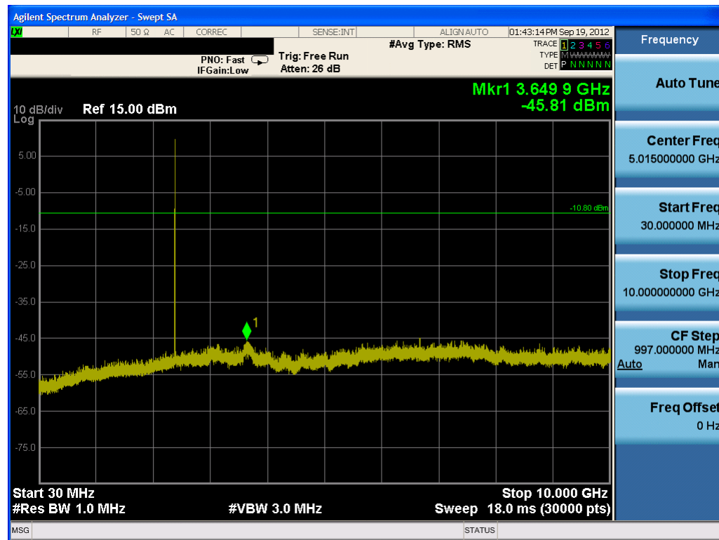
Plot 6-27. Conducted Spurious Plot (Bluetooth, 3Mbps – Ch. 0)
