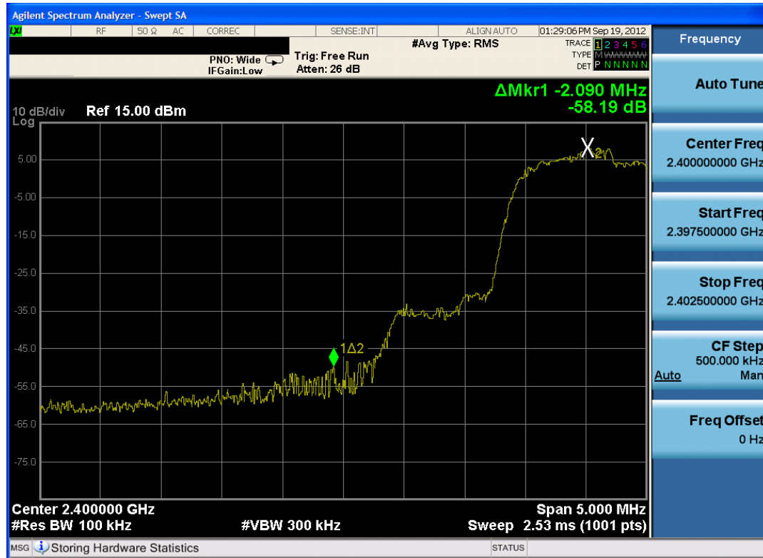
Plot 6-19. Band Edge Plot (Bluetooth with Hopping Disabled, 3Mbps – Ch. 0)
