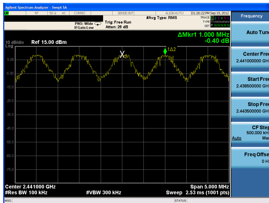
Plot 6-23. Channel Spacing Plot (Bluetooth)
