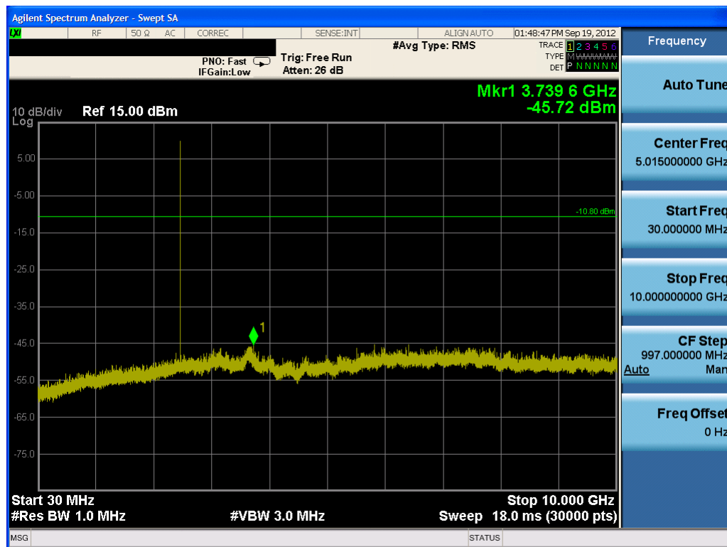
Plot 6-31. Conducted Spurious Plot (Bluetooth, 3Mbps – Ch. 78)
