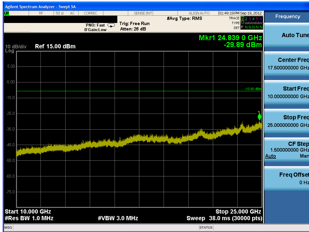
Plot 6-32. Conducted Spurious Plot (Bluetooth, 3Mbps – Ch. 78)
