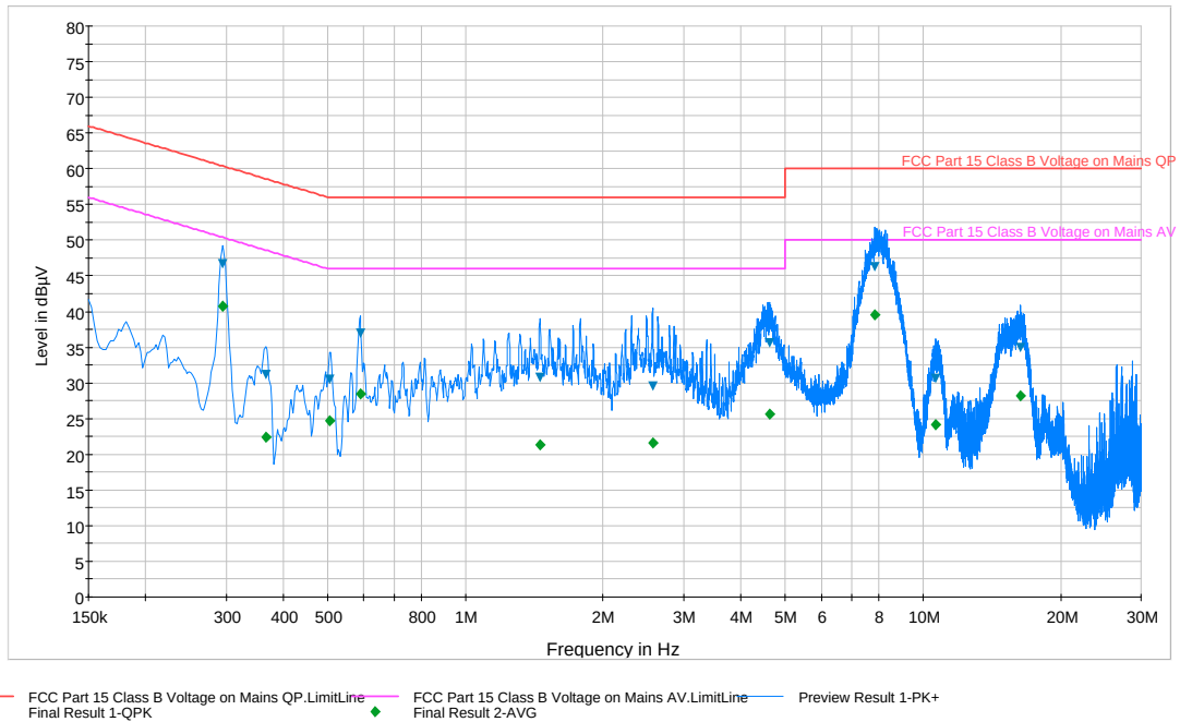
Plot 6-33. Line-Conducted Test Plot (L1)
