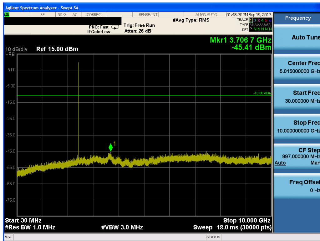
Plot 6-29. Conducted Spurious Plot (Bluetooth, 3Mbps – Ch. 39)
