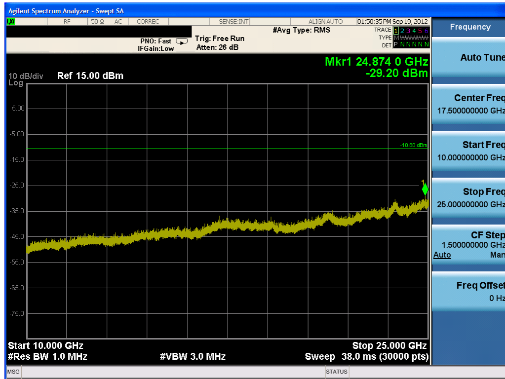
Plot 6-28. Conducted Spurious Plot (Bluetooth, 3Mbps – Ch. 0)
