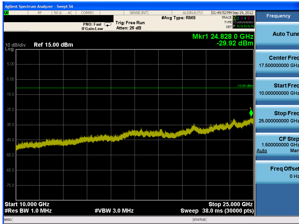
Plot 6-30. Conducted Spurious Plot (Bluetooth, 3Mbps – Ch. 39)
