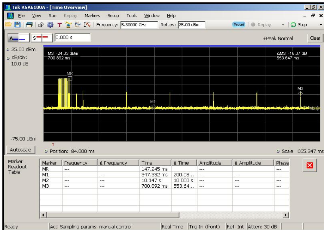
Figure 5-5. Aggregate Time using Pulse Table Capability
