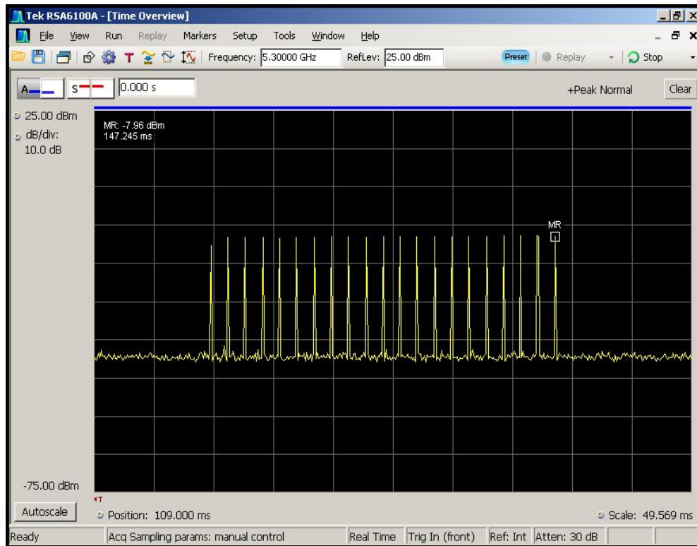
Figure 5-1. Type 1 Radar Pulse
