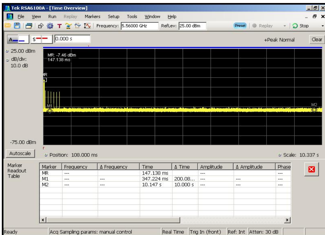
Figure 6-4. Channel Move Time (< 10sec)
