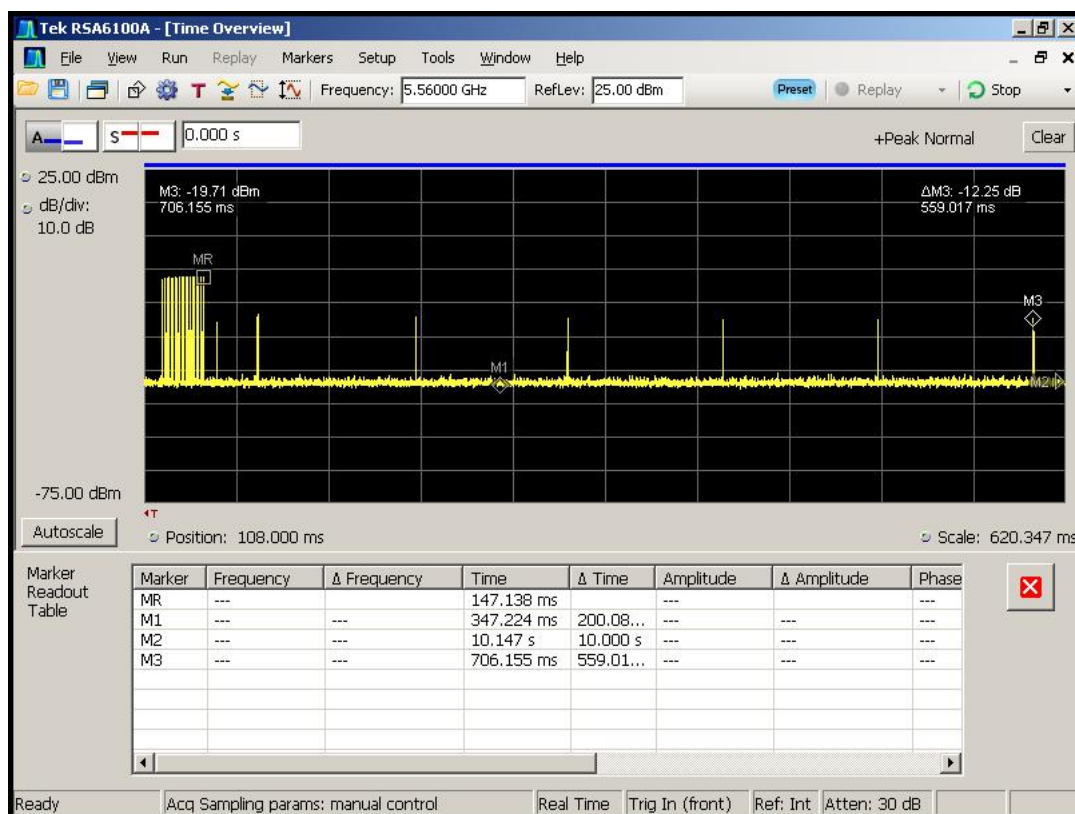
Figure 6-5. Aggregate Time using Pulse Table Capability
