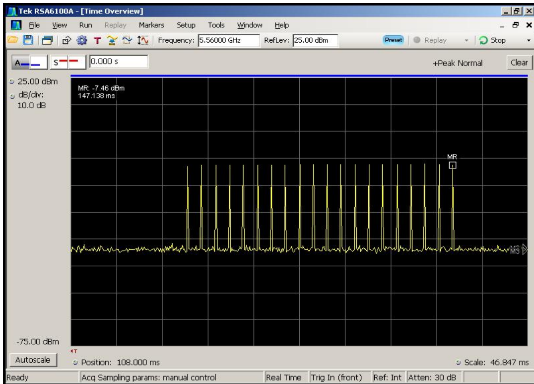
Figure 6-1. Type 1 Radar Pulse
