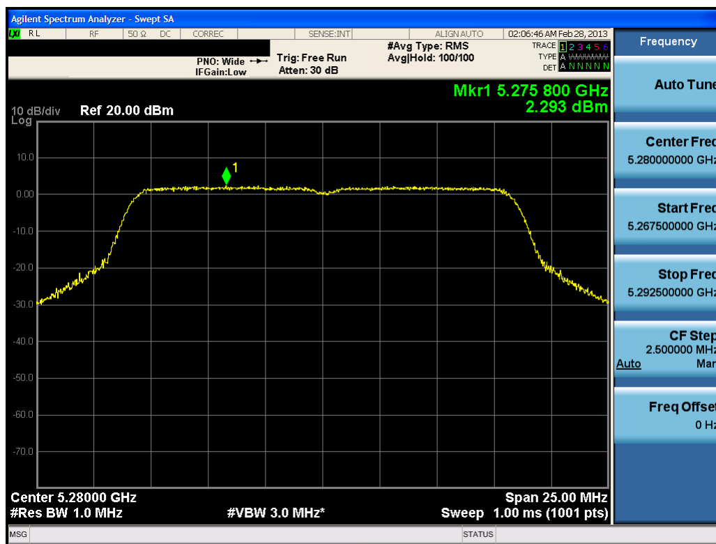
Plot 6-35. Peak Power Spectral Density Plot (802.11a (UNII Band 2) – Ch. 56)
