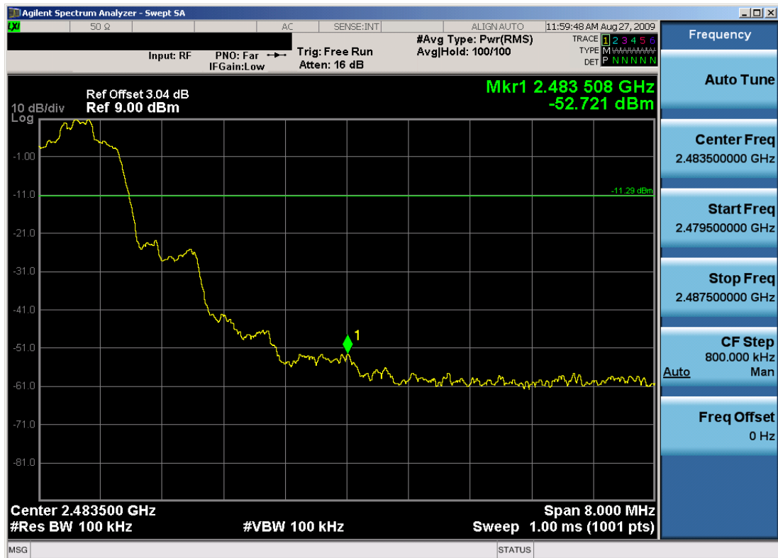
Plot 6-7. Band Edge Plot (Bluetooth 2.0 with Enhanced Data Rates – Ch. 78)
