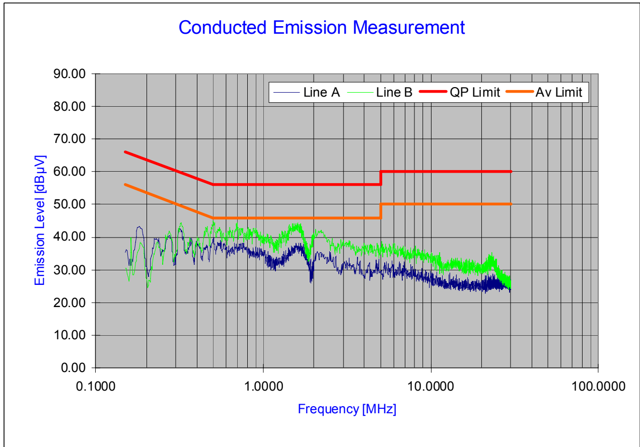
Plot 6-18. Line Conducted Plot with Bluetooth
