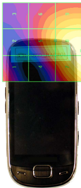
Figure 17-4 E-Field WD Scan overlay
