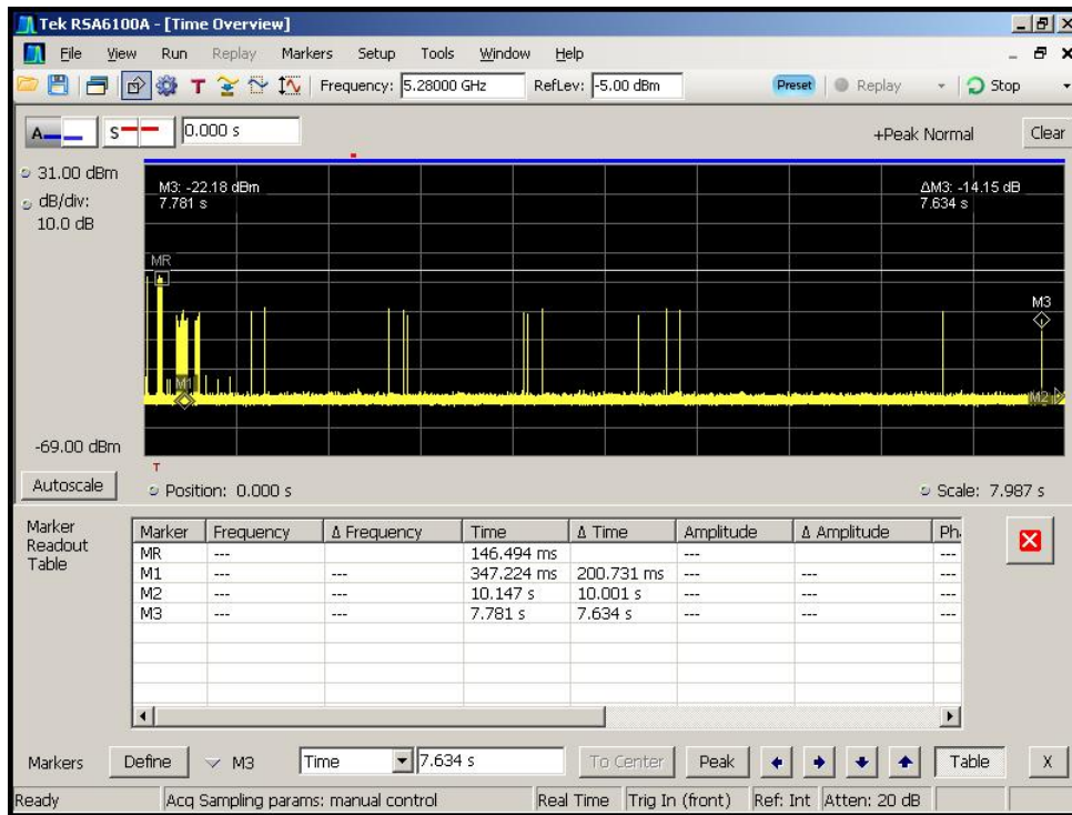
Figure 5-5. Channel Move Time (Zoomed In)
