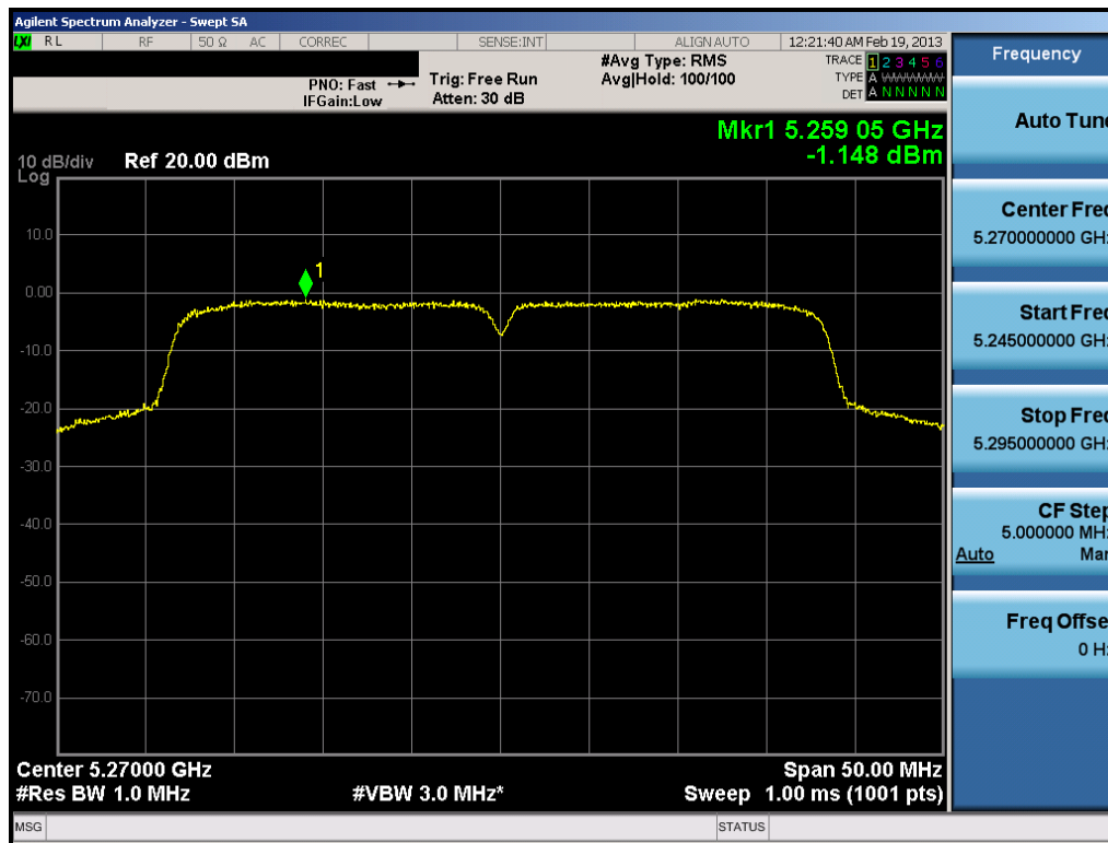
Plot 6-40. Peak Power Spectral Density Plot (40MHz BW 802.11n (UNII Band 2) – Ch. 54)
