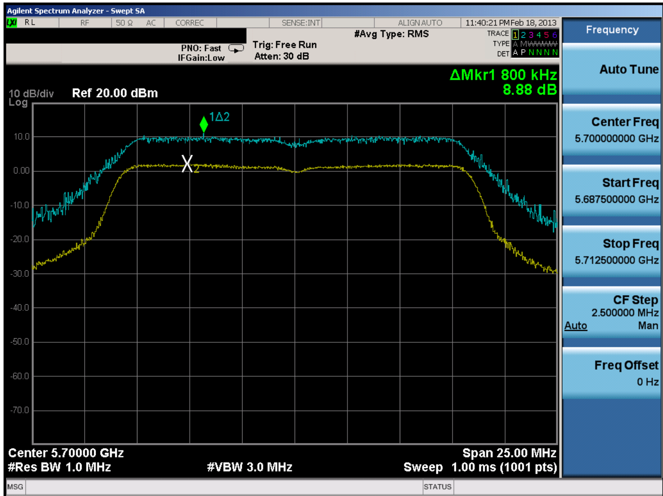
Plot 6-51. Peak Excursion Ratio Plot (802.11a)
