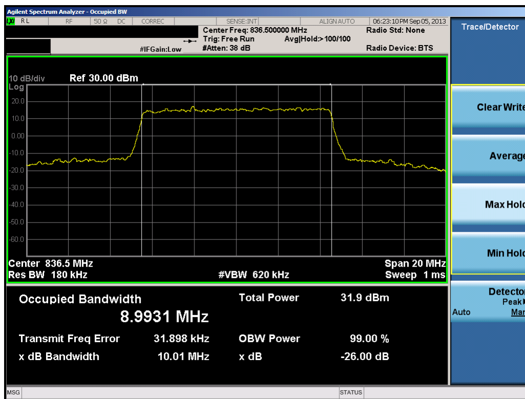
Plot 8-12. Occupied Bandwidth Plot (10.0MHz QPSK – RB Size 50)
