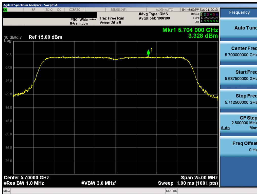
Plot 6-49. Peak Power Spectral Density Plot (20MHz BW 802.11a/n (UNII Band 3) – Ch. 140)
