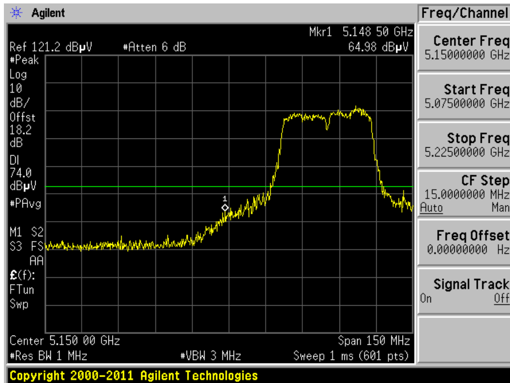
Plot 6-57. Radiated Restricted Lower Band Edge Plot (Peak – UNII Band 1)
