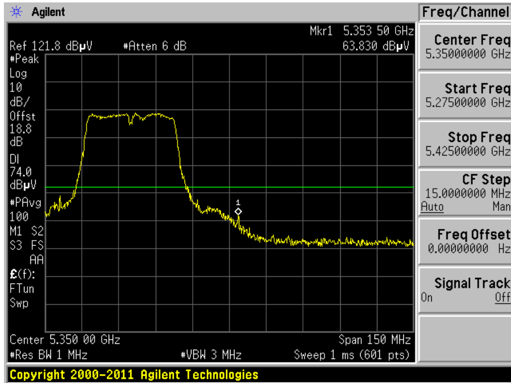
Plot 6-59. Radiated Restricted Upper Band Edge Plot (Peak – UNII Band 2)
