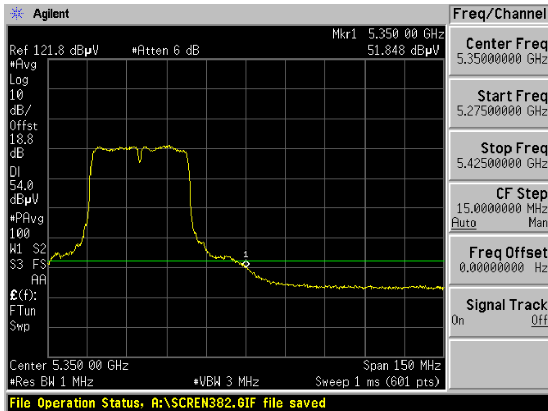
Plot 6-58. Radiated Restricted Upper Band Edge Plot (Average – UNII Band 2)
