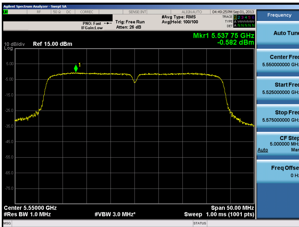
Plot 6-51. Peak Power Spectral Density Plot (40MHz BW 802.11a/n (UNII Band 3) – Ch. 110)
