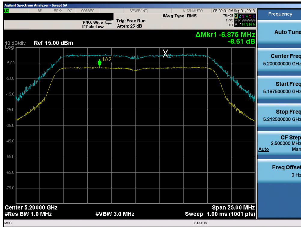
Plot 6-53. Peak Excursion Ratio Plot (802.11a)
