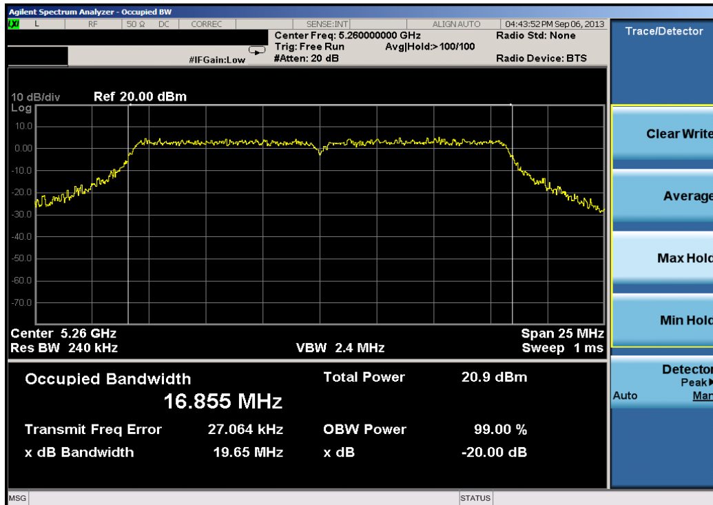
Plot 6-26. 20dB Bandwidth Plot (20MHz BW 802.11n (UNII Band 2) – Ch. 52)
