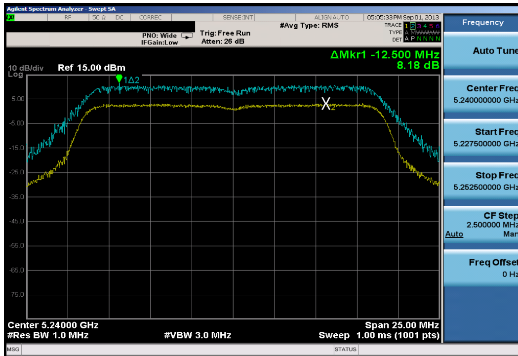
Plot 6-54. Peak Excursion Ratio Plot (20MHz BW 802.11n)
