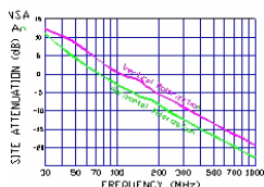
Figure 3-8. Normalized Site Attenuation Curves (H&V)
