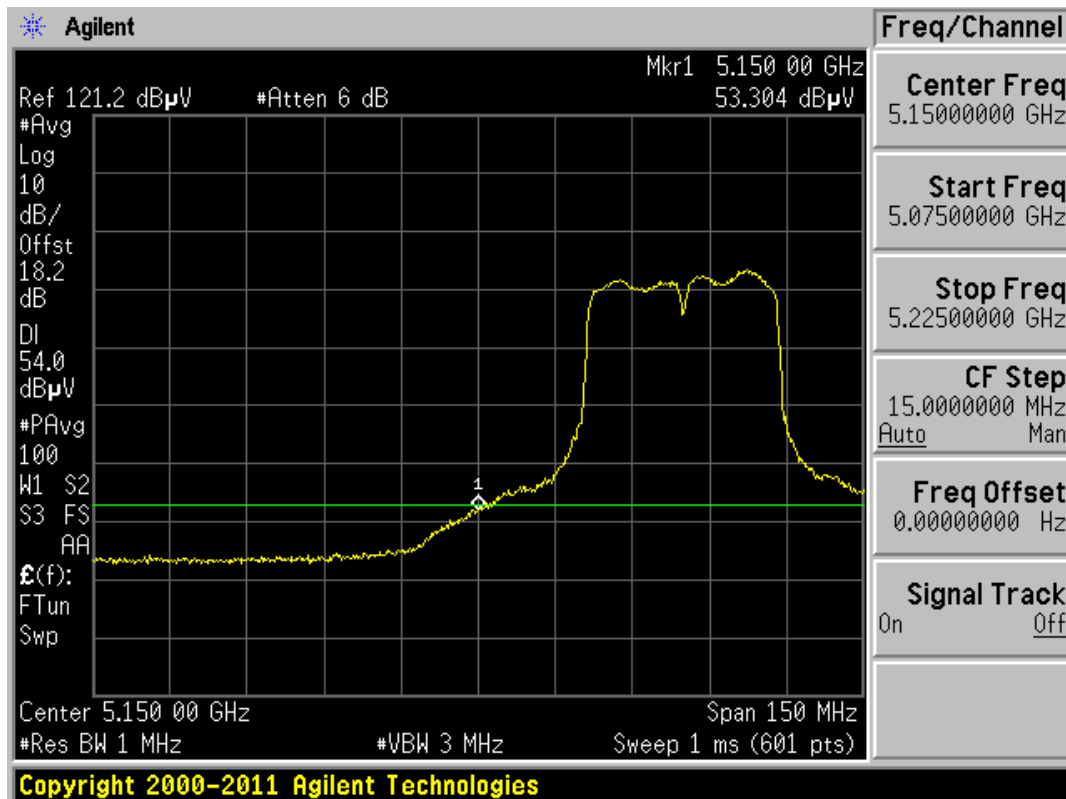
Plot 6-56. Radiated Restricted Lower Band Edge Plot (Average – UNII Band 1)
