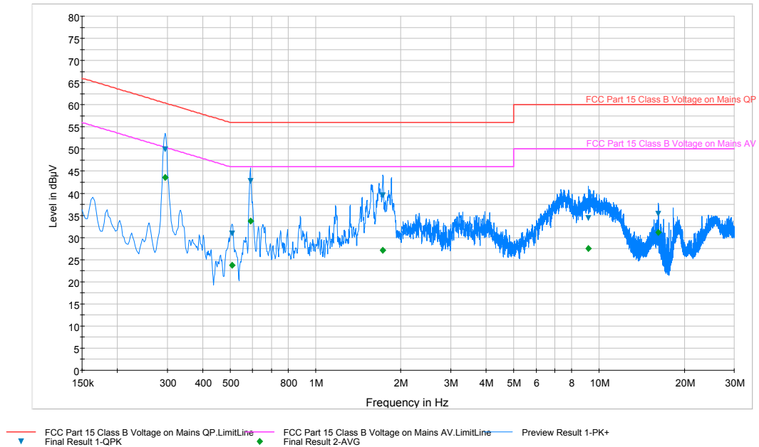
Plot 6-61. Line Conducted Plot with 802.11b (L1)
