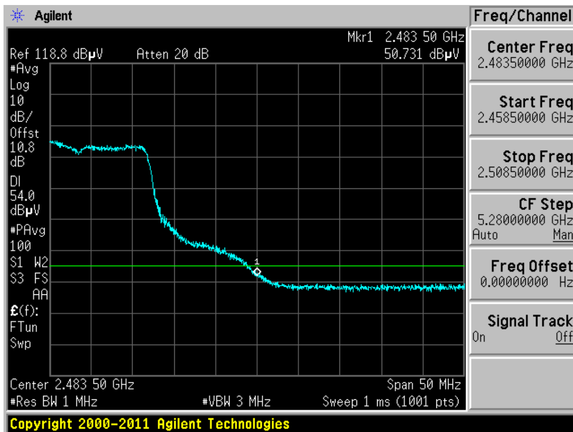
Plot 6-59. Radiated Restricted Upper Band Edge Measurement (Average)
