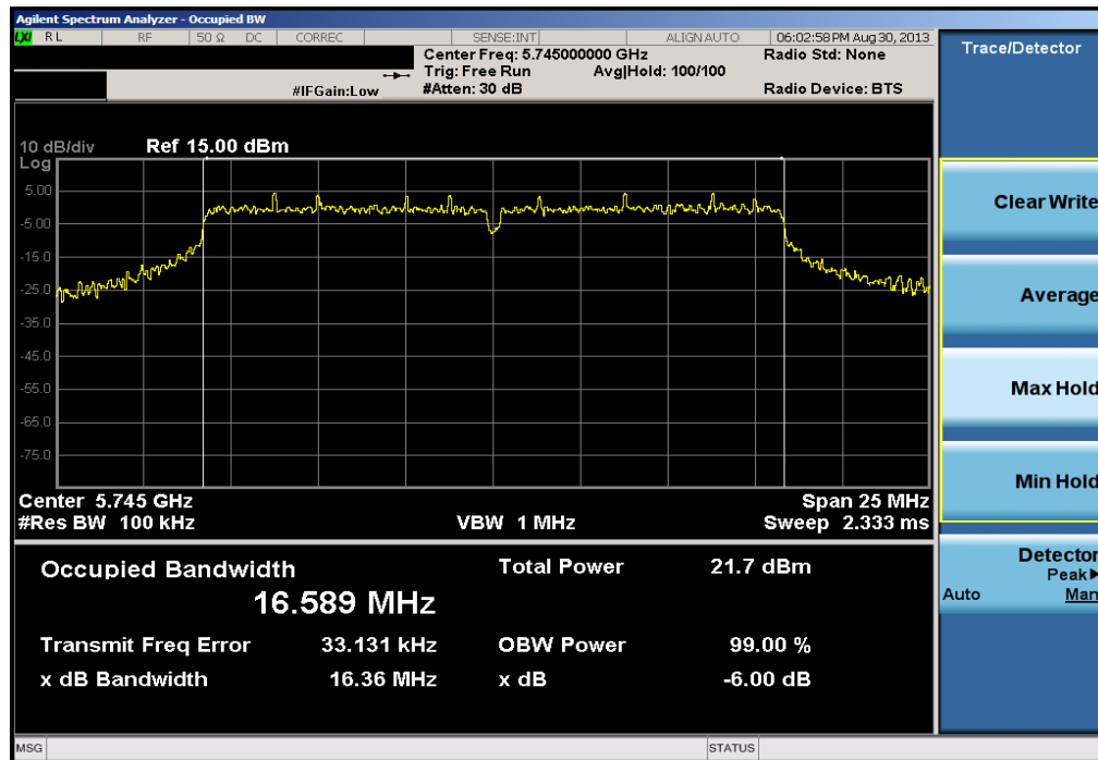
Plot 6-10. 6dB Bandwidth Plot (802.11a – Ch. 149)
