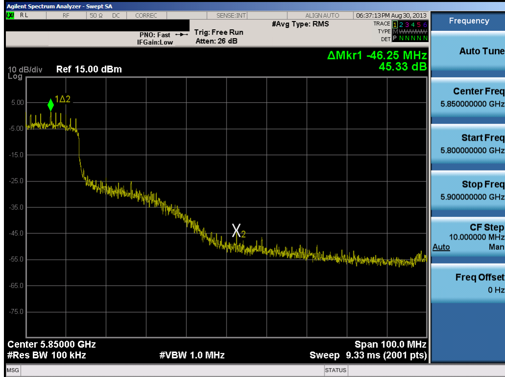
Plot 6-46. Band Edge Plot (40MHz BW 802.11a/b/g/n (5.8GHz) – Ch. 159)
