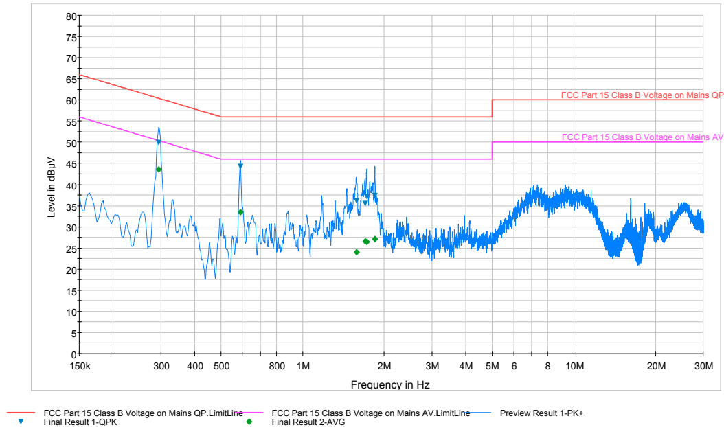
Plot 6-62. Line Conducted Plot with 802.11b (N)
