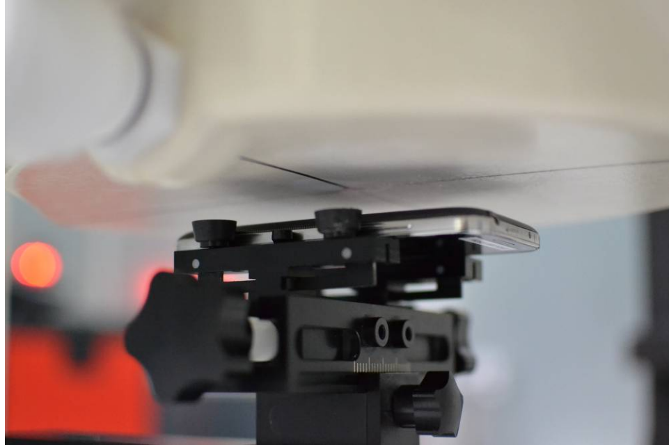
SAR Test Setup Photo 11 – Back Side at 1.5 cm
