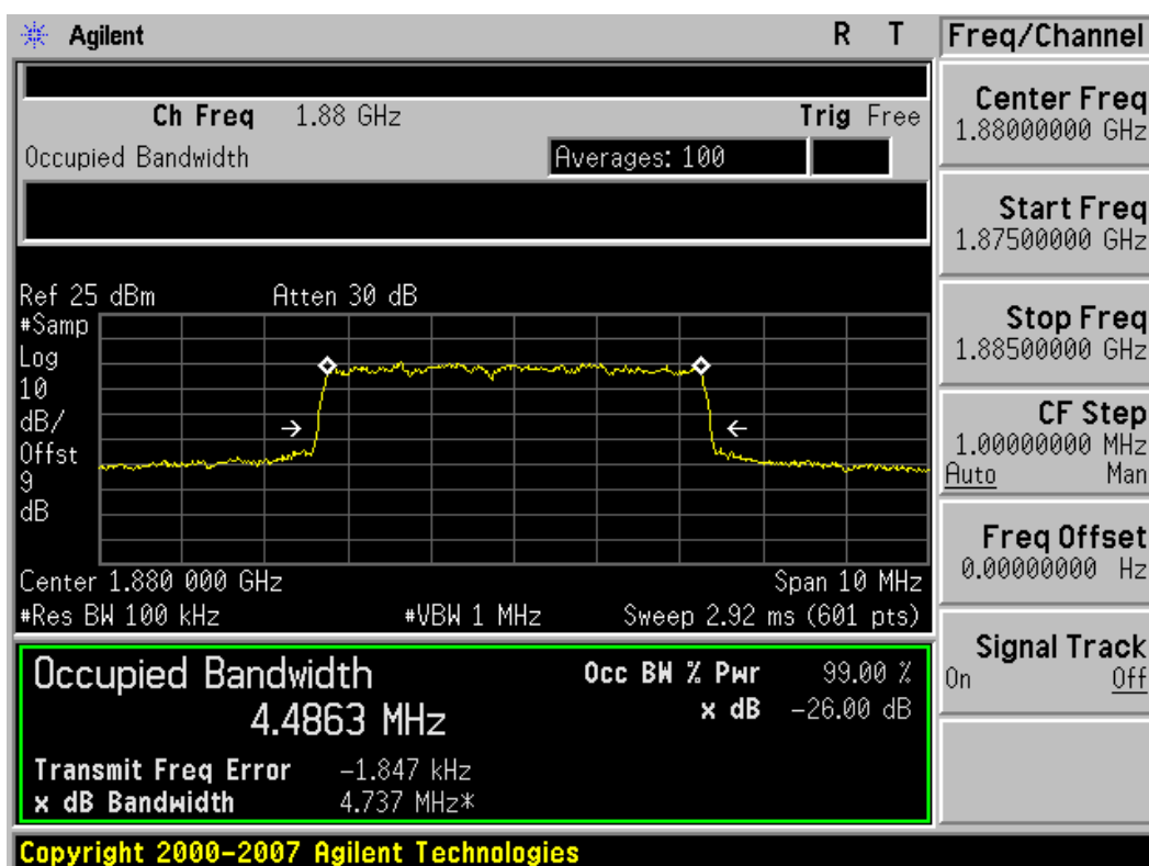
Plot 8-32. Occupied Bandwidth Plot (5MHz BW, 16-QAM, PCS Band – Mid Channel)
