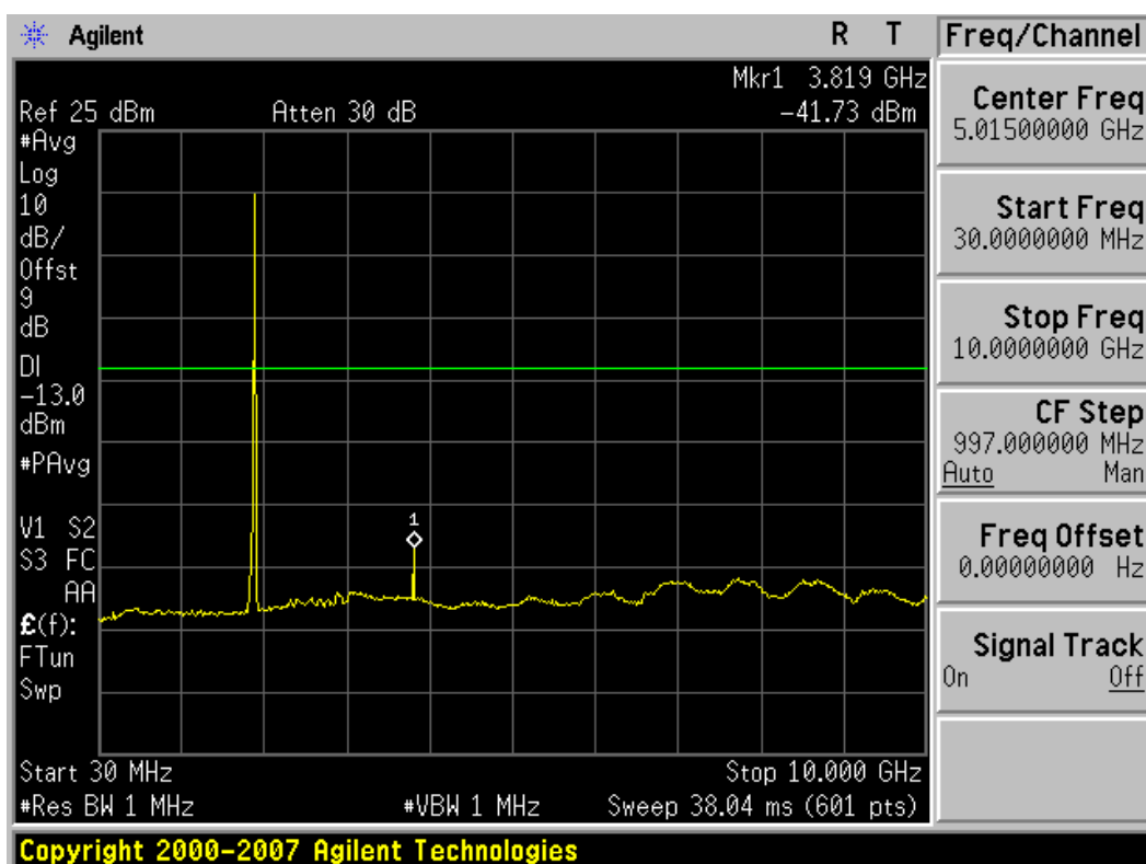
Plot 8-22. Conducted Spurious Plot (3MHz BW, QPSK, PCS Band – High Channel)
