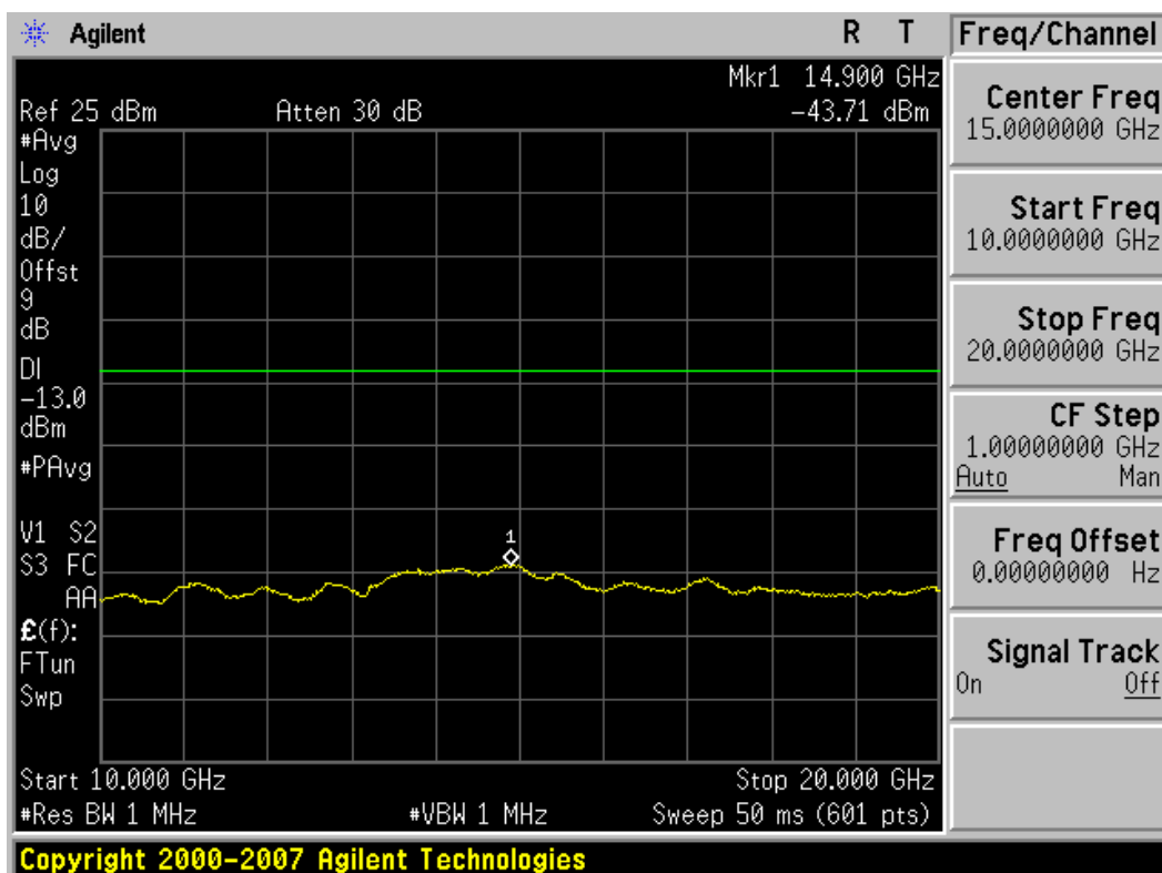
Plot 8-14. Conducted Spurious Plot (3MHz BW, QPSK, PCS Band – Low Channel)
