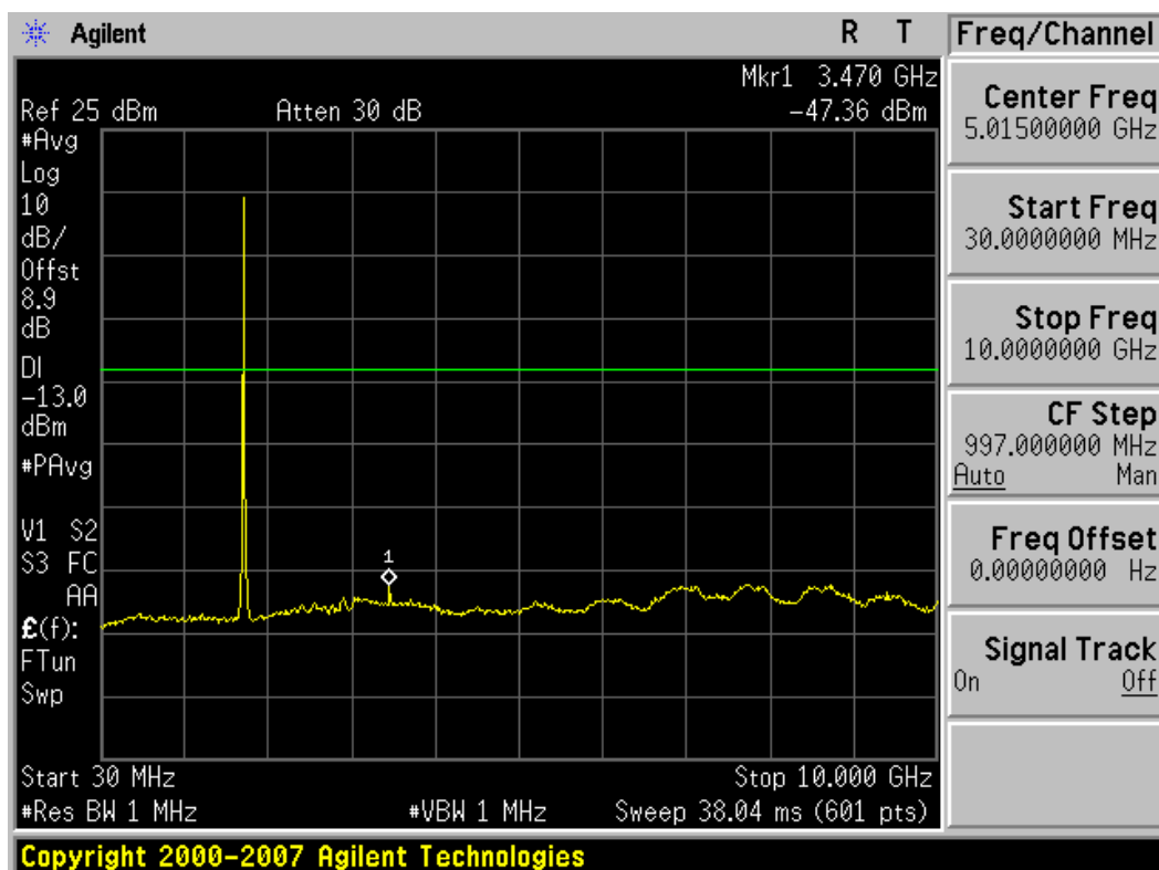
Plot 7-16. Conducted Spurious Plot (3MHz BW, QPSK, AWS Band – Mid Channel)
