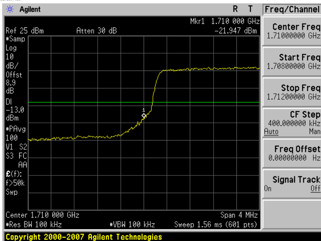
Plot 7-27. Band Edge Plot (5MHz BW, QPSK, AWS Band – Low Channel)
