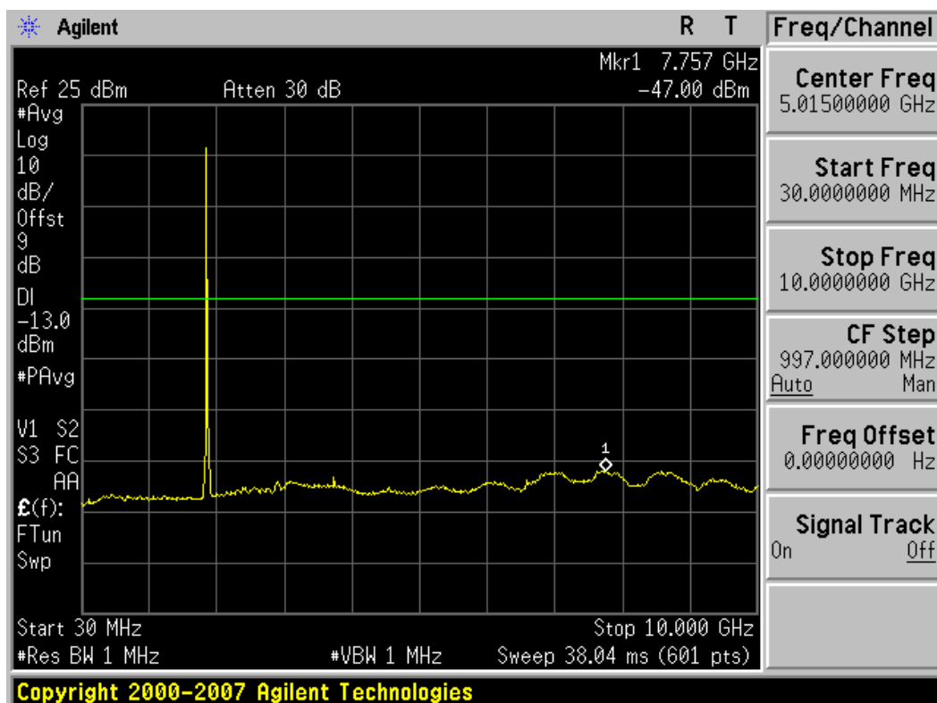
Plot 8-16. Conducted Spurious Plot (3MHz BW, QPSK, PCS Band – Mid Channel)
