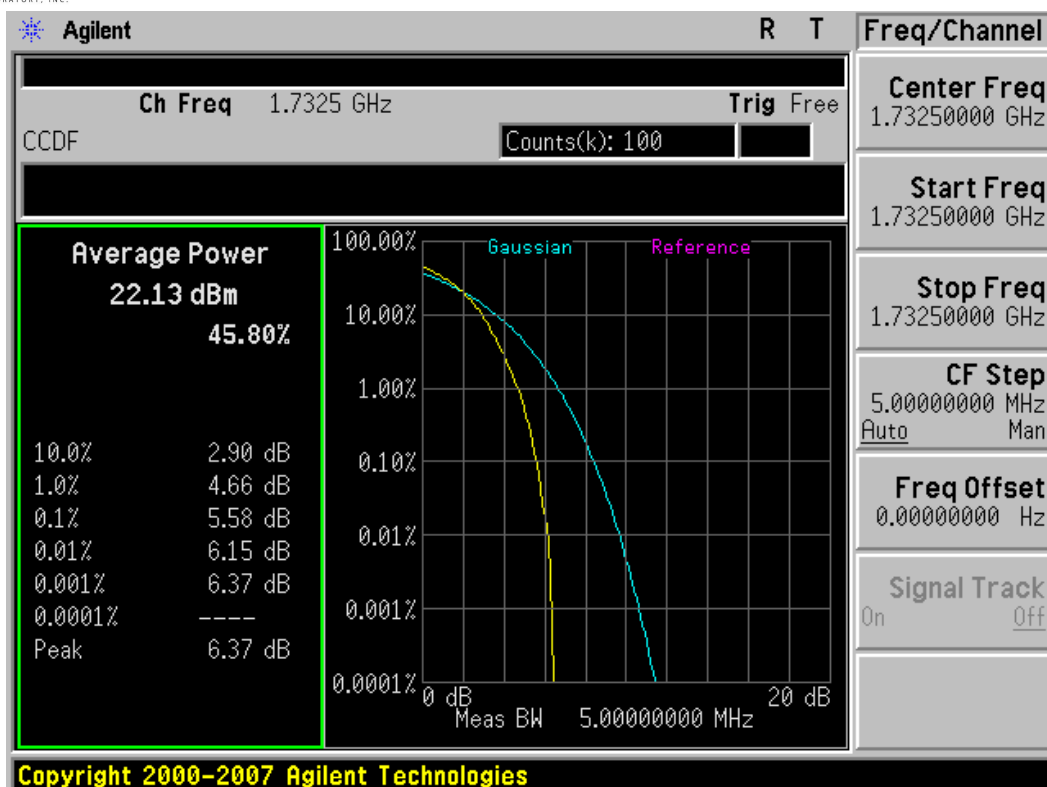
Plot 7-33. Peak-Average Ratio Plot (5MHz BW, 16-QAM, AWS Band – Mid Channel)
