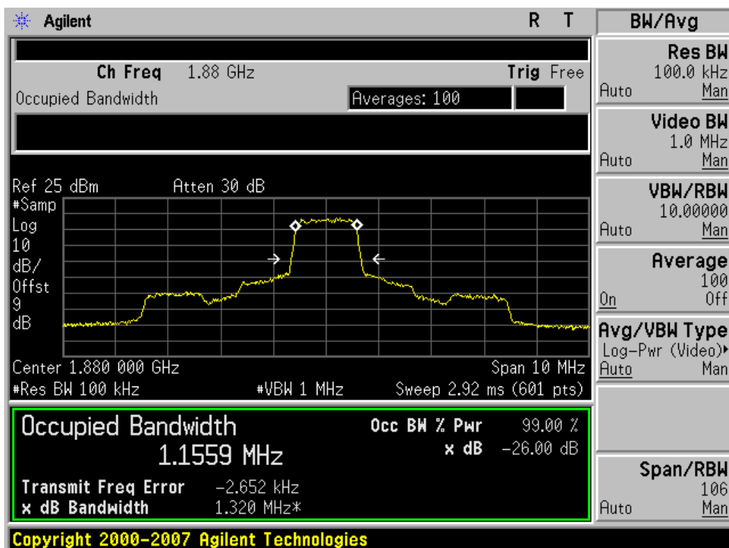
Plot 8-6. Occupied Bandwidth Plot (1.4MHz BW, QPSK, PCS Band – Mid Channel)
