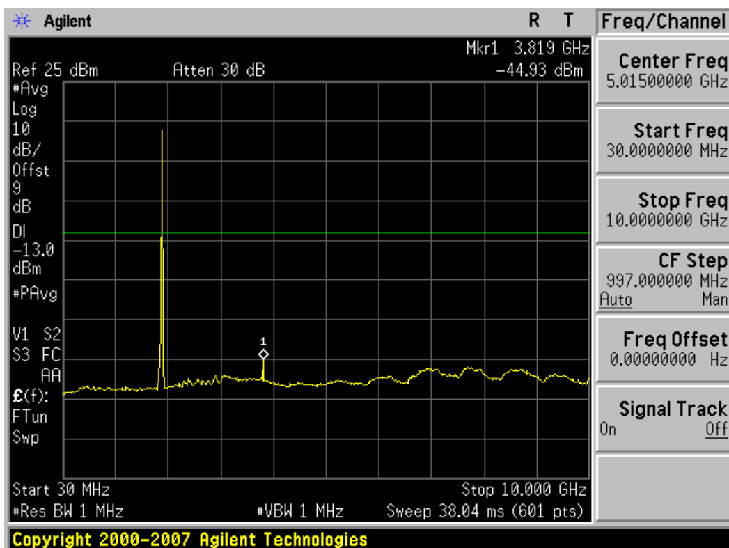
Plot 8-10. Conducted Spurious Plot (1.4MHz BW, QPSK, PCS Band – High Channel)
