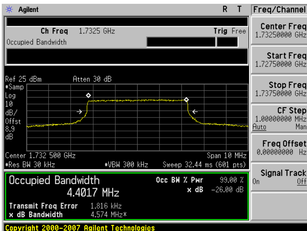
Plot 7-32. Occupied Bandwidth Plot (5MHz BW, 16-QAM, AWS Band – Mid Channel)
