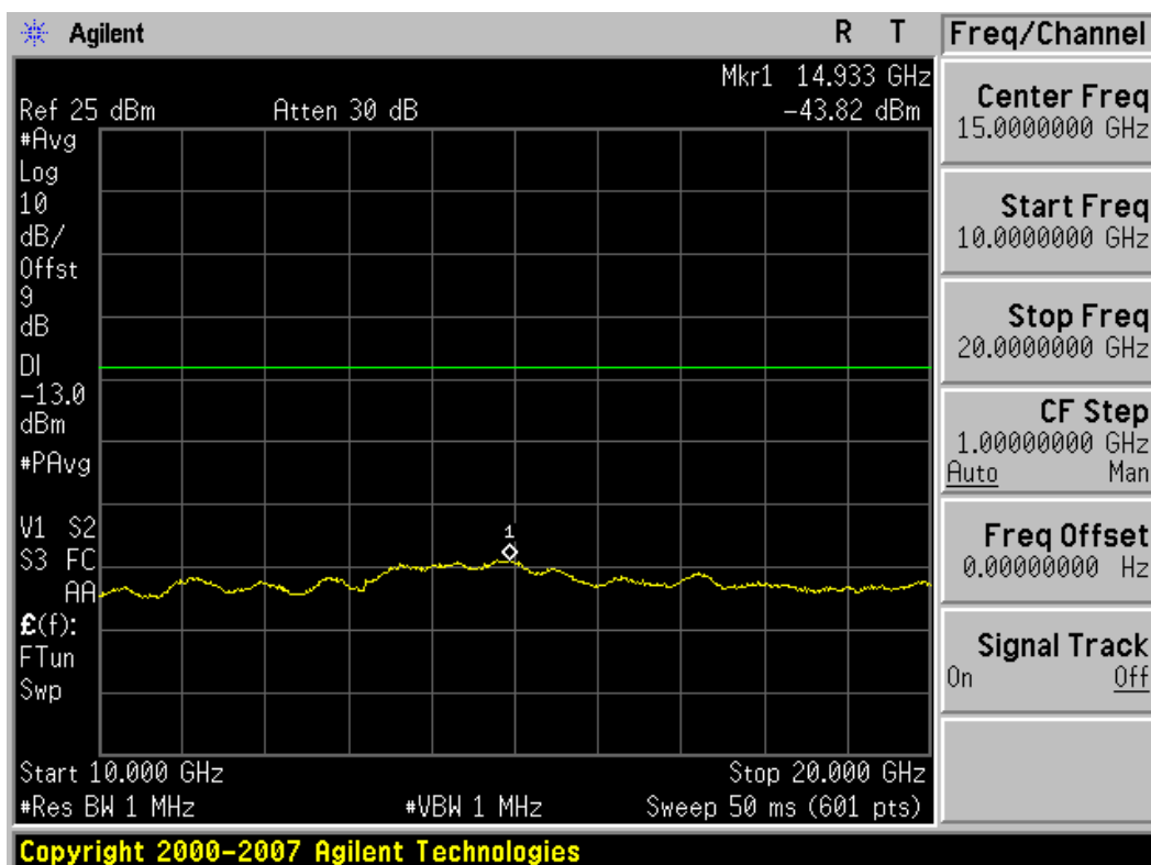
Plot 8-26. Conducted Spurious Plot (5MHz BW, QPSK, PCS Band – Low Channel)
