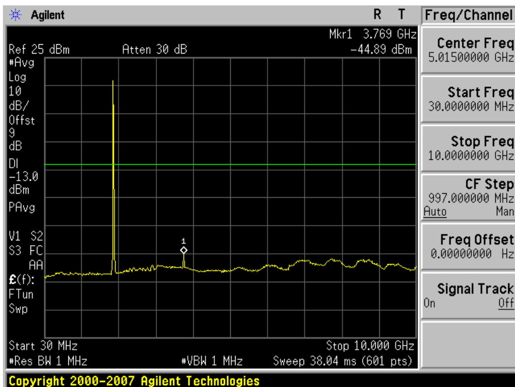
Plot 8-28. Conducted Spurious Plot (5MHz BW, QPSK, PCS Band – Mid Channel)
