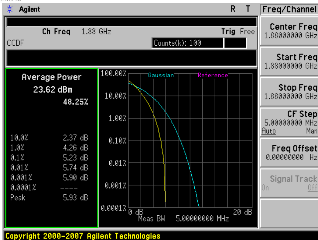
Plot 8-31. Peak-Average Ratio Plot (5MHz BW, QPSK, PCS Band – Mid Channel)
