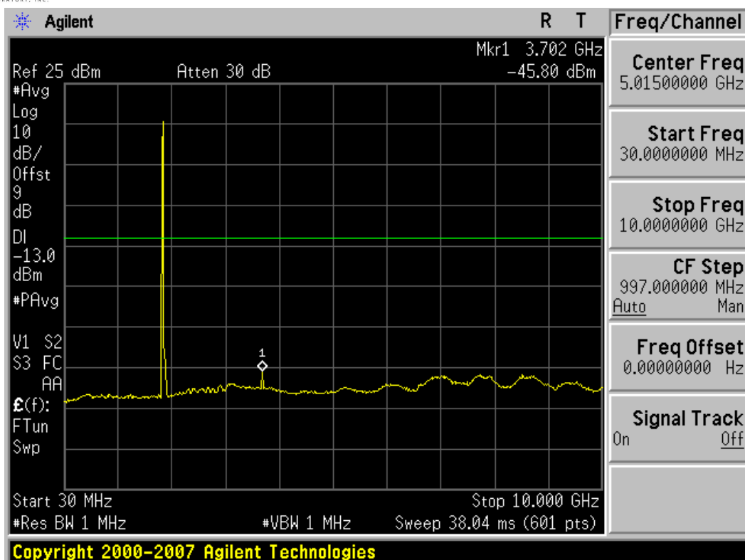
Plot 8-13. Conducted Spurious Plot (3MHz BW, QPSK, PCS Band – Low Channel)
