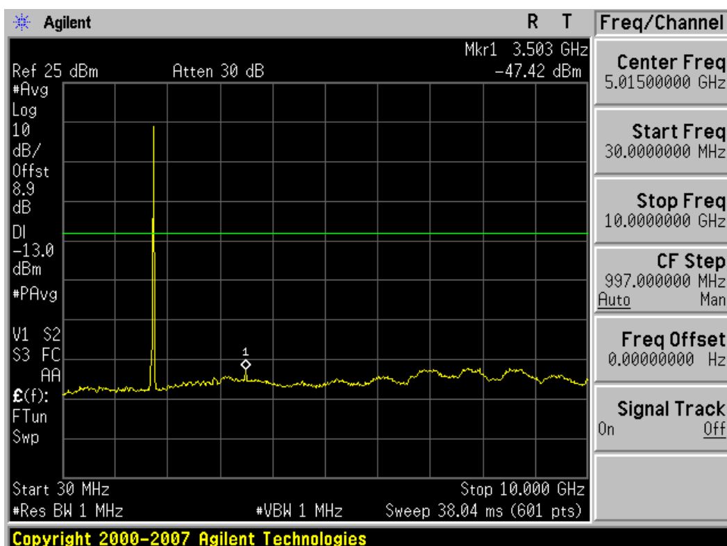
Plot 7-22. Conducted Spurious Plot (3MHz BW, QPSK, AWS Band – High Channel)
