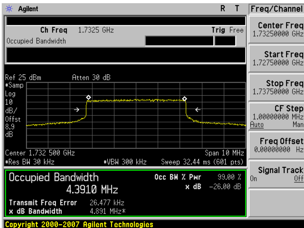
Plot 7-30. Occupied Bandwidth Plot (5MHz BW, QPSK, AWS Band – Mid Channel)
