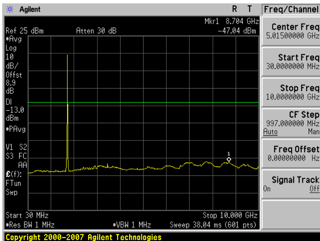
Plot 7-28. Conducted Spurious Plot (5MHz BW, QPSK, AWS Band – Mid Channel)
