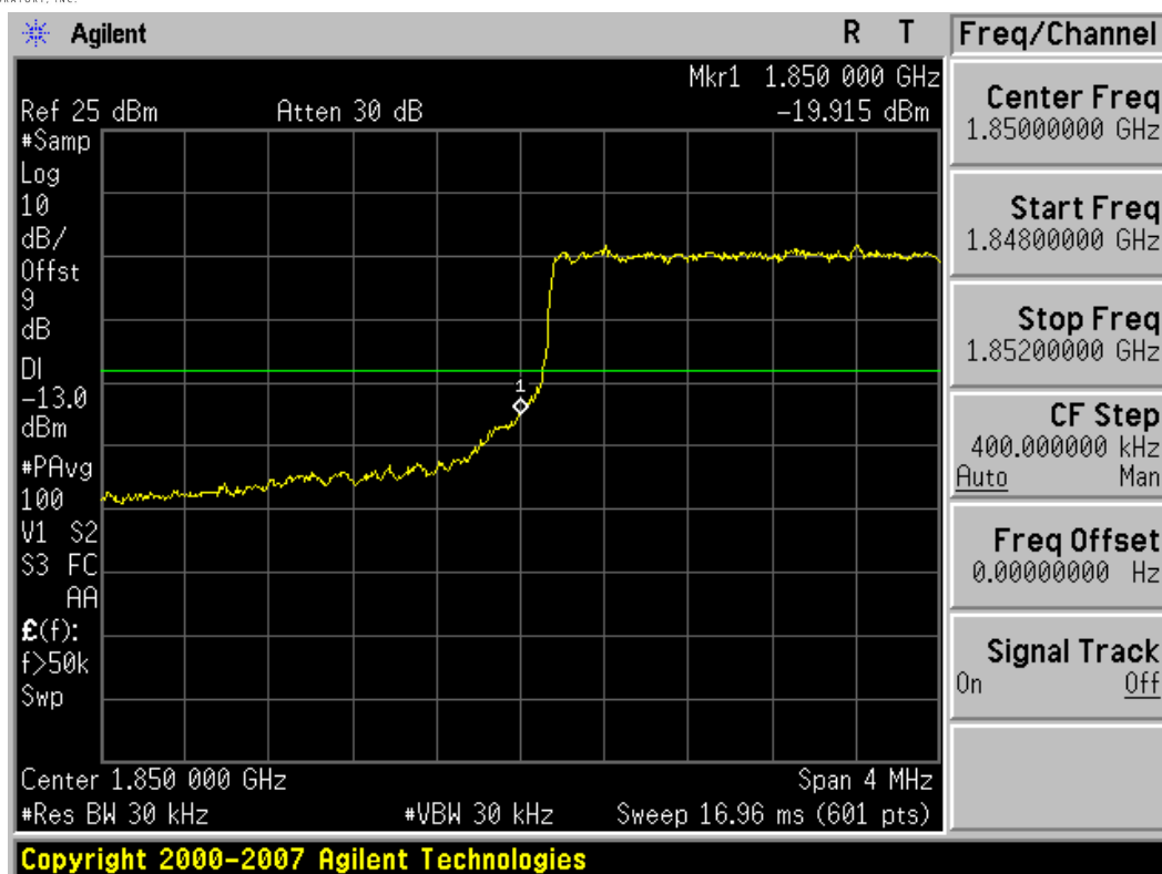
Plot 8-15. Band Edge Plot (3MHz BW, QPSK, PCS Band – Low Channel)
