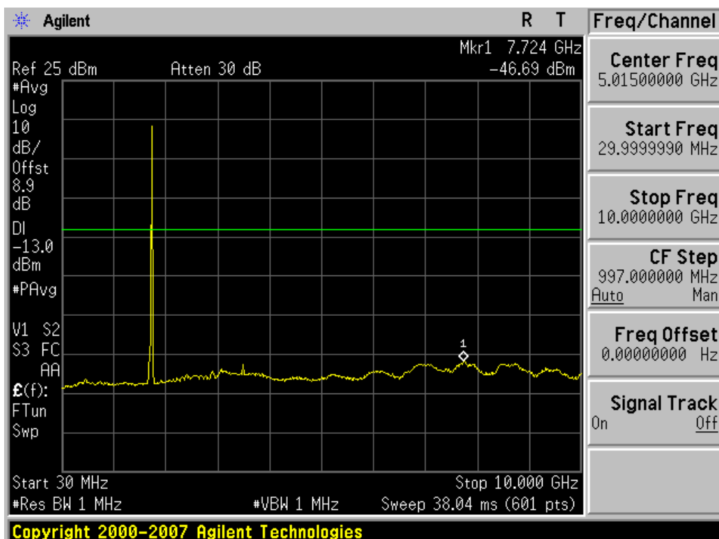
Plot 7-10. Conducted Spurious Plot (1.4MHz BW, QPSK, AWS Band – High Channel)
