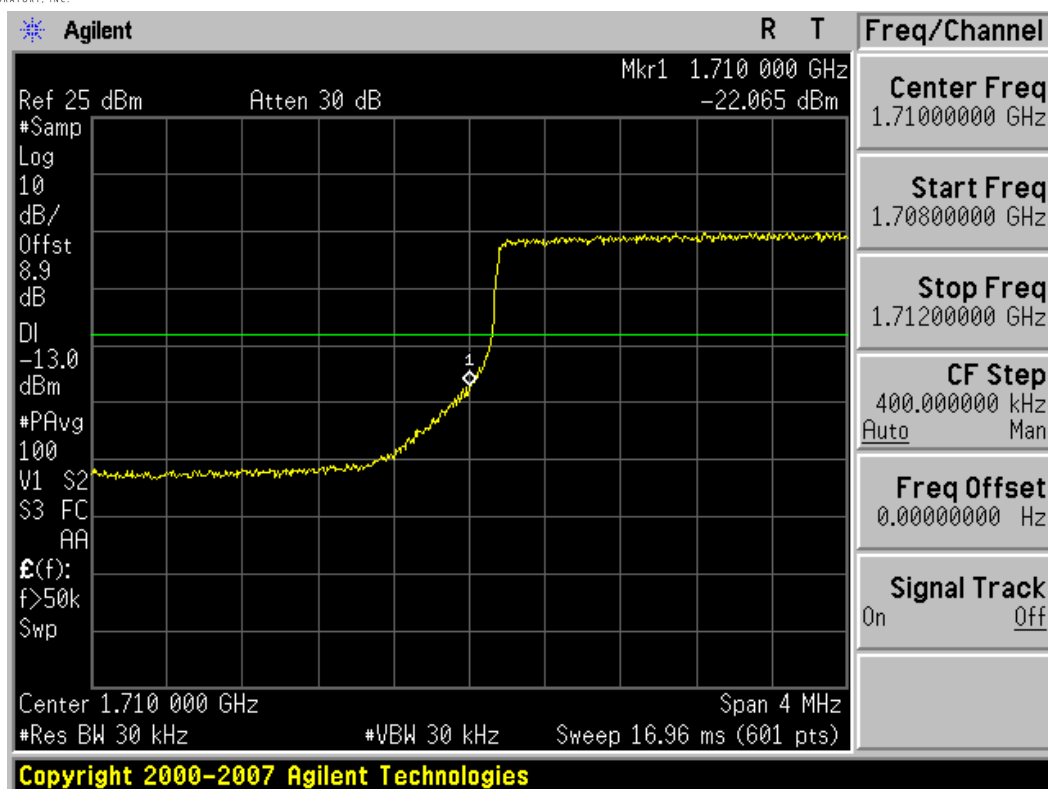
Plot 7-15. Band Edge Plot (3MHz BW, QPSK, AWS Band – Low Channel)
