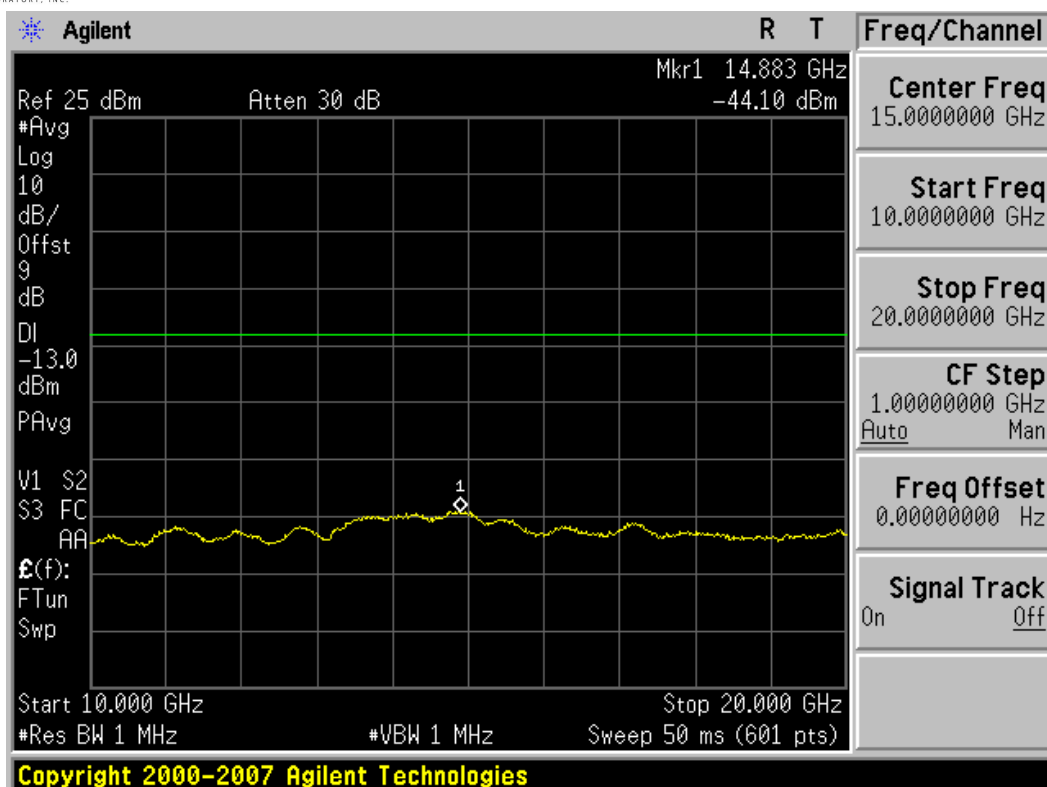
Plot 8-29. Conducted Spurious Plot (5MHz BW, QPSK, PCS Band – Mid Channel)
