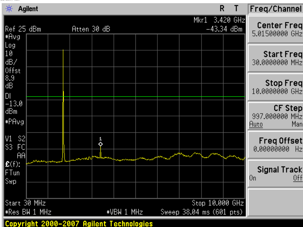
Plot 7-25. Conducted Spurious Plot (5MHz BW, QPSK, AWS Band – Low Channel)
