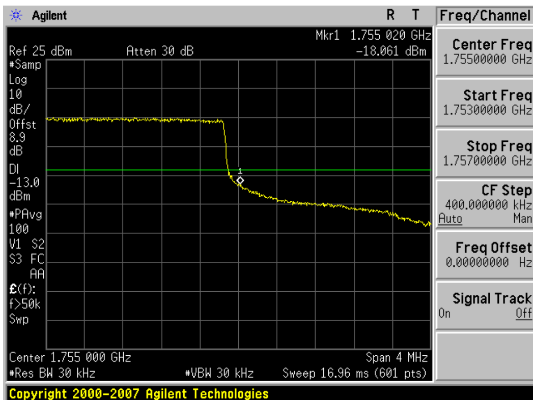
Plot 7-24. Band Edge Plot (3MHz BW, QPSK, AWS Band – High Channel)
