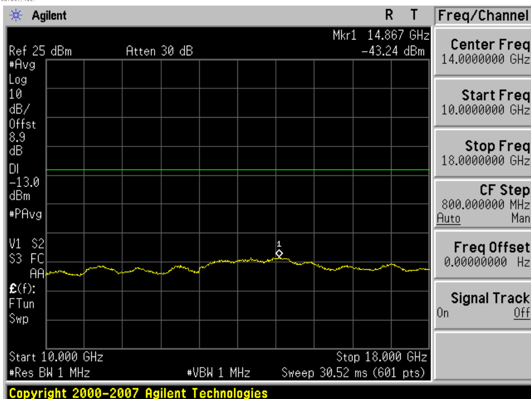
Plot 7-35. Conducted Spurious Plot (5MHz BW, QPSK, AWS Band – High Channel)
