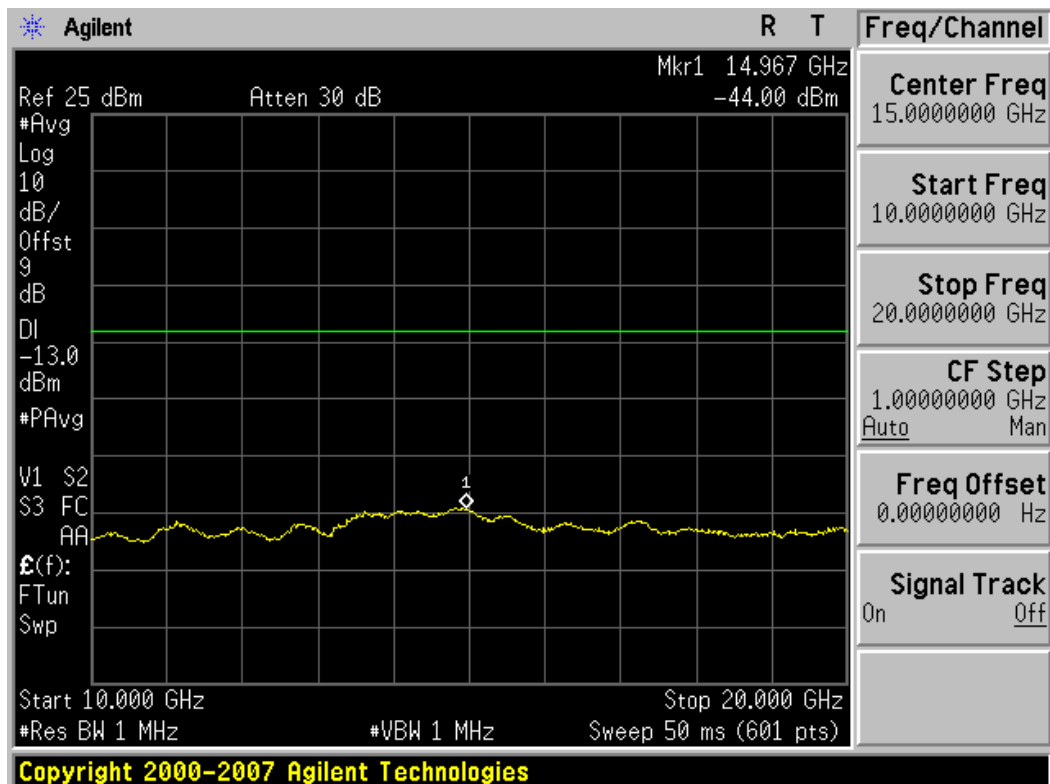
Plot 8-17. Conducted Spurious Plot (3MHz BW, QPSK, PCS Band – Mid Channel)
