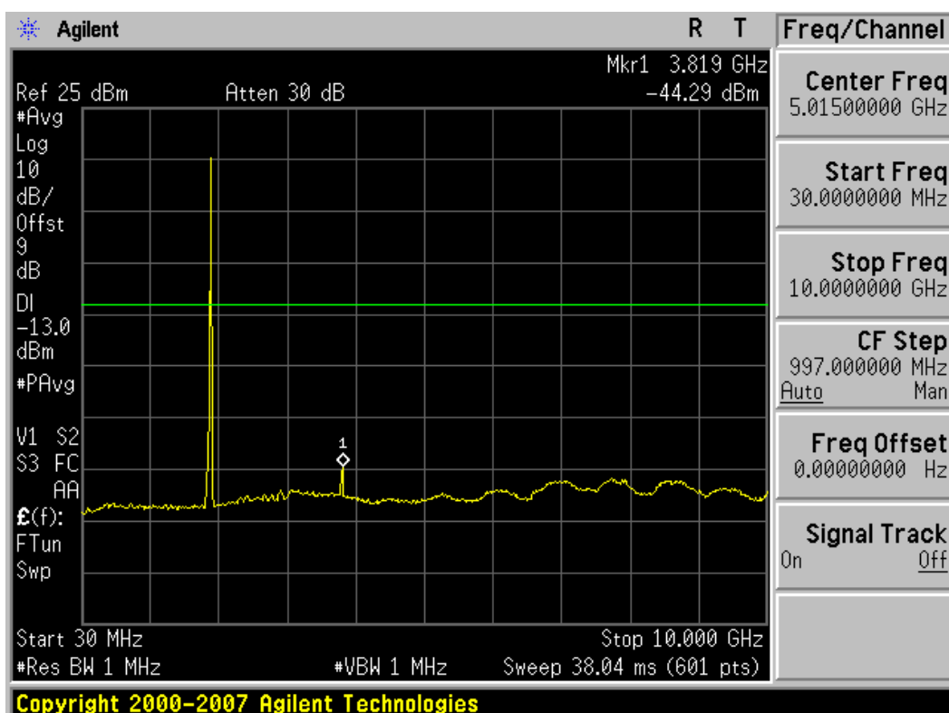
Plot 8-34. Conducted Spurious Plot (5MHz BW, QPSK, PCS Band – High Channel)
