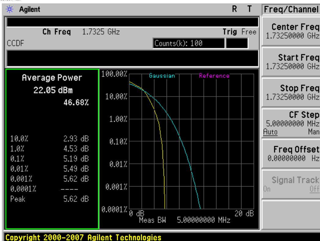
Plot 7-9. Peak-Average Ratio Plot (1.4MHz BW, 16-QAM, AWS Band – Mid Channel)
