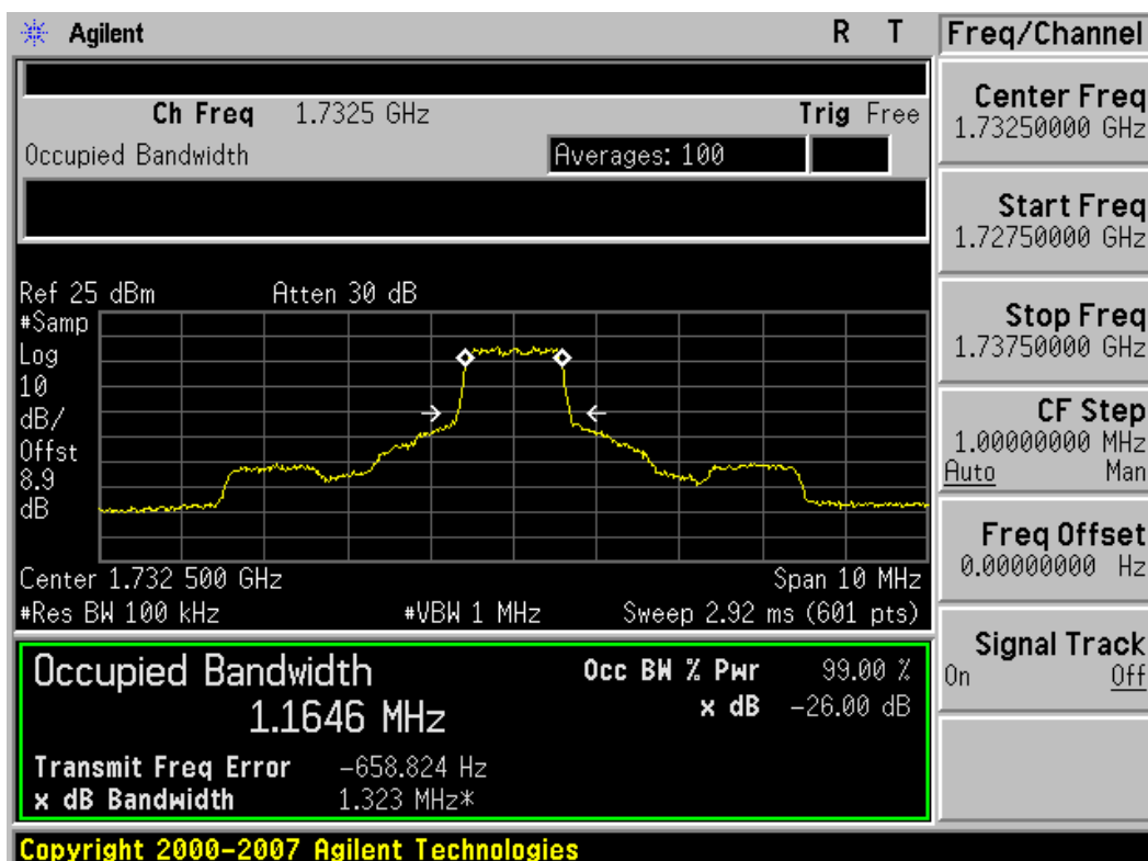
Plot 7-6. Occupied Bandwidth Plot (1.4MHz BW, QPSK, AWS Band – Mid Channel)
