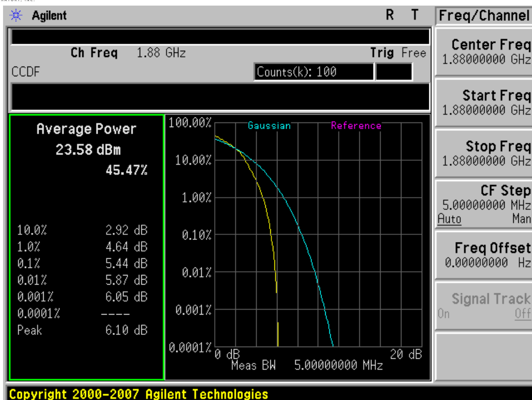
Plot 8-21. Peak-Average Ratio Plot (3MHz BW, 16-QAM, PCS Band – Mid Channel)
