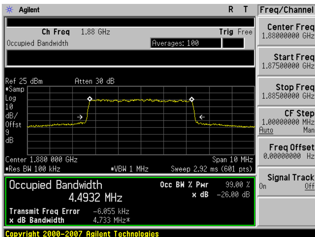
Plot 8-30. Occupied Bandwidth Plot (5MHz BW, QPSK, PCS Band – Mid Channel)
