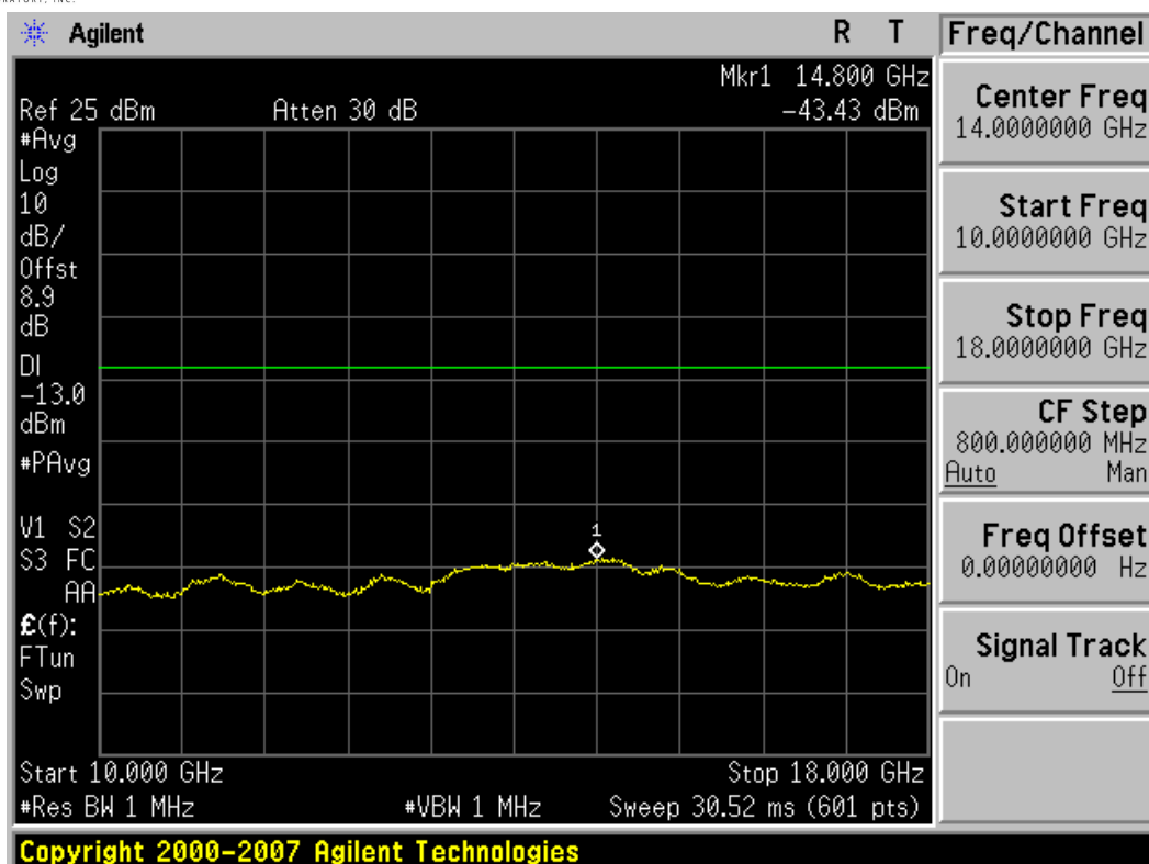
Plot 7-29. Conducted Spurious Plot (5MHz BW, QPSK, AWS Band – Mid Channel)
