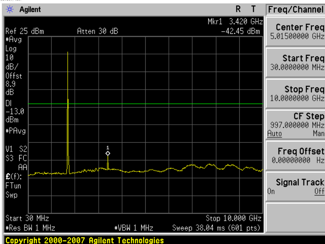
Plot 7-13. Conducted Spurious Plot (3MHz BW, QPSK, AWS Band – Low Channel)
