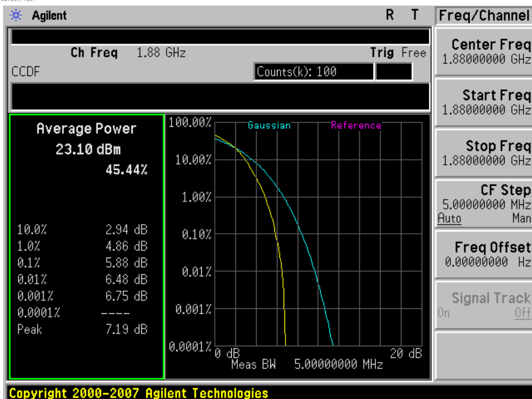
Plot 8-33. Peak-Average Ratio Plot (5MHz BW, 16-QAM, PCS Band – Mid Channel)
