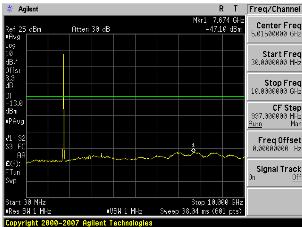
Plot 7-4. Conducted Spurious Plot (1.4MHz BW, QPSK, AWS Band – Mid Channel)
