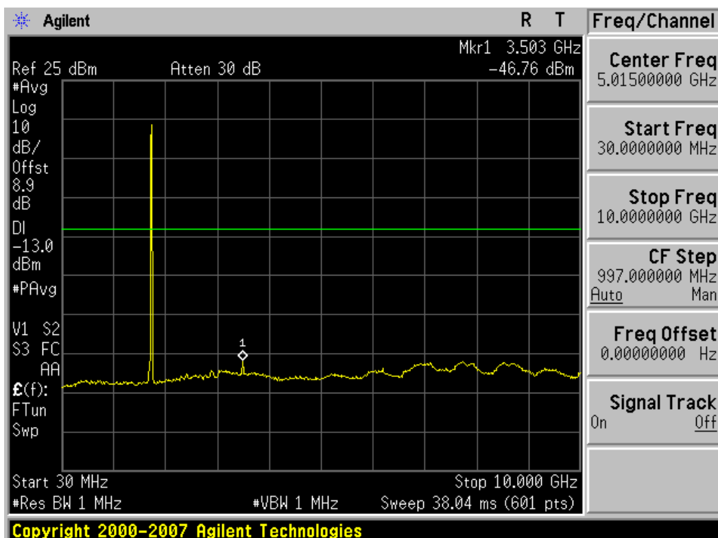
Plot 7-34. Conducted Spurious Plot (5MHz BW, QPSK, AWS Band – High Channel)
