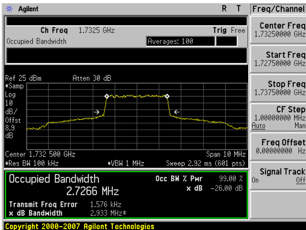
Plot 7-18. Occupied Bandwidth Plot (3MHz BW, QPSK, AWS Band – Mid Channel)
