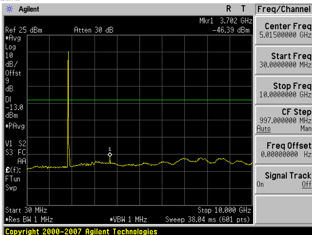
Plot 8-25. Conducted Spurious Plot (5MHz BW, QPSK, PCS Band – Low Channel)
