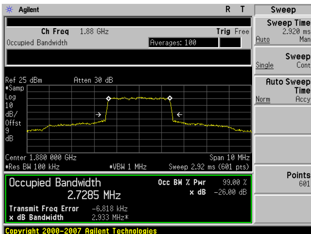
Plot 8-20. Occupied Bandwidth Plot (3MHz BW, 16-QAM, PCS Band – Mid Channel)
