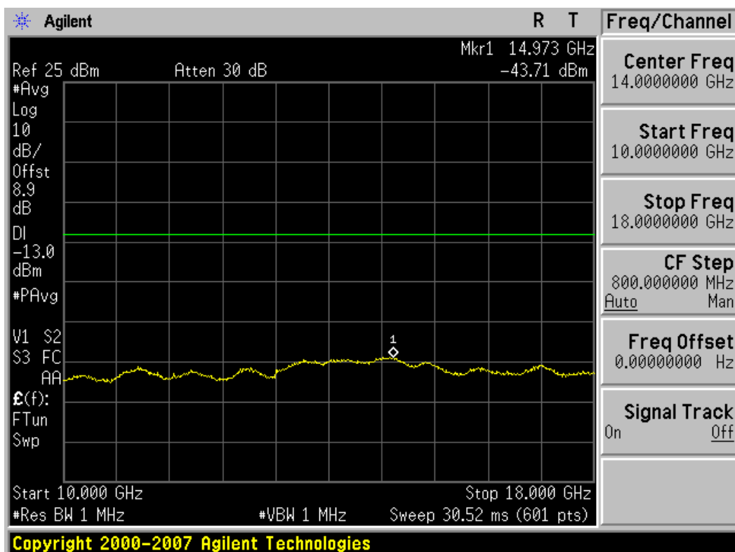
Plot 7-26. Conducted Spurious Plot (5MHz BW, QPSK, AWS Band – Low Channel)
