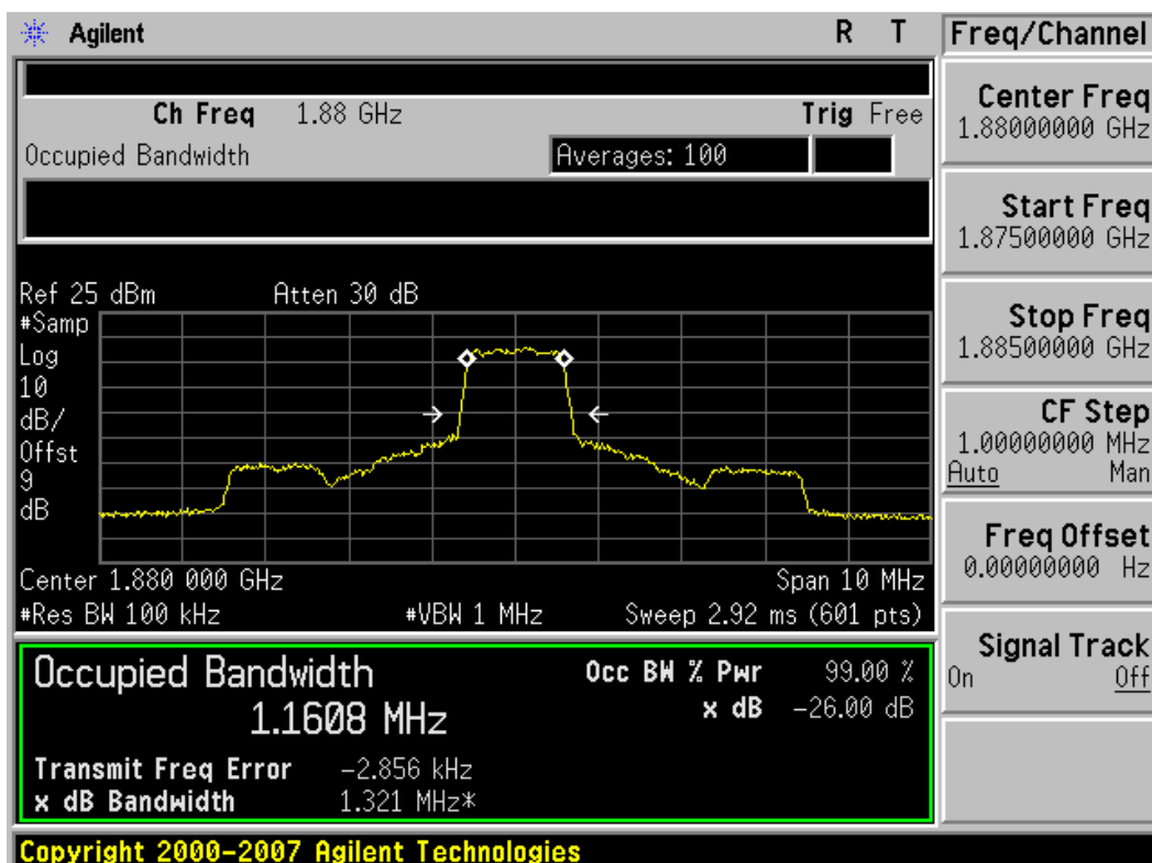
Plot 8-8. Occupied Bandwidth Plot (1.4MHz BW, 16-QAM, PCS Band – Mid Channel)
