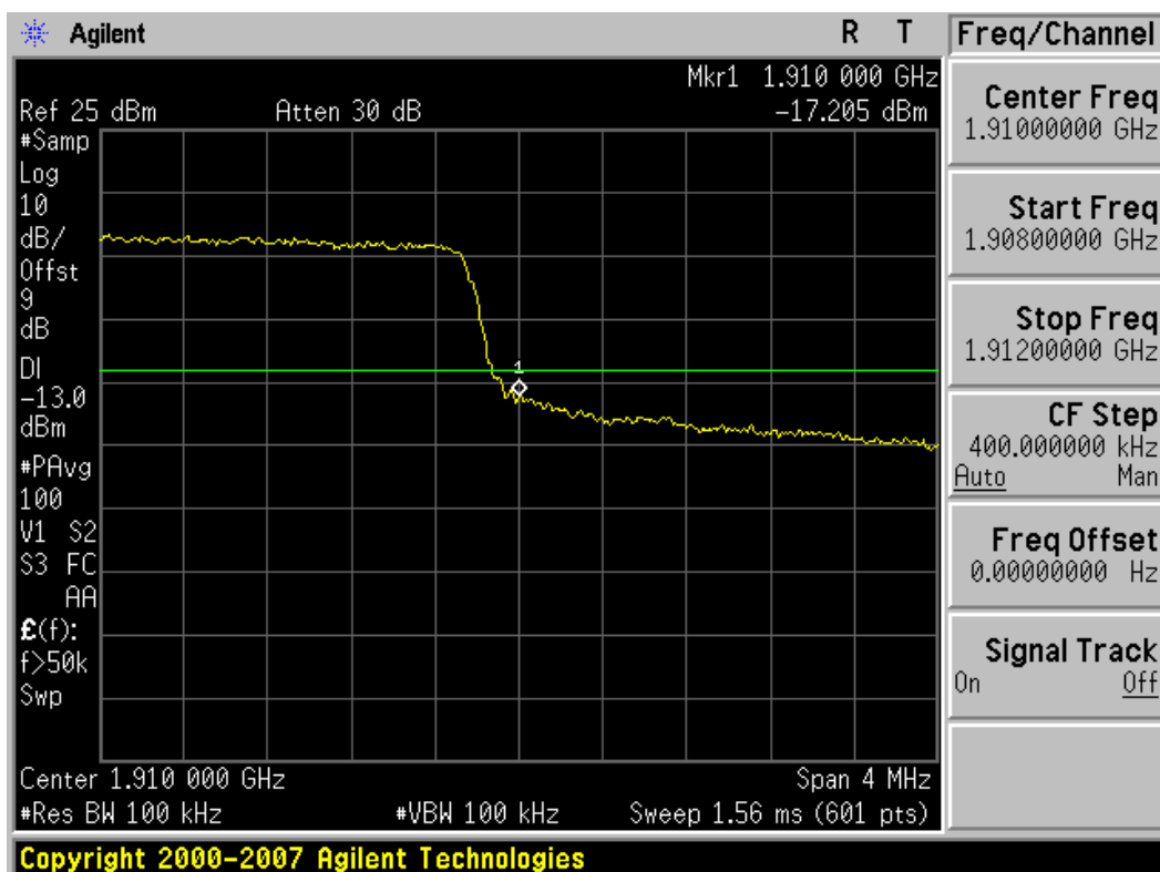
Plot 8-36. Band Edge Plot (5MHz BW, QPSK, PCS Band – High Channel)
