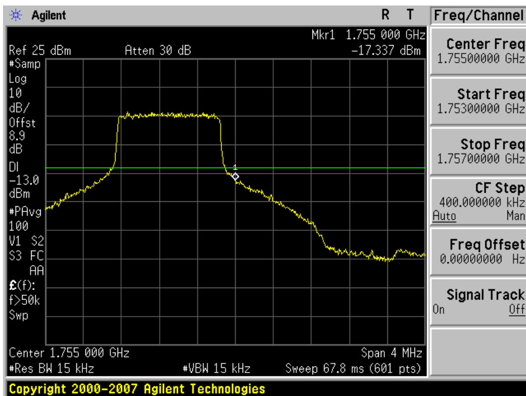
Plot 7-12. Band Edge Plot (1.4MHz BW, QPSK, AWS Band – High Channel)
