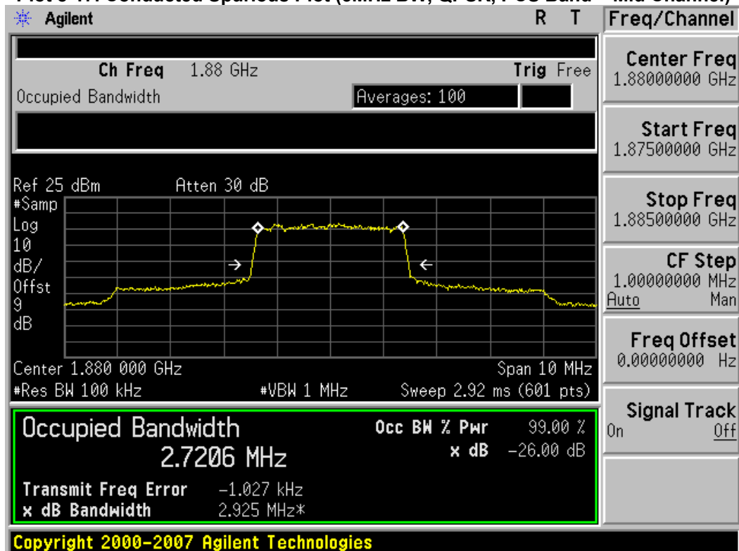
Plot 8-18. Occupied Bandwidth Plot (3MHz BW, QPSK, PCS Band – Mid Channel)
