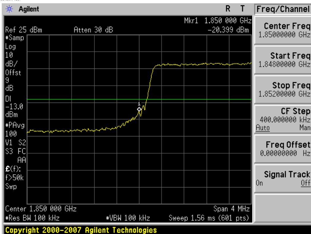
Plot 8-27. Band Edge Plot (5MHz BW, QPSK, PCS Band – Low Channel)
