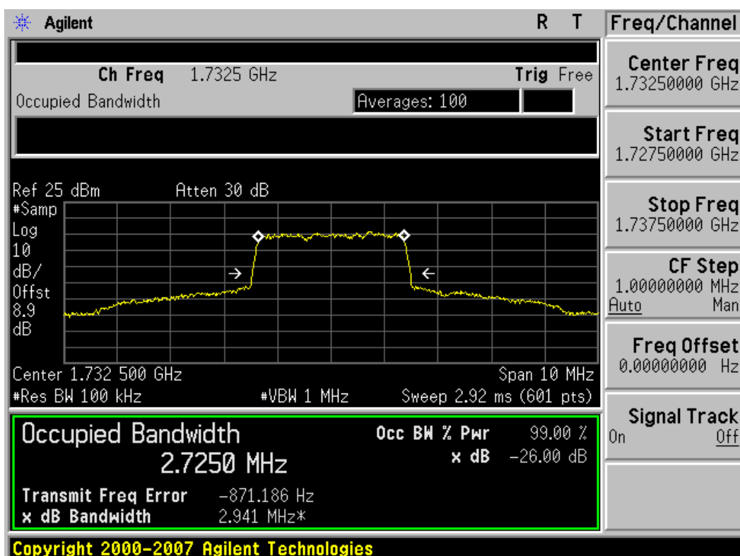
Plot 7-20. Occupied Bandwidth Plot (3MHz BW, 16-QAM, AWS Band – Mid Channel)
