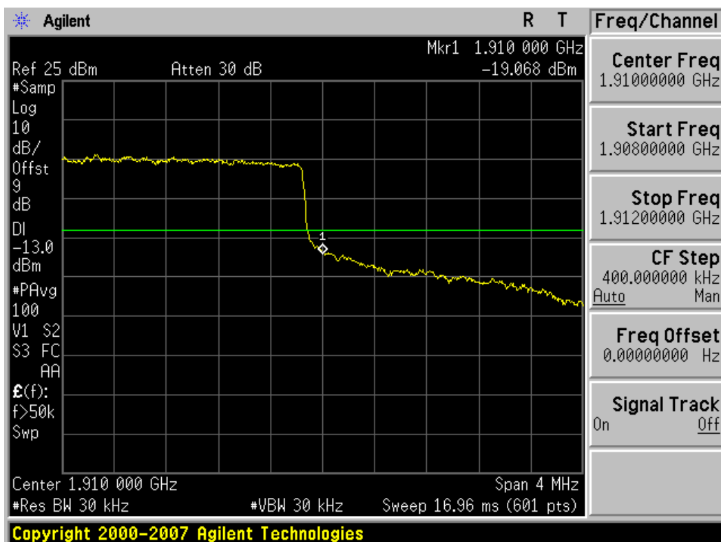
Plot 8-24. Band Edge Plot (3MHz BW, QPSK, PCS Band – High Channel)
