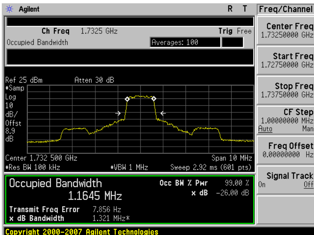
Plot 7-8. Occupied Bandwidth Plot (1.4MHz BW, 16-QAM, AWS Band – Mid Channel)
