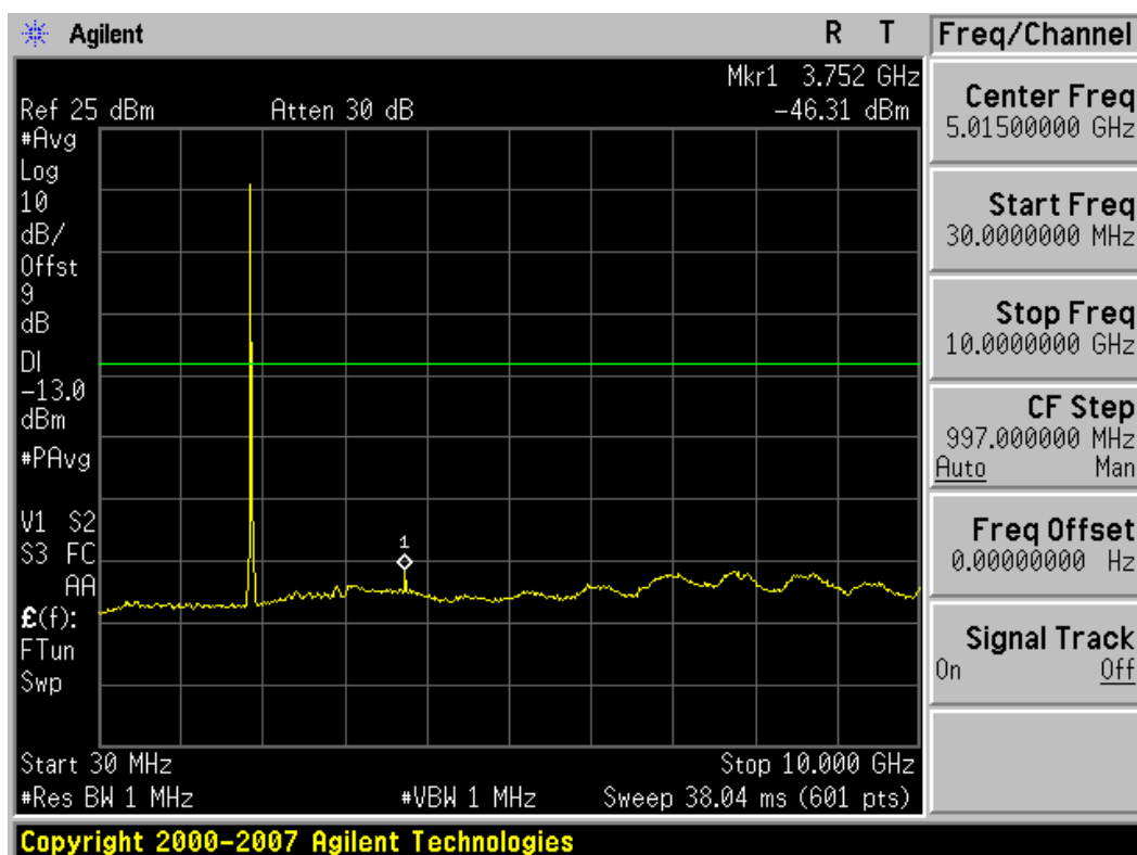
Plot 8-4. Conducted Spurious Plot (1.4MHz BW, QPSK, PCS Band – Mid Channel)
