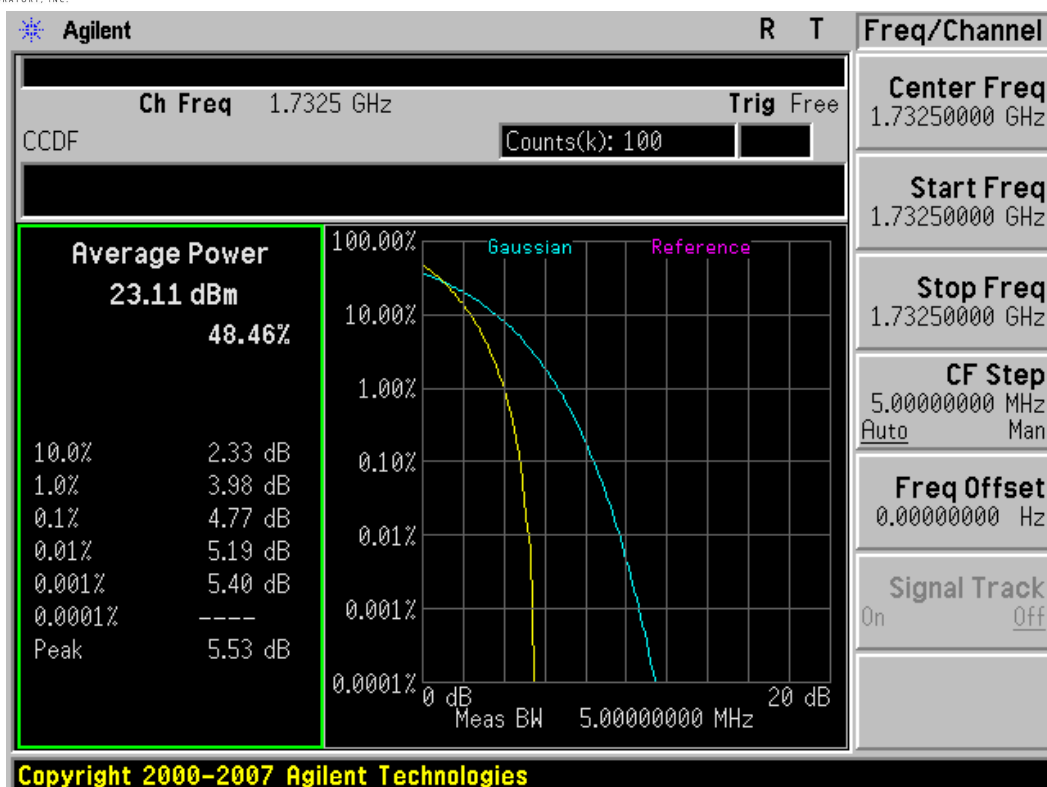
Plot 7-31. Peak-Average Ratio Plot (5MHz BW, QPSK, AWS Band – Mid Channel)
