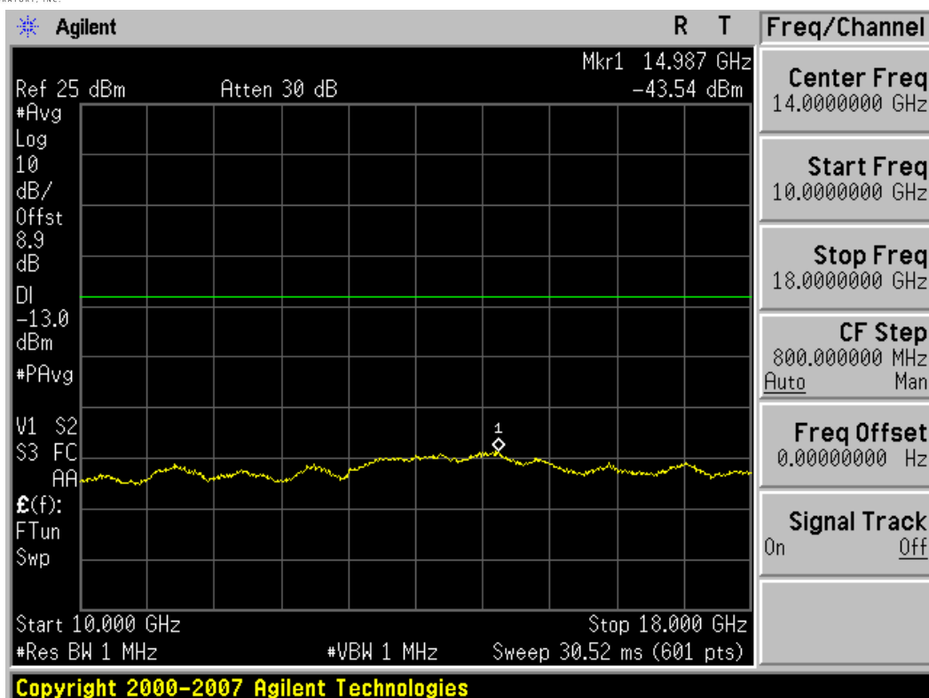
Plot 7-17. Conducted Spurious Plot (3MHz BW, QPSK, AWS Band – Mid Channel)
