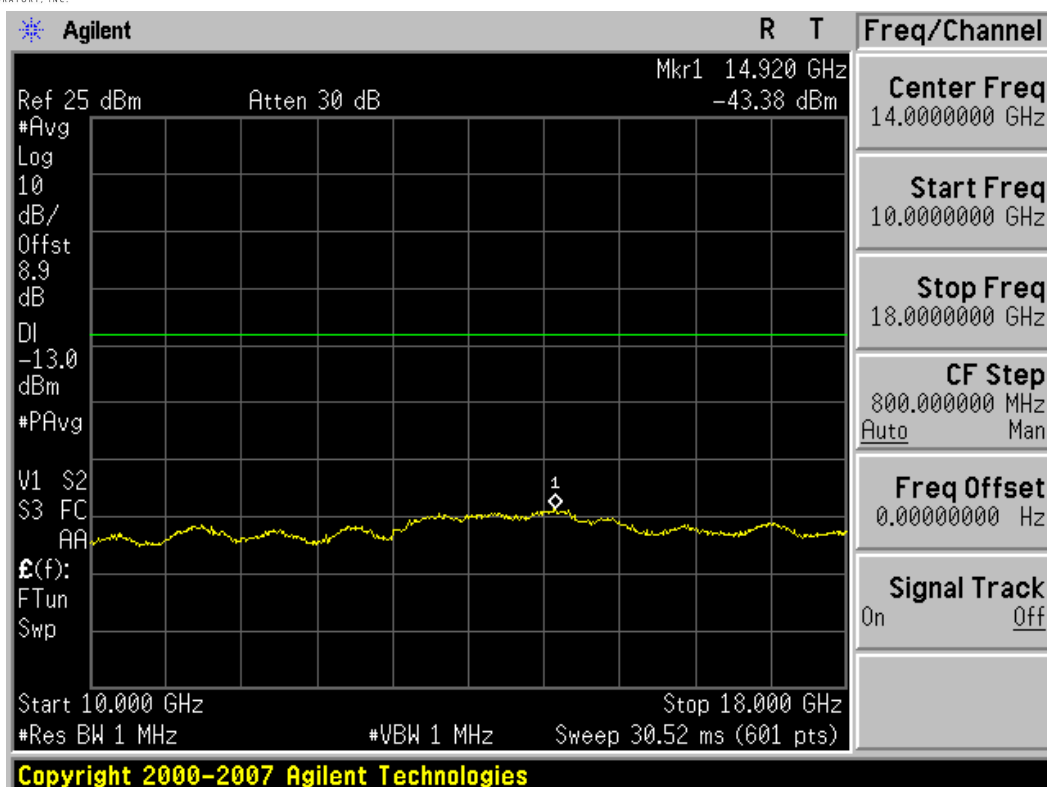
Plot 7-23. Conducted Spurious Plot (3MHz BW, QPSK, AWS Band – High Channel)
