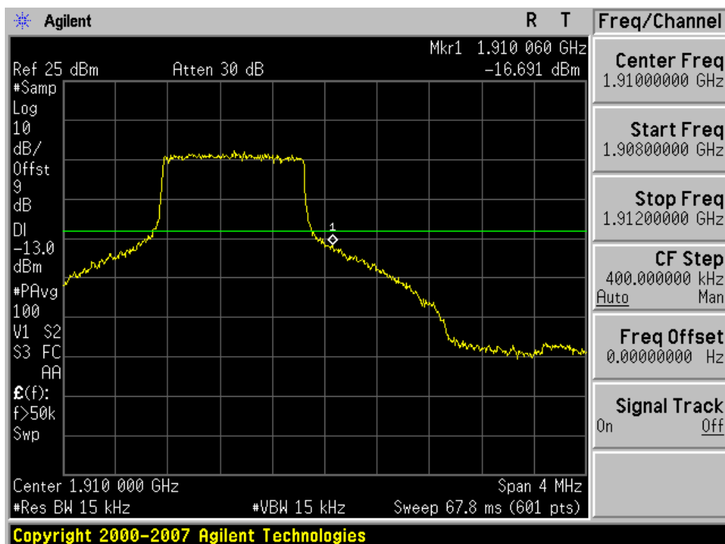
Plot 8-12. Band Edge Plot (1.4MHz BW, QPSK, PCS Band – High Channel)
