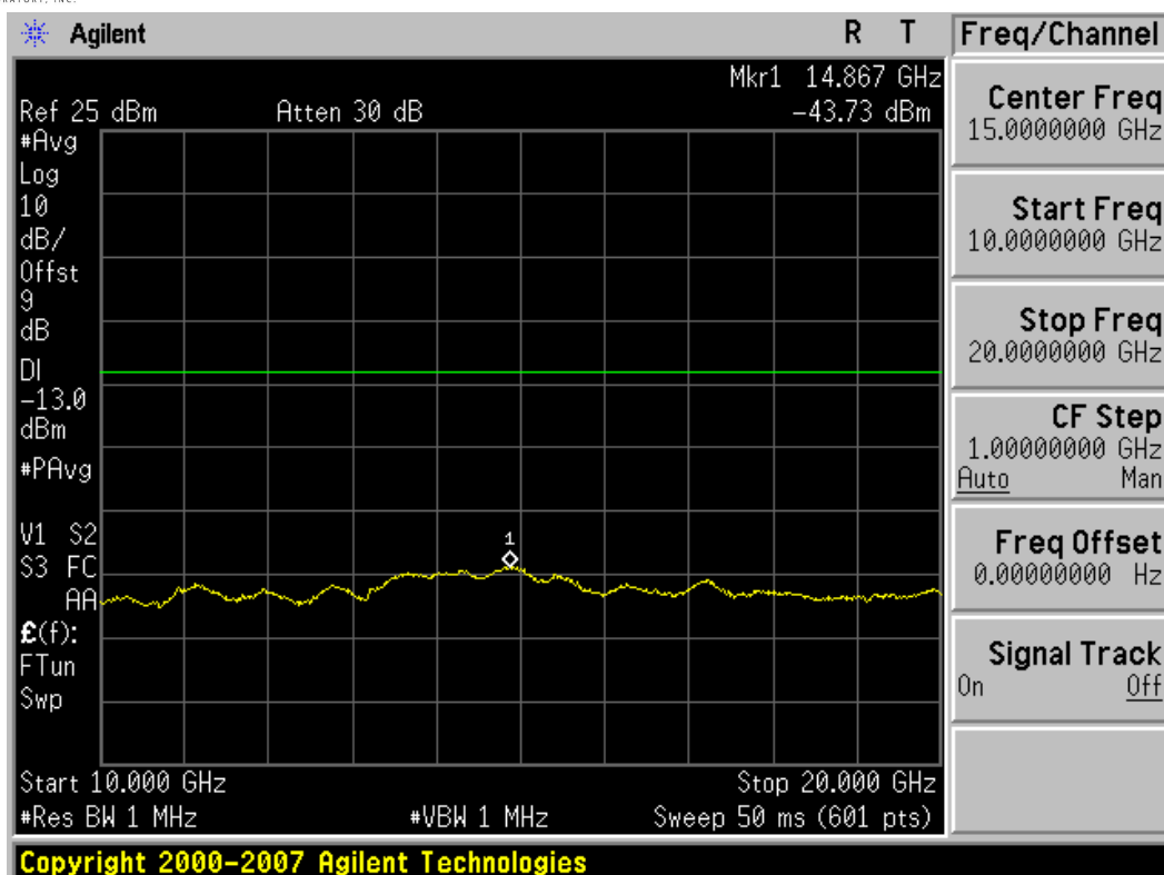
Plot 8-23. Conducted Spurious Plot (3MHz BW, QPSK, PCS Band – High Channel)
