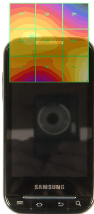
Figure 17-5 H-Field WD Scan overlay
