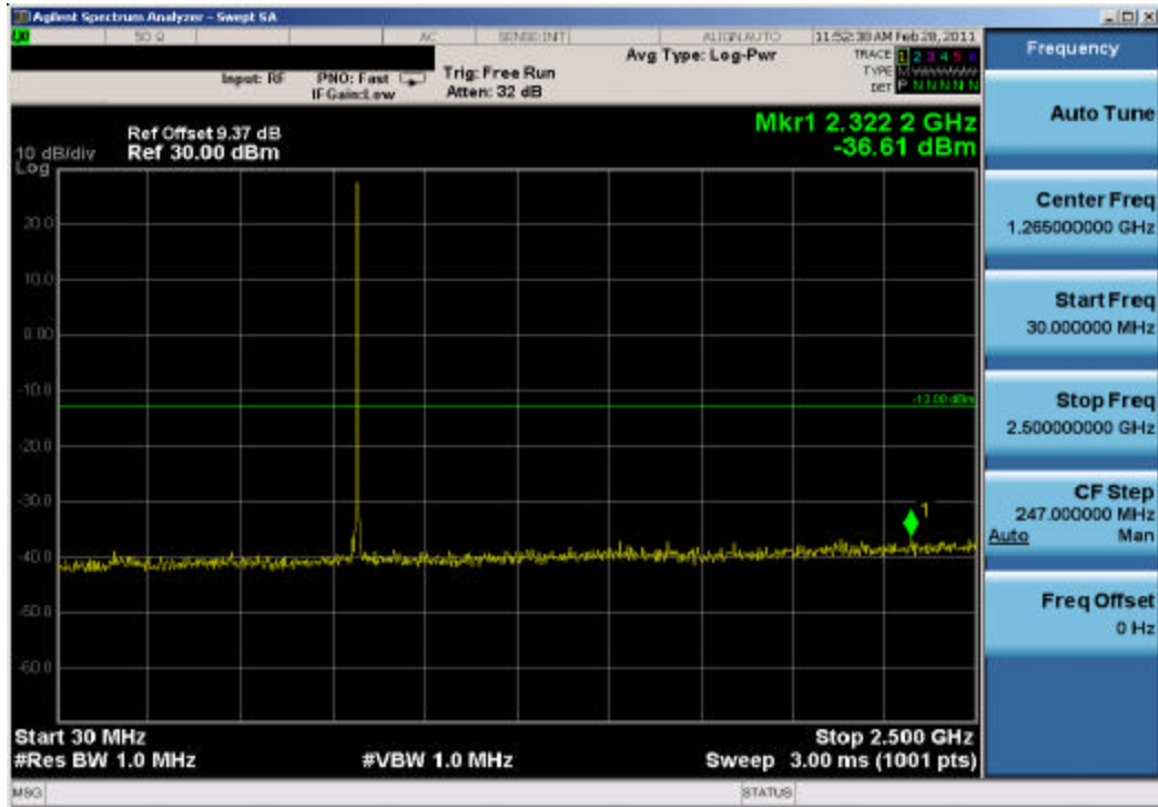
Plot 7-5. Conducted Spurious Plot (Cellular CDMA Mode – Ch. 384)
