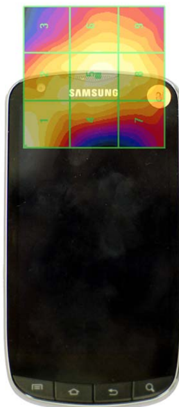
Figure 17-5 H-Field WD Scan overlay
