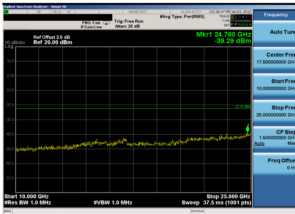
Plot 6-30. Conducted Spurious Plot (802.11b – Ch. 11)
