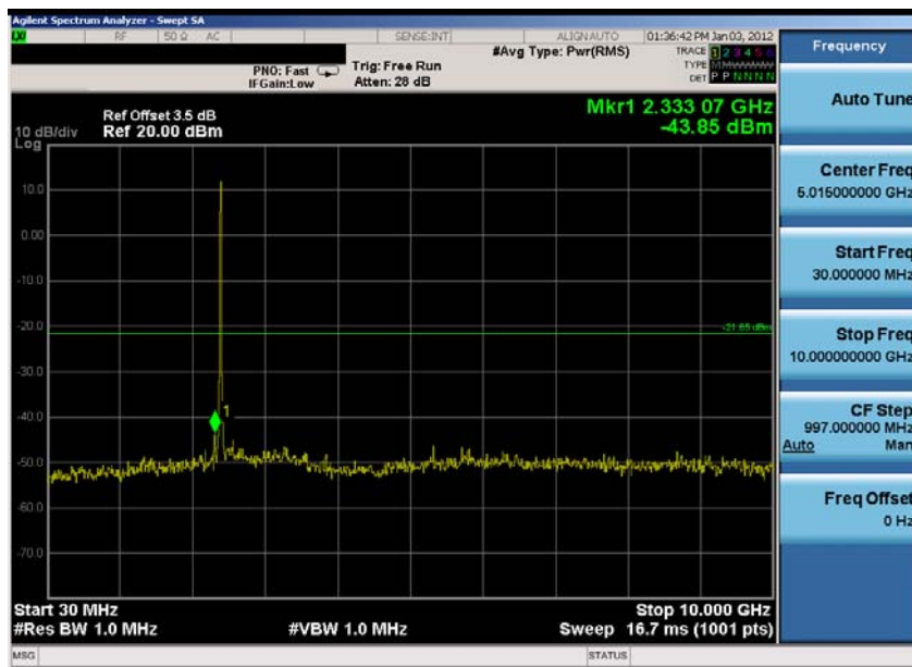
Plot 6-25. Conducted Spurious Plot (802.11b – Ch. 1)
