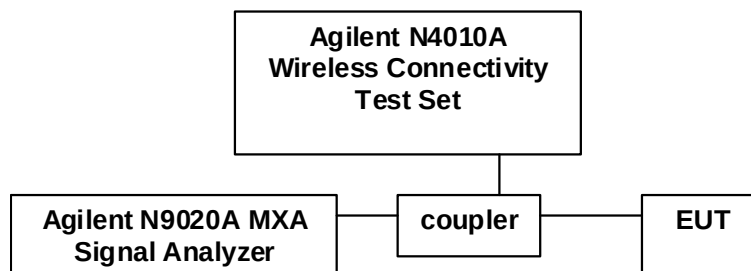
Figure 6-2. Test Instrument & Measurement Setup
