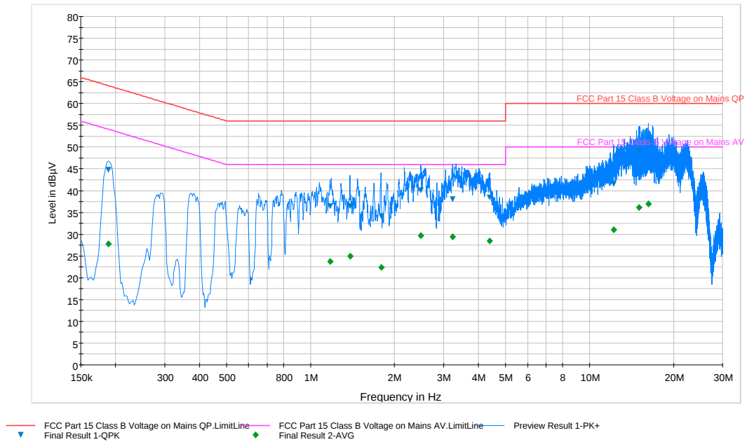
Plot 6-59. Line Conducted Plot with 802.11b (L1)
