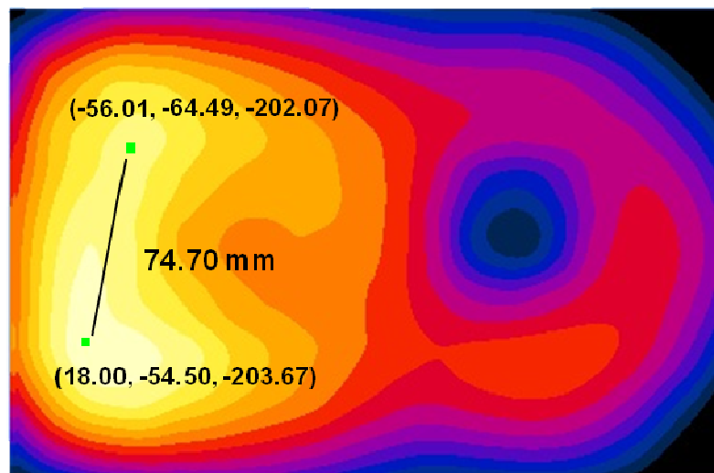
Figure 12-1 Peak SAR Location Plot of PCS CDMA and LTE Band 4
