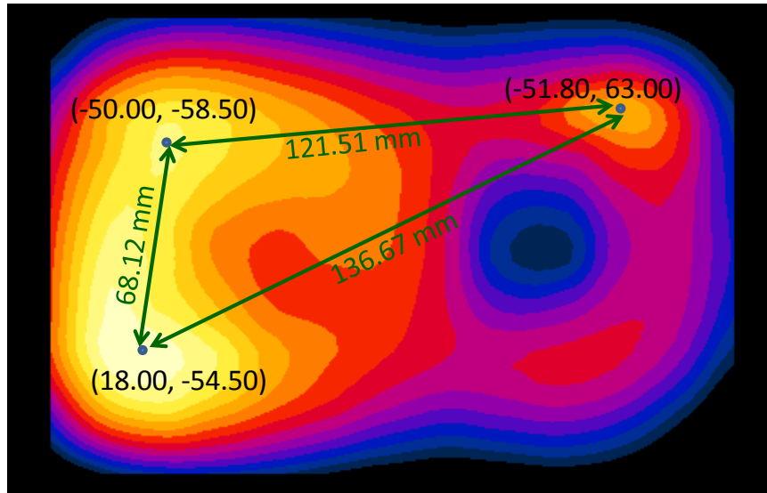
Figure 12-1 Peak SAR location plots of PCS CDMA, LTE B2, and 2.4 GHz WLAN at 10 mm.
