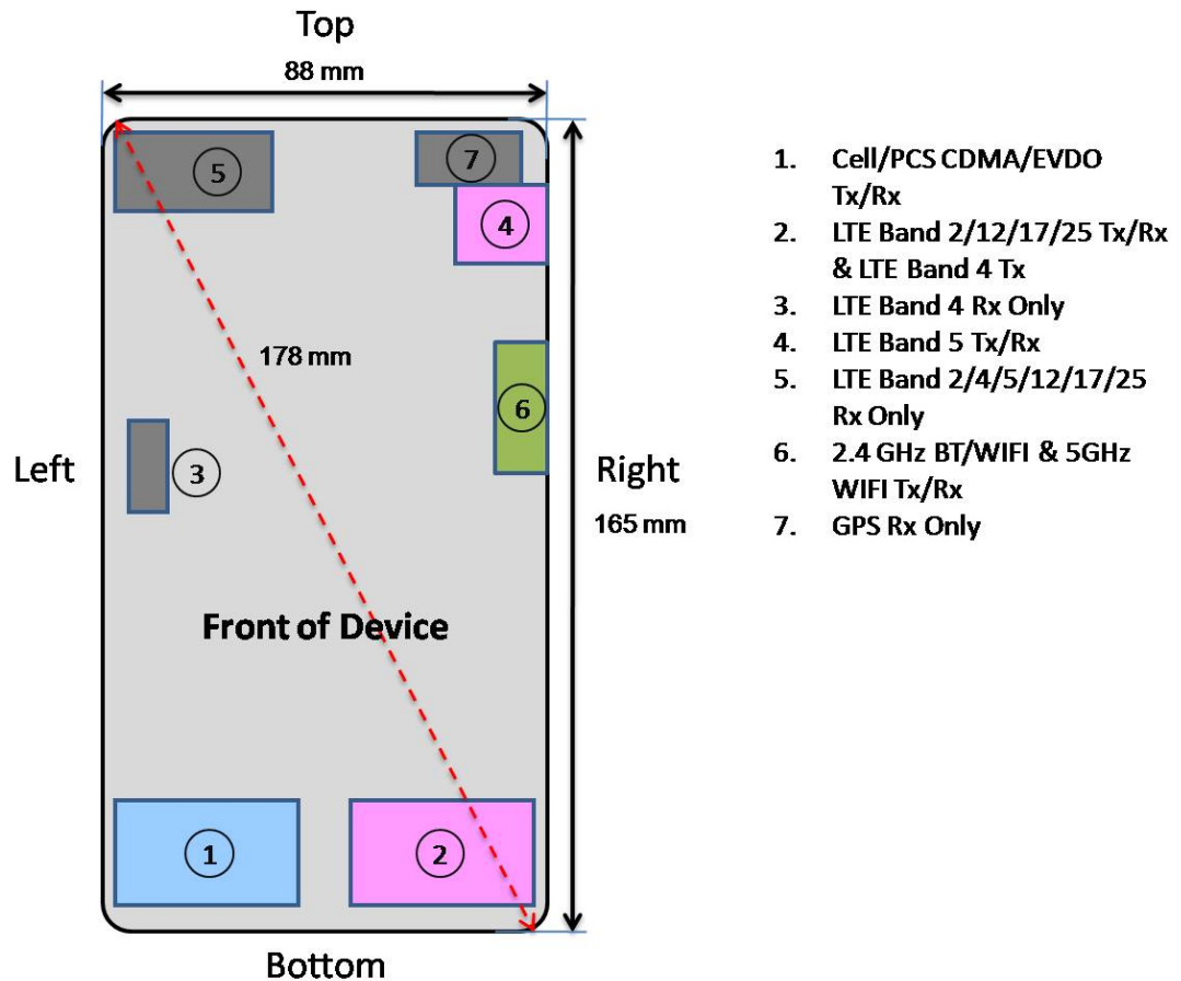
Figure 1-1 DUT Antenna Locations
