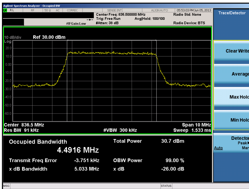
Plot 9-3. Occupied Bandwidth Plot (5.0MHz QPSK – RB Size 25)
