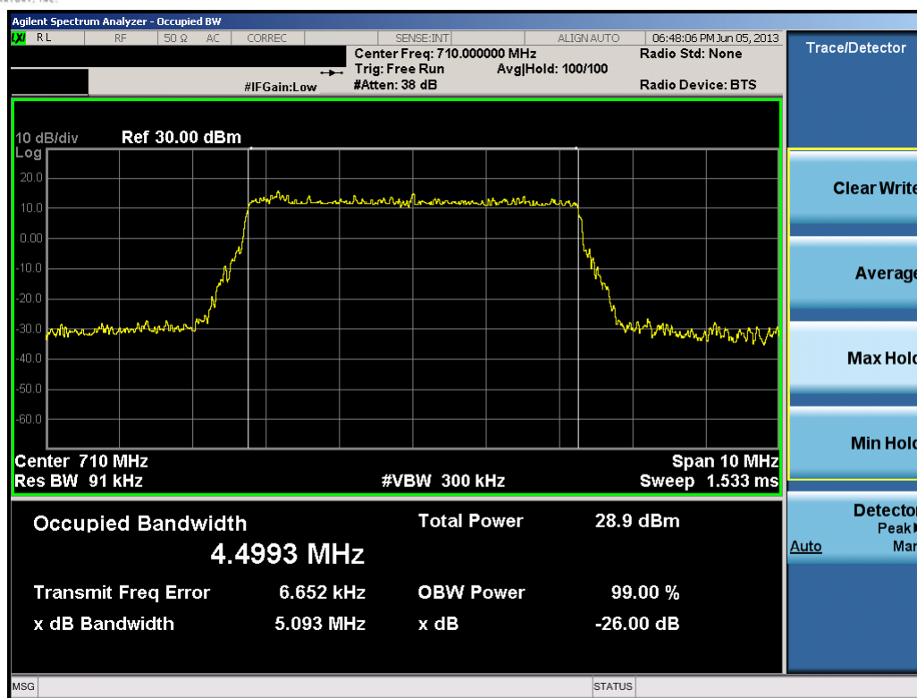
Plot 8-4. Occupied Bandwidth Plot (5.0MHz 16-QAM – RB Size 25)
