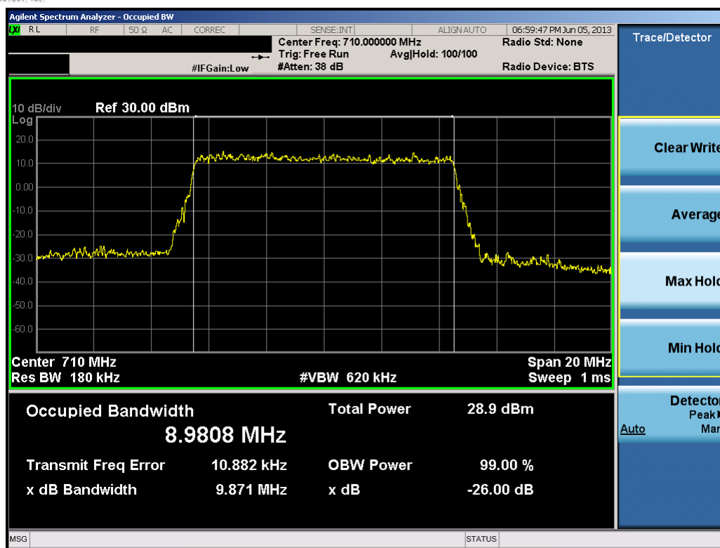
Plot 8-16. Occupied Bandwidth Plot (10.0MHz 16-QAM – RB Size 50)
