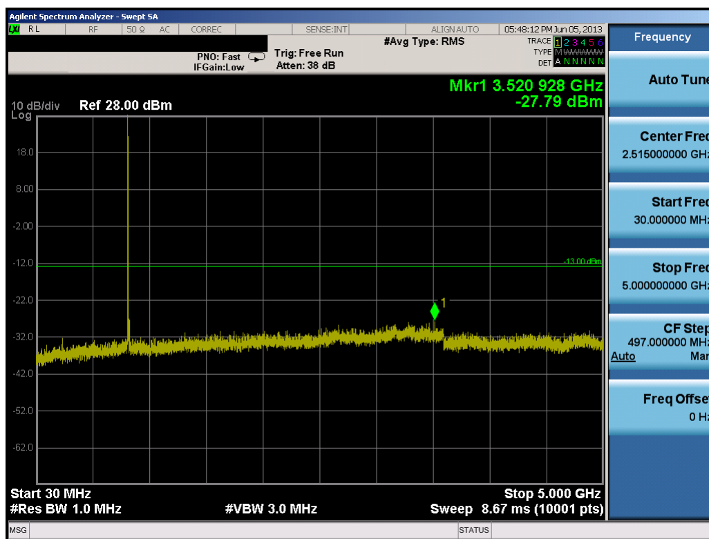
Plot 9-19. Conducted Spurious Plot (10.0MHz QPSK – RB Size 1, RB Offset 0 – Mid Channel)
