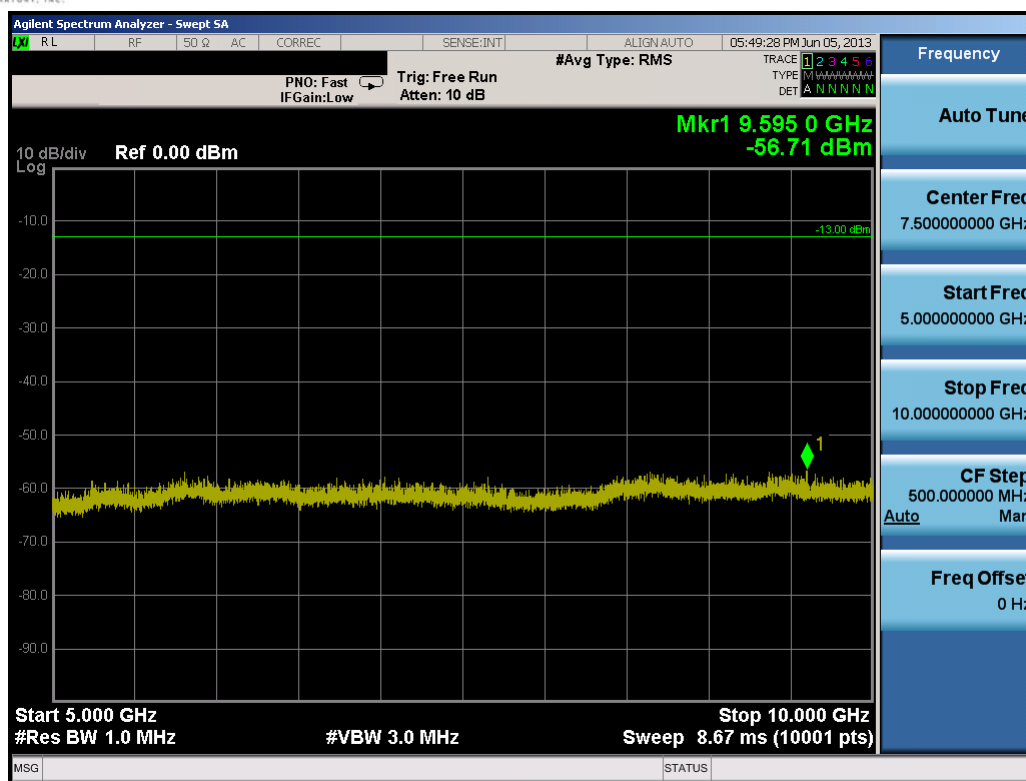
Plot 9-18. Conducted Spurious Plot (10.0MHz QPSK – RB Size 1, RB Offset 0 – Low Channel)
