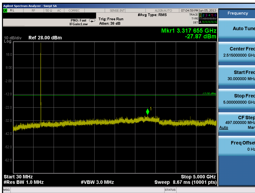
Plot 8-21. Conducted Spurious Plot (10.0MHz QPSK – RB Size 1, RB Offset 0 – High Channel)
