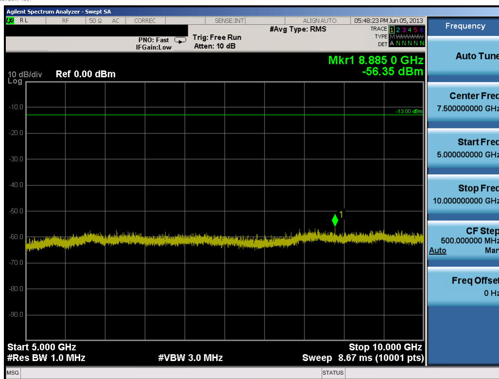
Plot 9-20. Conducted Spurious Plot (10.0MHz QPSK – RB Size 1, RB Offset 0 – Mid Channel)
