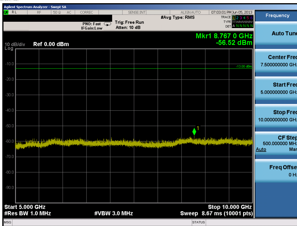
Plot 8-18. Conducted Spurious Plot (10.0MHz QPSK – RB Size 1, RB Offset 0 – Low Channel)
