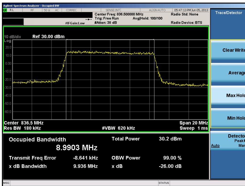
Plot 9-15. Occupied Bandwidth Plot (10.0MHz QPSK – RB Size 50)
