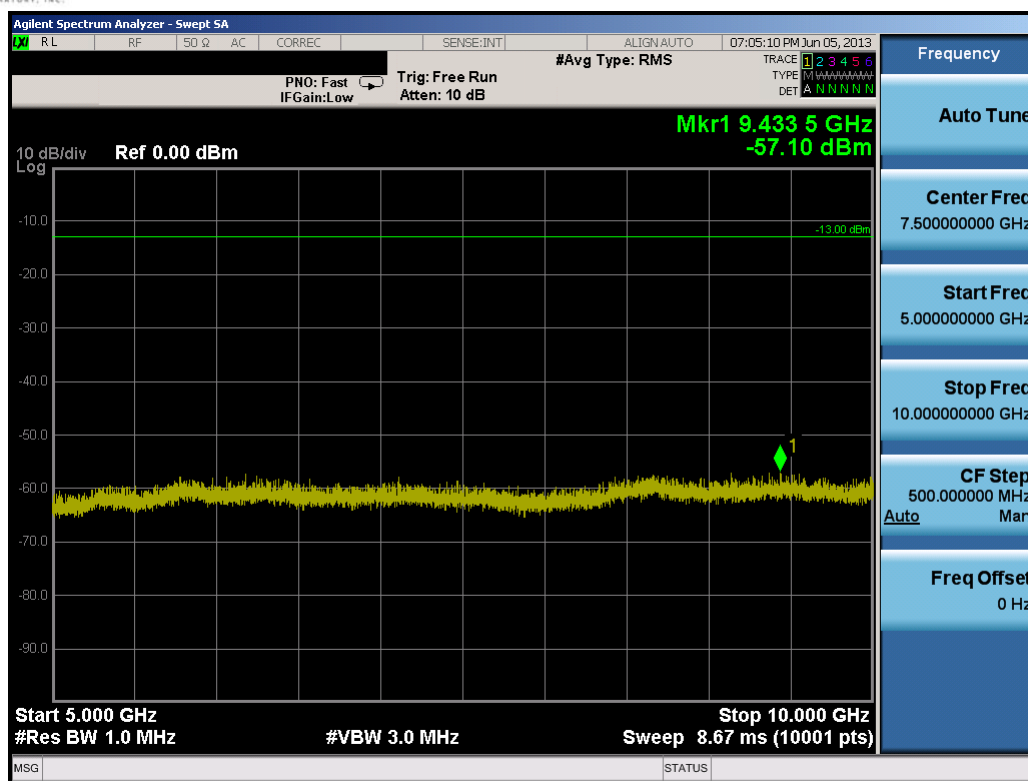
Plot 8-22. Conducted Spurious Plot (10.0MHz QPSK – RB Size 1, RB Offset 0 – High Channel)
