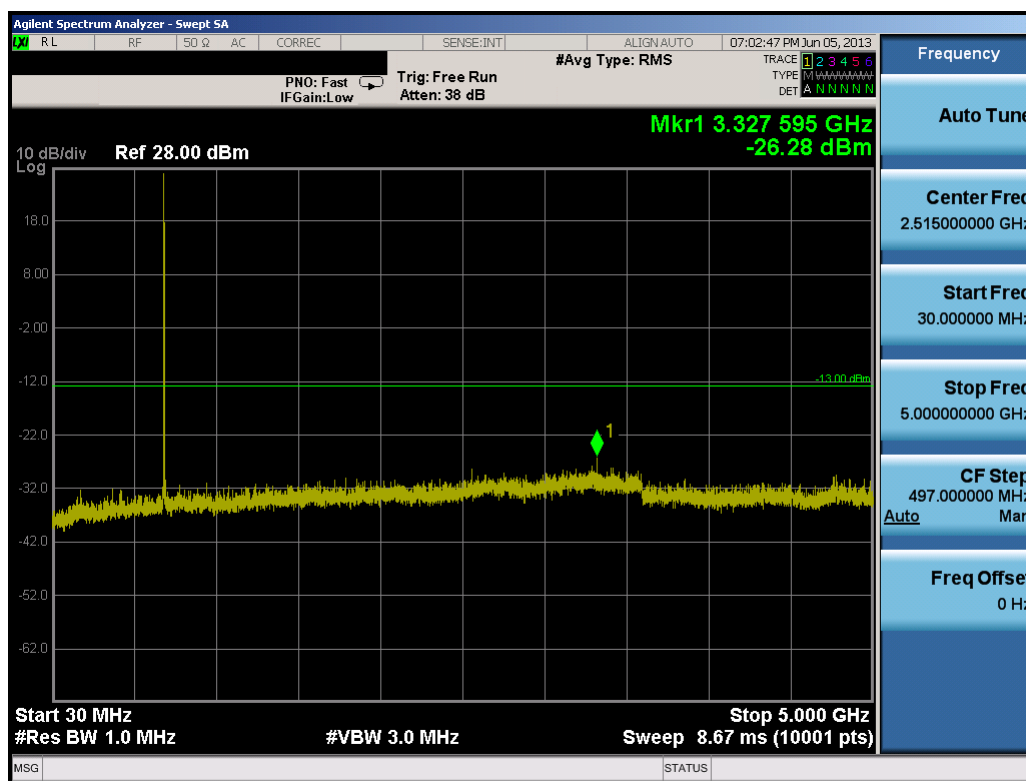
Plot 8-17. Conducted Spurious Plot (10.0MHz QPSK – RB Size 1, RB Offset 0– Low Channel)
