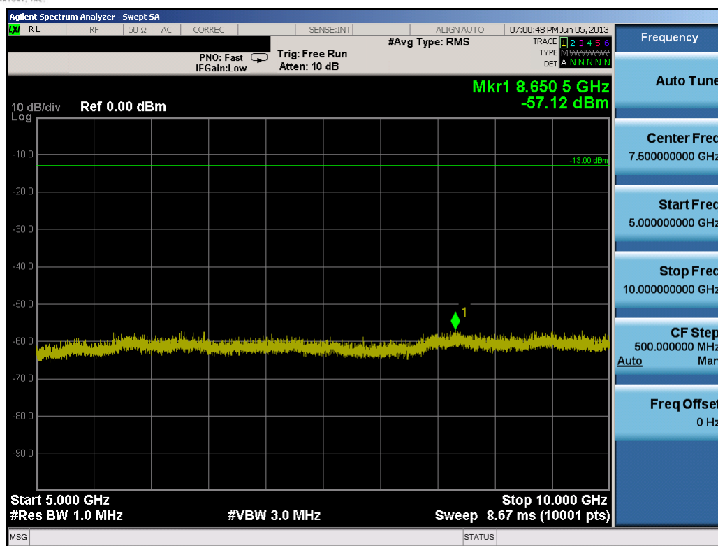
Plot 8-20. Conducted Spurious Plot (10.0MHz QPSK – RB Size 1, RB Offset 0 – Mid Channel)
