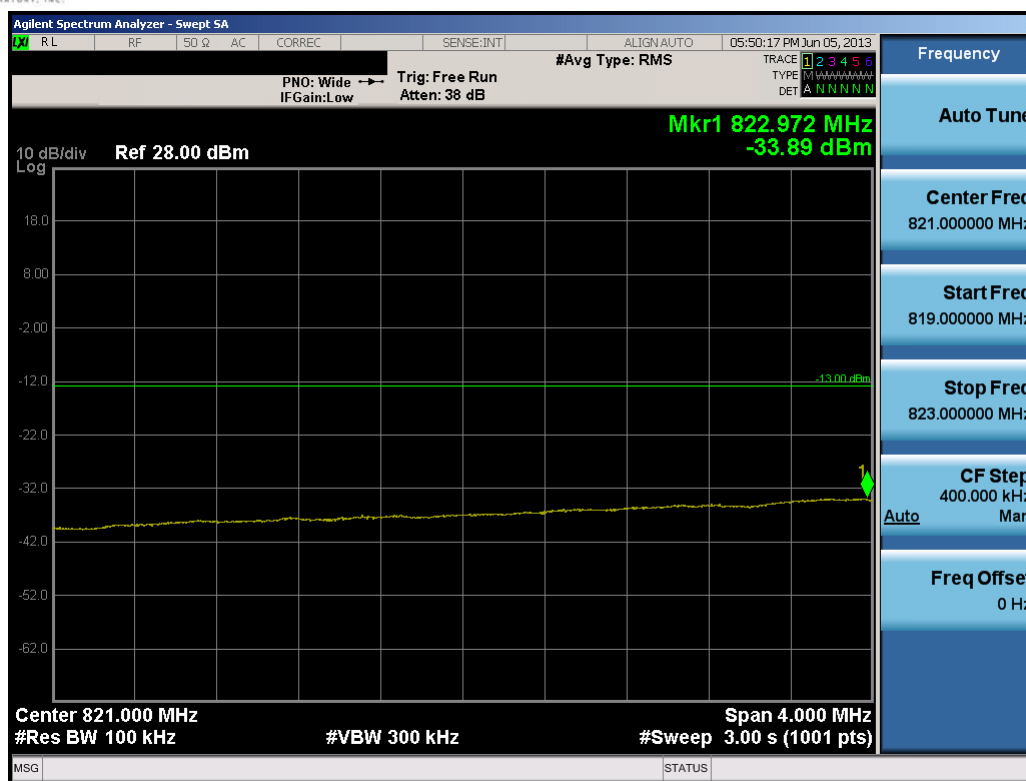
Plot 9-14. Lower Extended Band Edge Plot (10.0MHz QPSK – RB Size 50)
