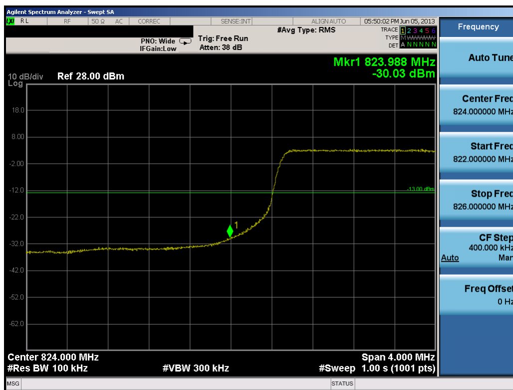
Plot 9-13. Lower Band Edge Plot (10.0MHz QPSK – RB Size 50)
