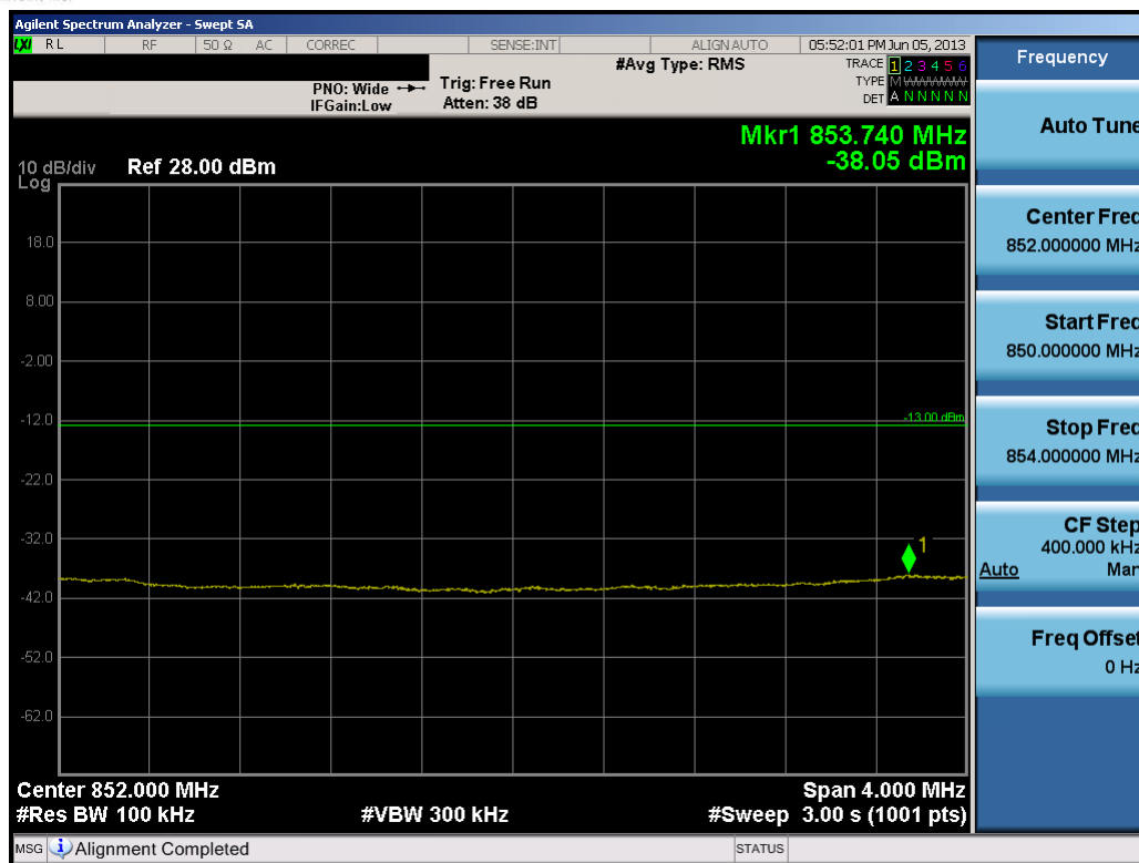
Plot 9-24. Upper Extended Band Edge Plot (10.0MHz QPSK – RB Size 50)
