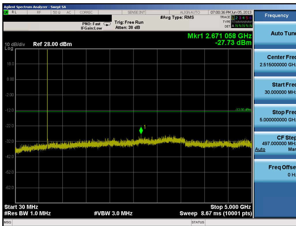
Plot 8-19. Conducted Spurious Plot (10.0MHz QPSK – RB Size 1, RB Offset 0 – Mid Channel)
