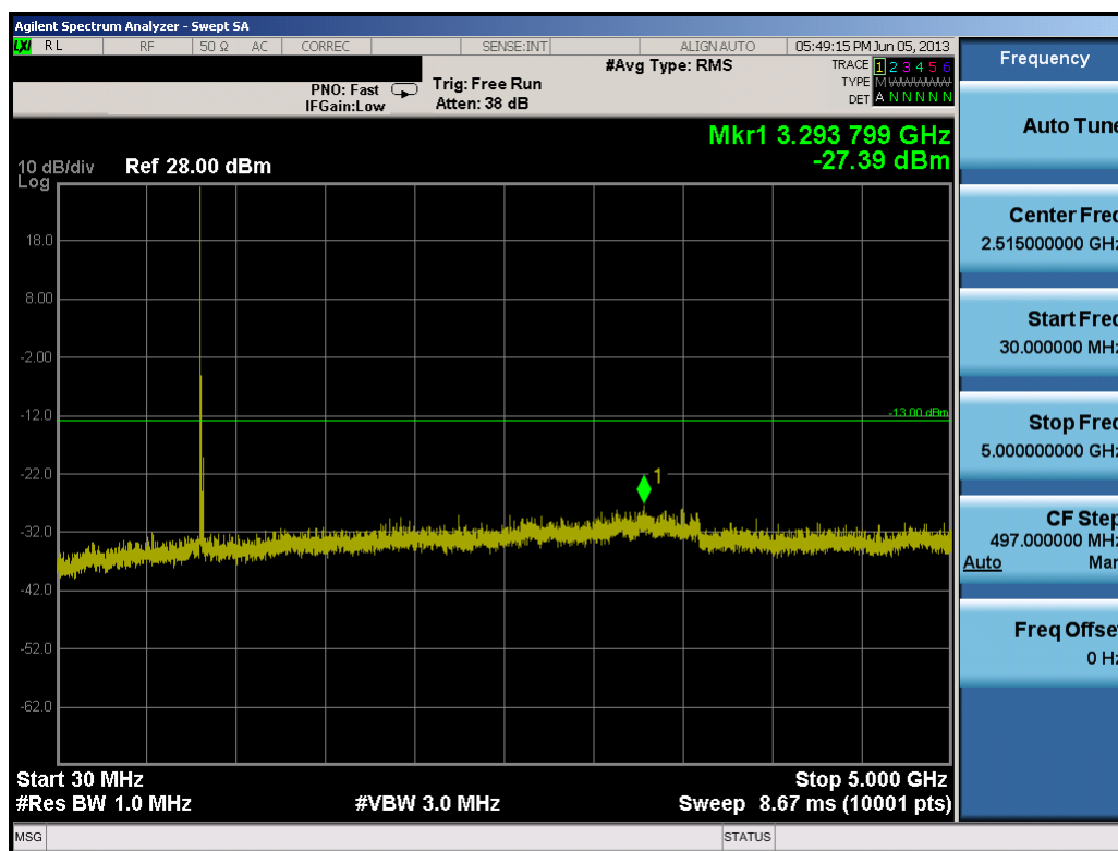
Plot 9-17. Conducted Spurious Plot (10.0MHz QPSK – RB Size 1, RB Offset 0– Low Channel)
