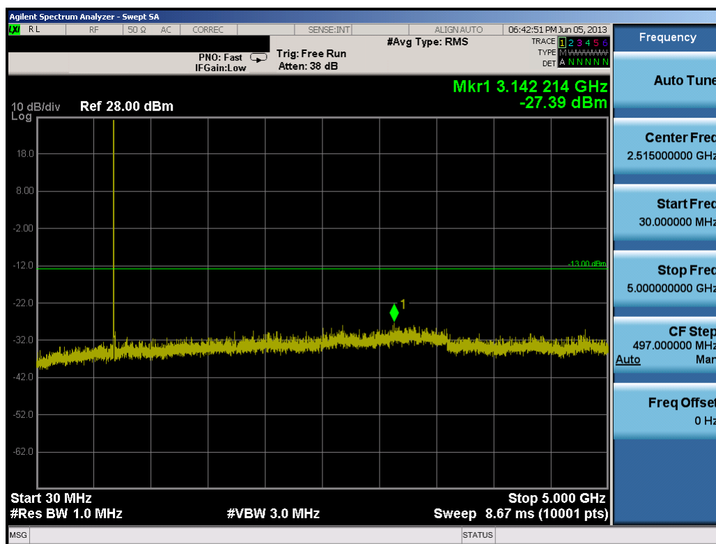
Plot 7-17. Conducted Spurious Plot (10.0MHz QPSK – RB Size 1, RB Offset 0– Low Channel)
