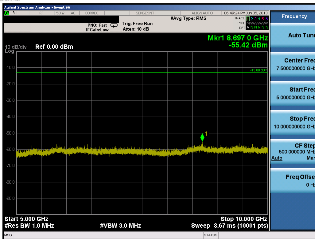
Plot 8-8. Conducted Spurious Plot (5.0MHz QPSK – RB Size 1, RB Offset 0 – Mid Channel)
