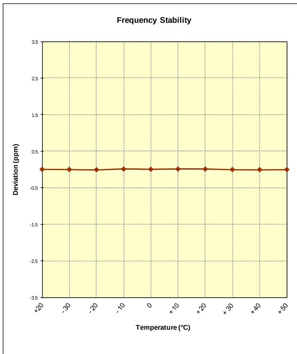
Figure 6-6. Frequency Stability Graph (Band 25)
