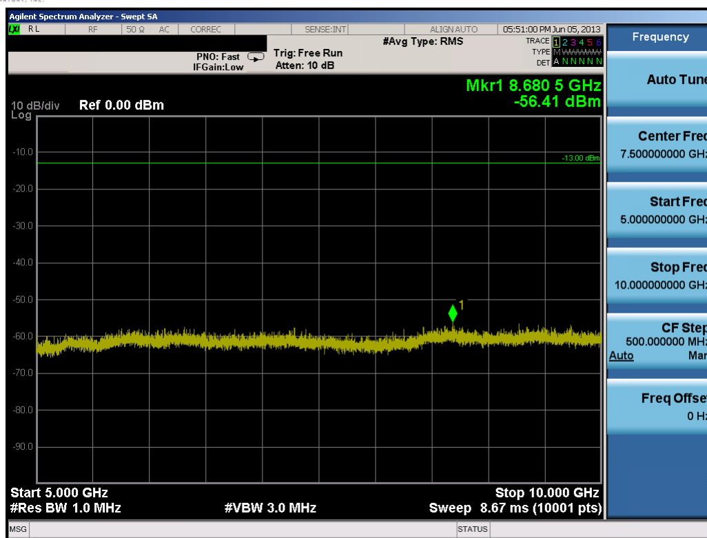
Plot 9-22. Conducted Spurious Plot (10.0MHz QPSK – RB Size 1, RB Offset 0 – High Channel)
