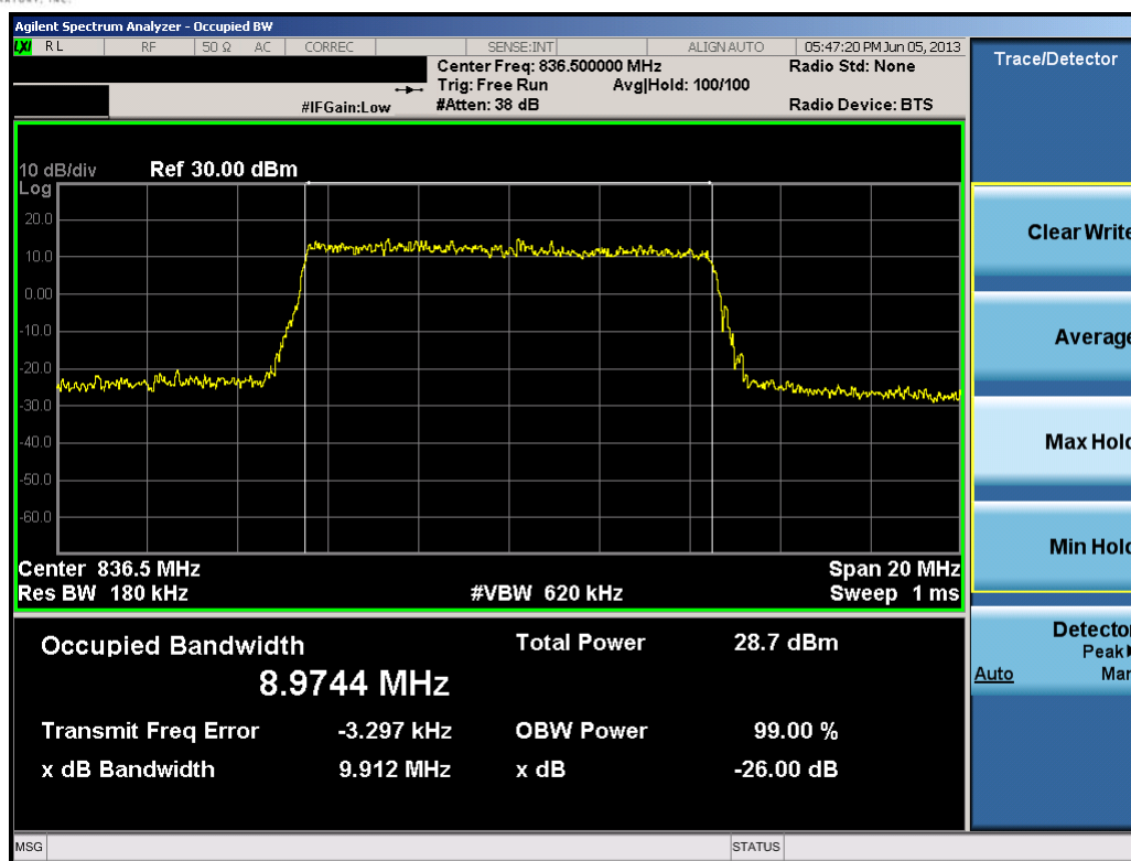
Plot 9-16. Occupied Bandwidth Plot (10.0MHz 16-QAM – RB Size 50)
