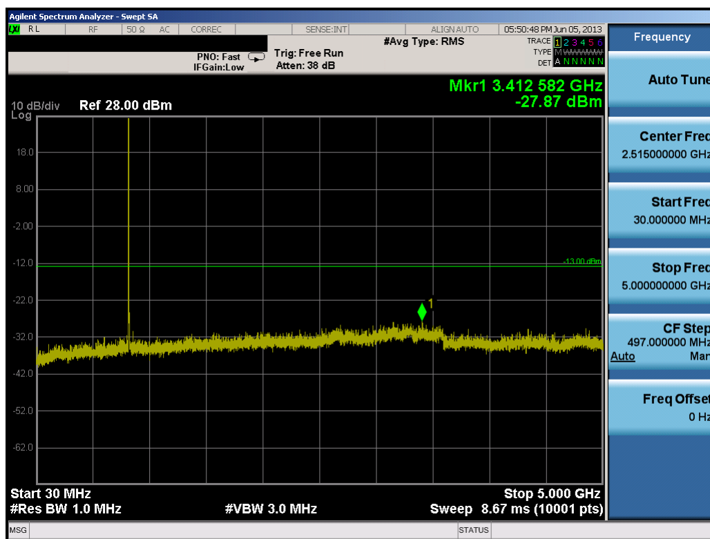
Plot 9-21. Conducted Spurious Plot (10.0MHz QPSK – RB Size 1, RB Offset 0 – High Channel)
