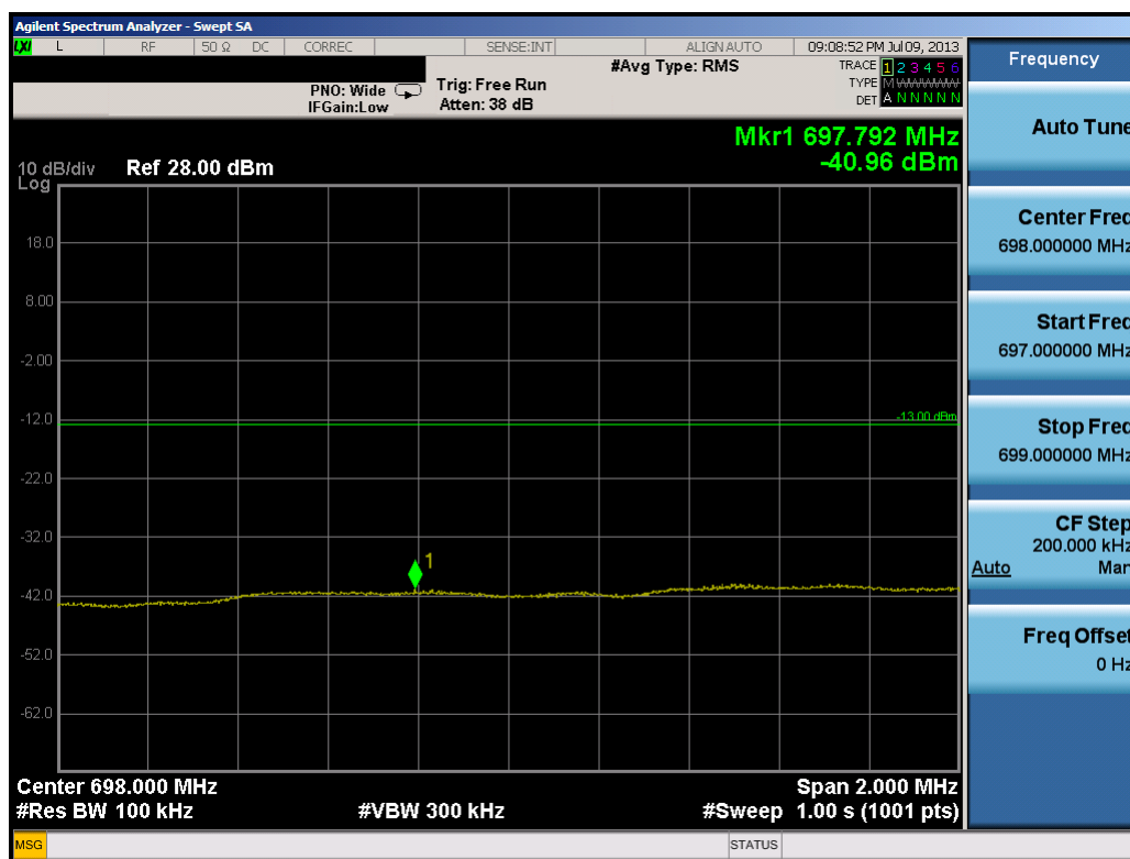
Plot 8-13. Lower Band Edge Plot (10.0MHz QPSK – RB Size 50)
