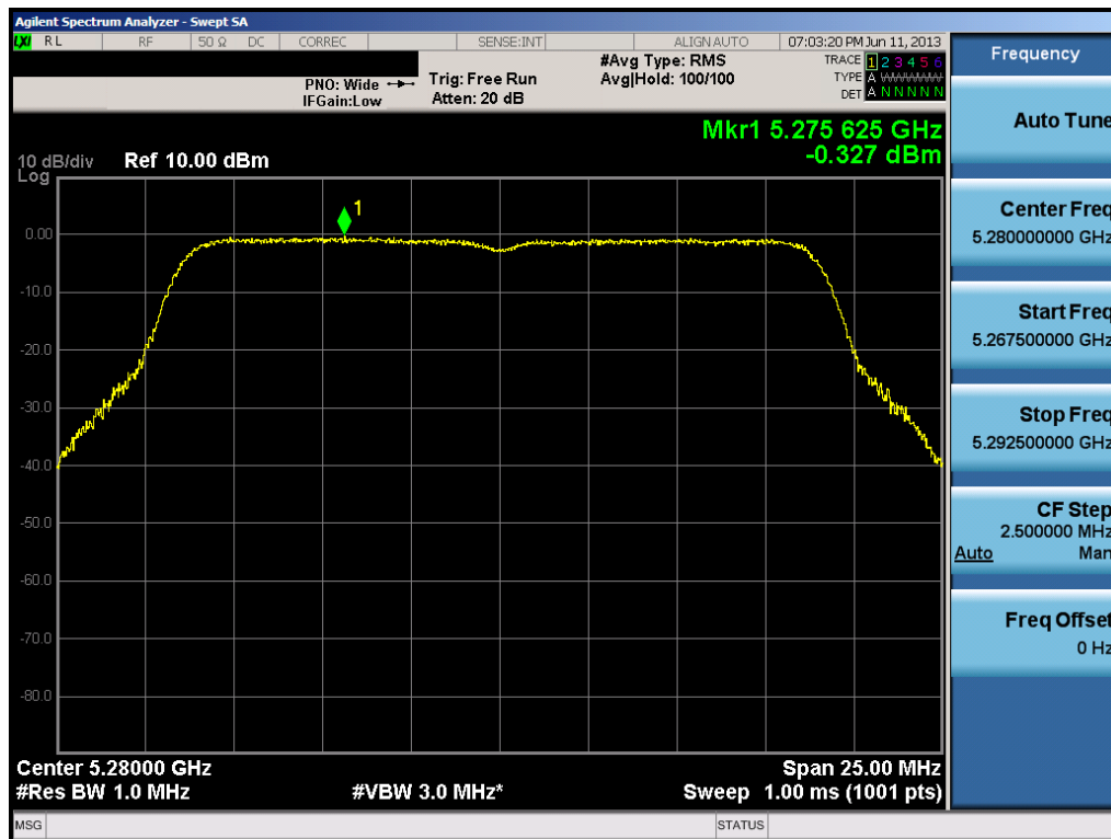
Plot 6-44. Peak Power Spectral Density Plot (20MHz BW 802.11n (UNII Band 2) – Ch. 56)
