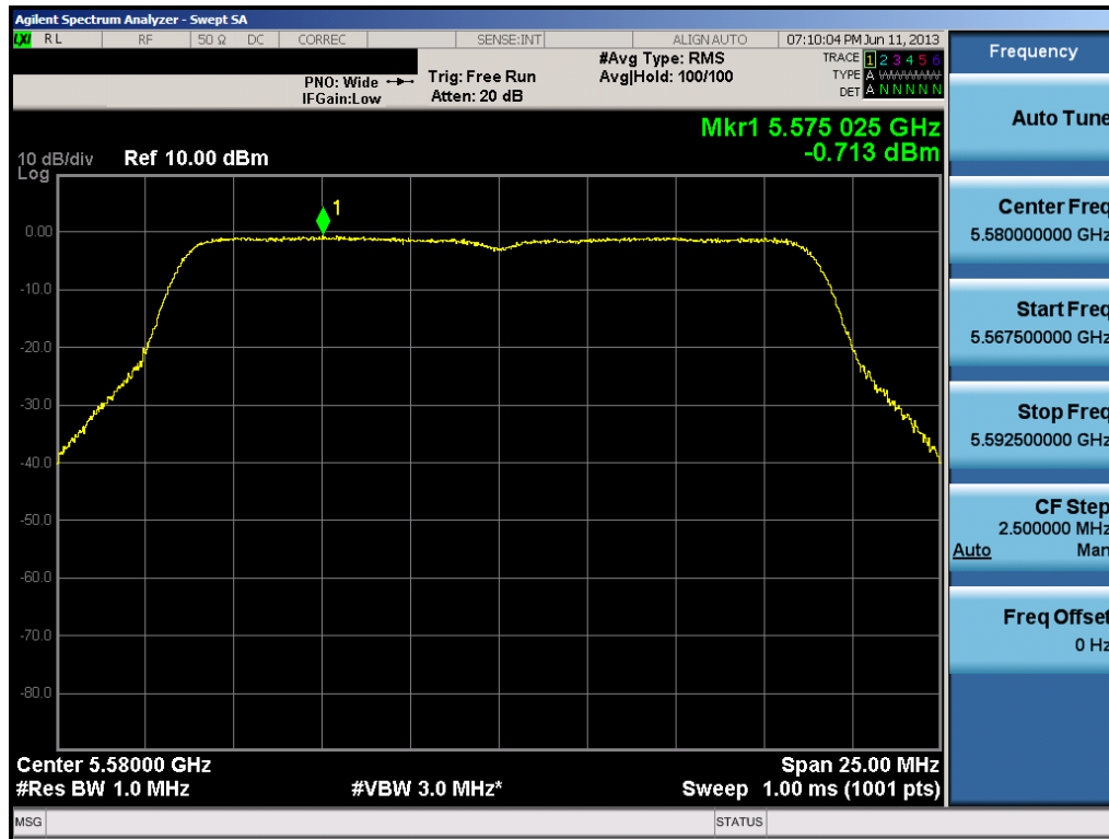
Plot 6-53. Peak Power Spectral Density Plot (20MHz BW 802.11n (UNII Band 3) – Ch. 116)
