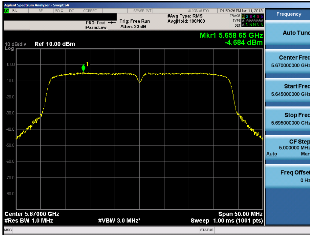
Plot 6-57. Peak Power Spectral Density Plot (40MHz BW 802.11n (UNII Band 3) – Ch. 134)
