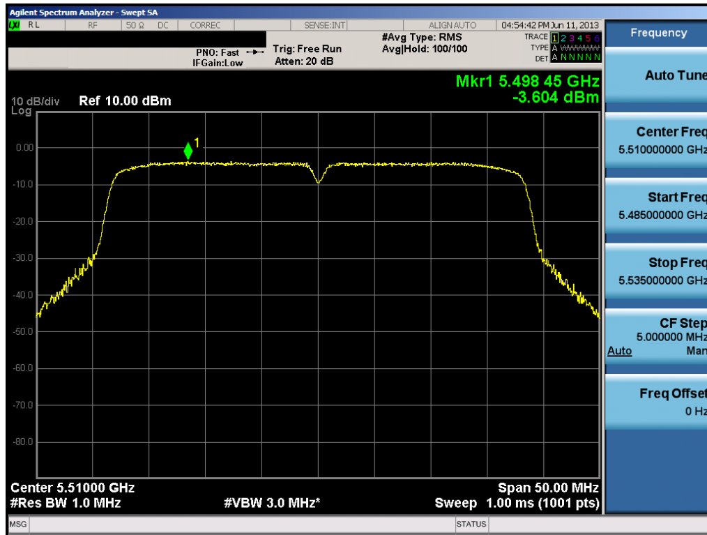
Plot 6-55. Peak Power Spectral Density Plot (40MHz BW 802.11n (UNII Band 3) – Ch. 102)
