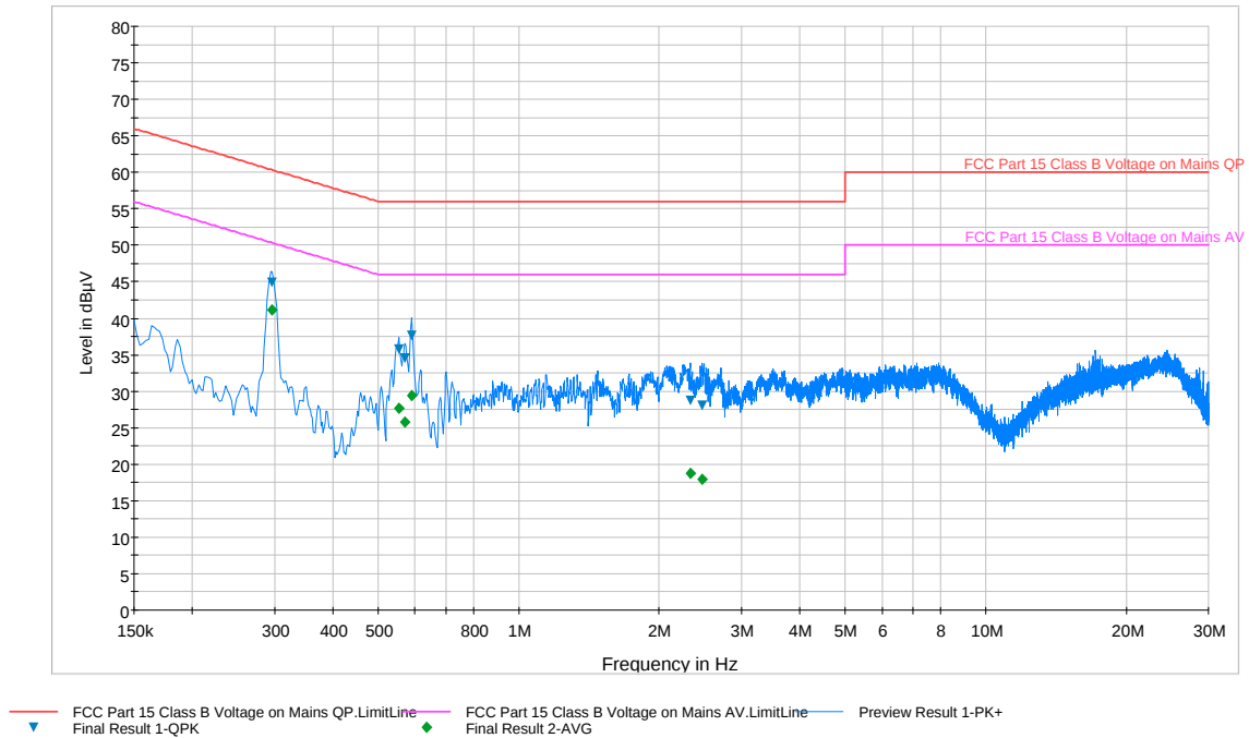
Plot 6-86. Line Conducted Plot with 802.11a UNII Band 2 (N)
