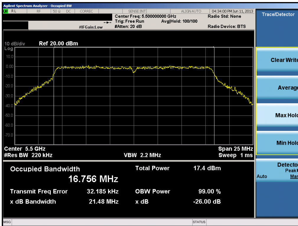
Plot 6-19. 26dB Bandwidth Plot (802.11a (UNII Band 3) – Ch. 100)
