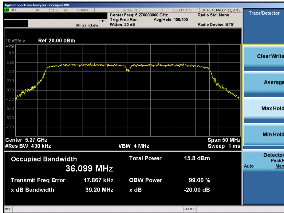
Plot 6-29. 20dB Bandwidth Plot (40MHz BW 802.11n (UNII Band 2) – Ch. 54)
