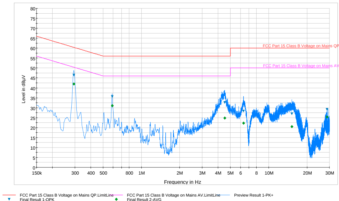
Plot 6-83. Line Conducted Plot with 802.11a UNII Band 1 (L1)
