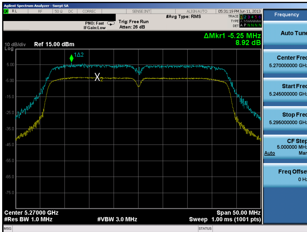
Plot 6-61. Peak Excursion Ratio Plot (40MHz BW 802.11n)
