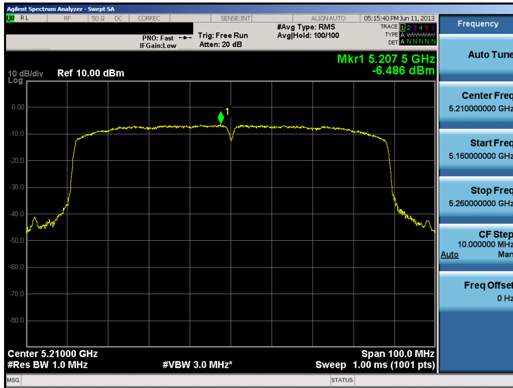
Plot 6-39. Peak Power Spectral Density Plot (80MHz BW 802.11ac (UNII Band 1) – Ch. 42)
