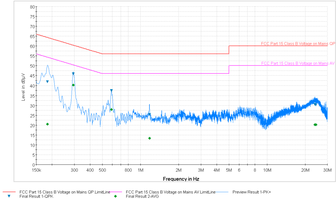
Plot 6-85. Line Conducted Plot with 802.11a UNII Band 2 (L1)
