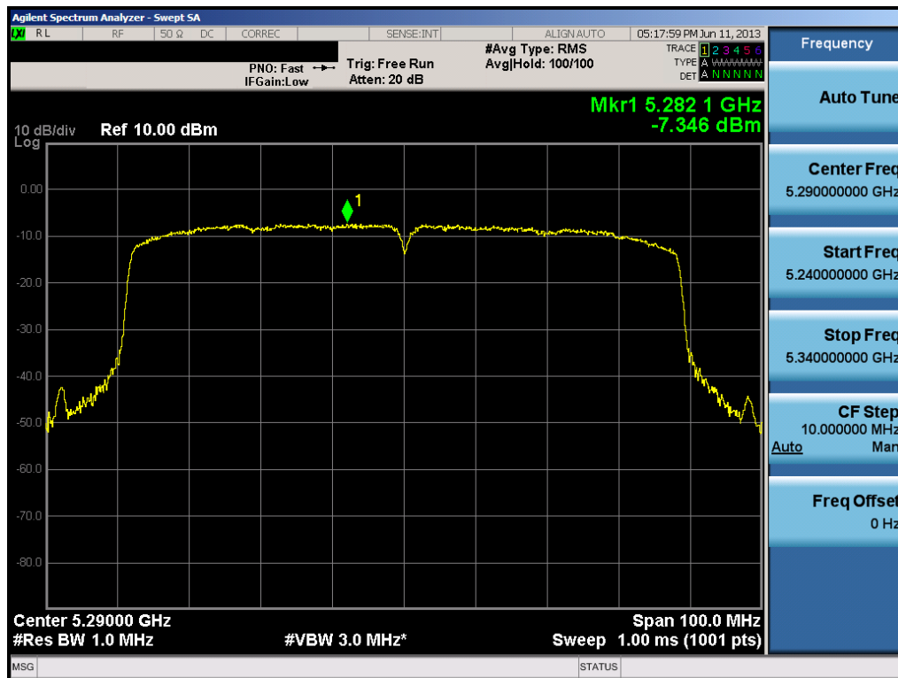
Plot 6-48. Peak Power Spectral Density Plot (80MHz BW 802.11ac (UNII Band 2) – Ch. 58)
