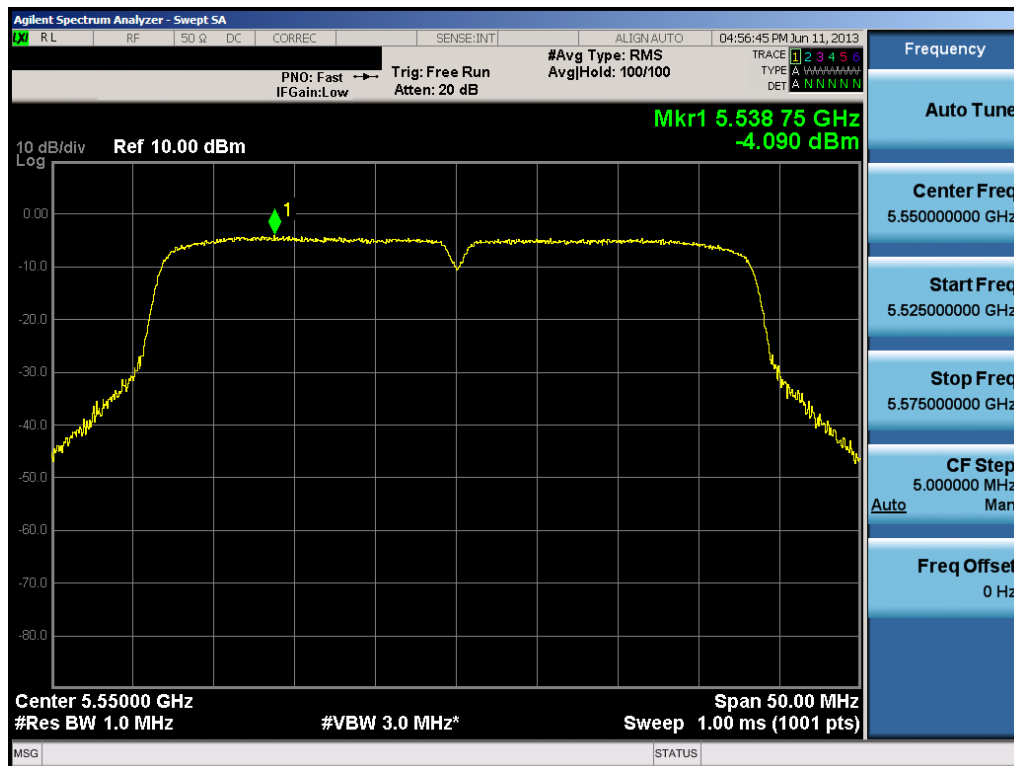
Plot 6-56. Peak Power Spectral Density Plot (40MHz BW 802.11n (UNII Band 3) – Ch. 110)
