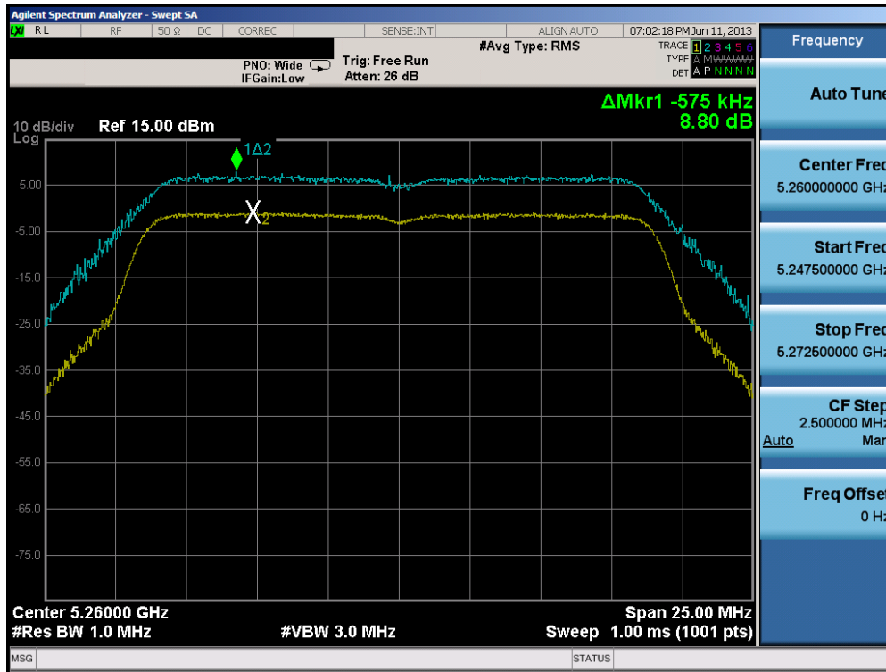
Plot 6-60. Peak Excursion Ratio Plot (20MHz BW 802.11n)
