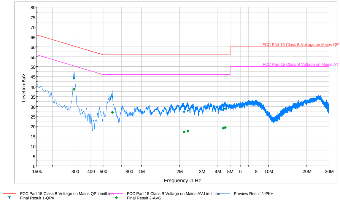
Plot 6-88. Line Conducted Plot with 802.11a UNII Band 3 (N)
