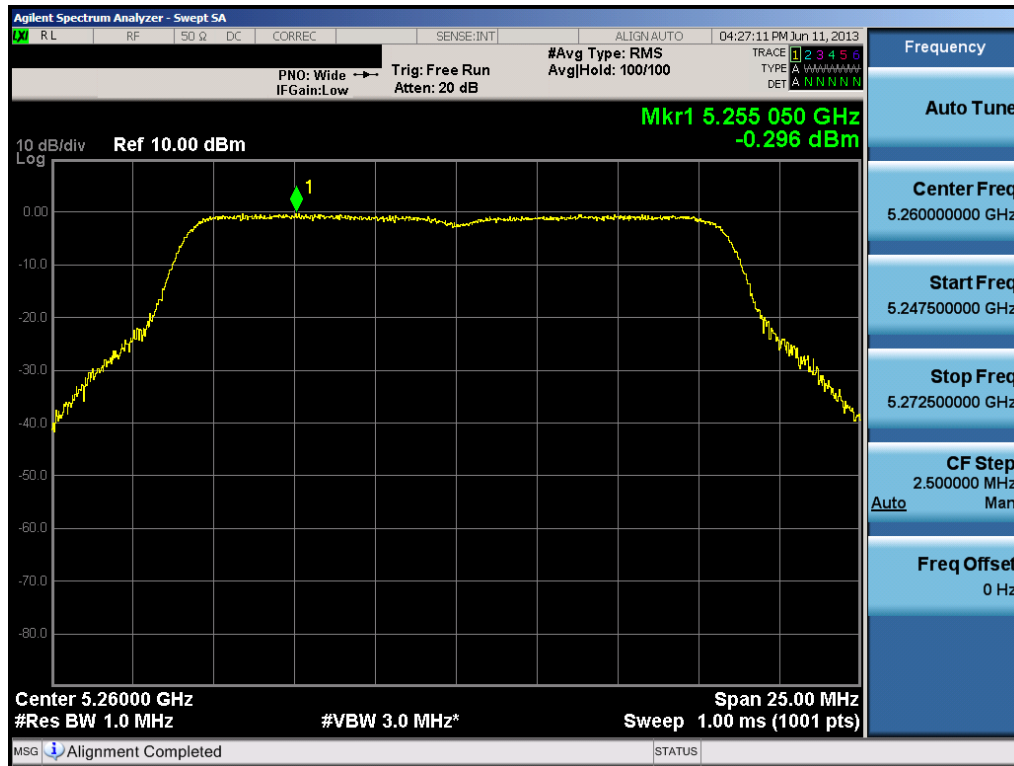
Plot 6-40. Peak Power Spectral Density Plot (802.11a (UNII Band 2) – Ch. 52)
