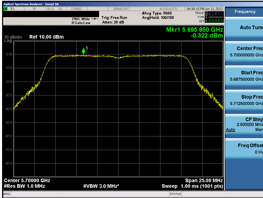
Plot 6-51. Peak Power Spectral Density Plot (802.11a (UNII Band 3) – Ch. 140)
