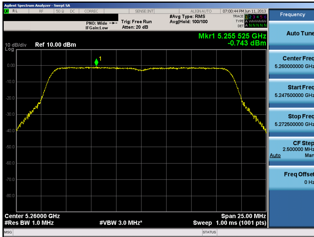
Plot 6-43. Peak Power Spectral Density Plot (20MHz BW 802.11n (UNII Band 2) – Ch. 52)
