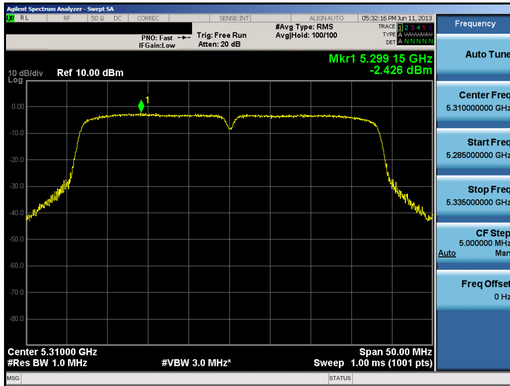
Plot 6-47. Peak Power Spectral Density Plot (40MHz BW 802.11n (UNII Band 2) – Ch. 62)
