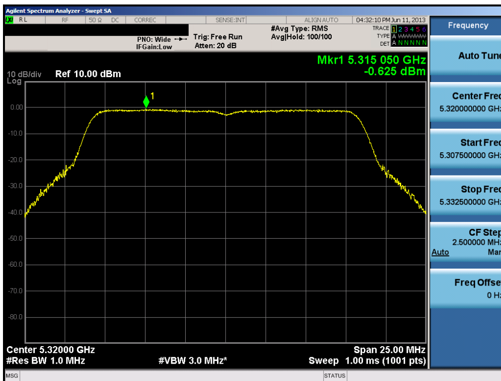
Plot 6-42. Peak Power Spectral Density Plot (802.11a (UNII Band 2) – Ch. 64)
