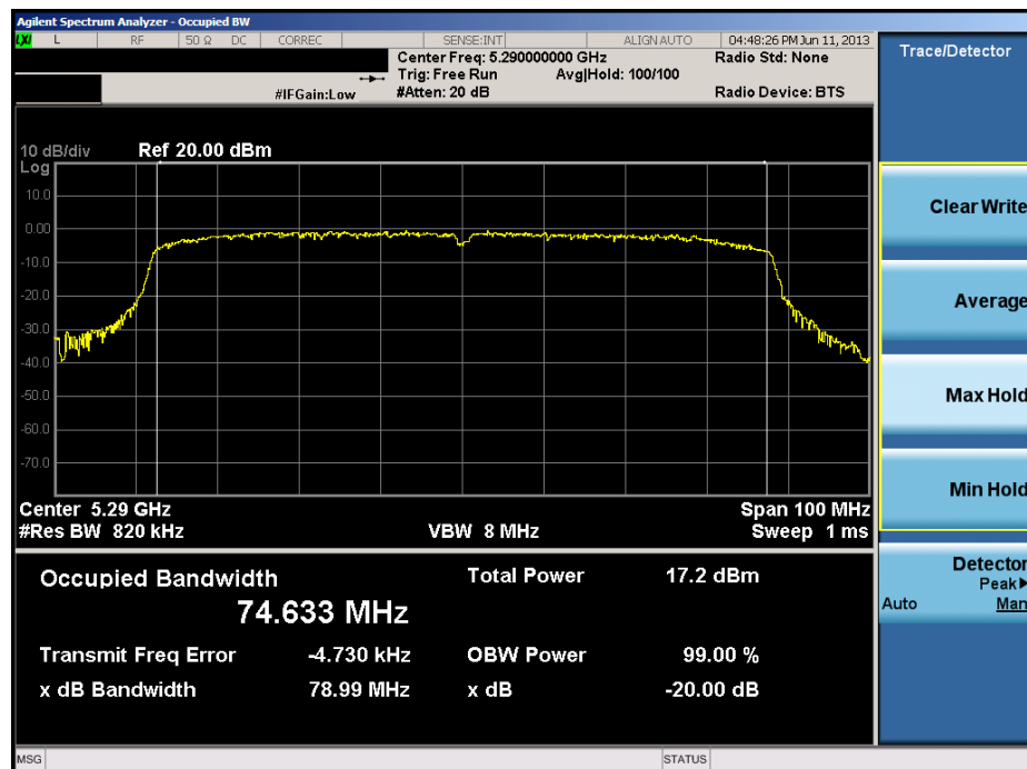
Plot 6-30. 20dB Bandwidth Plot (80MHz BW 802.11n (UNII Band 2) – Ch. 58)
