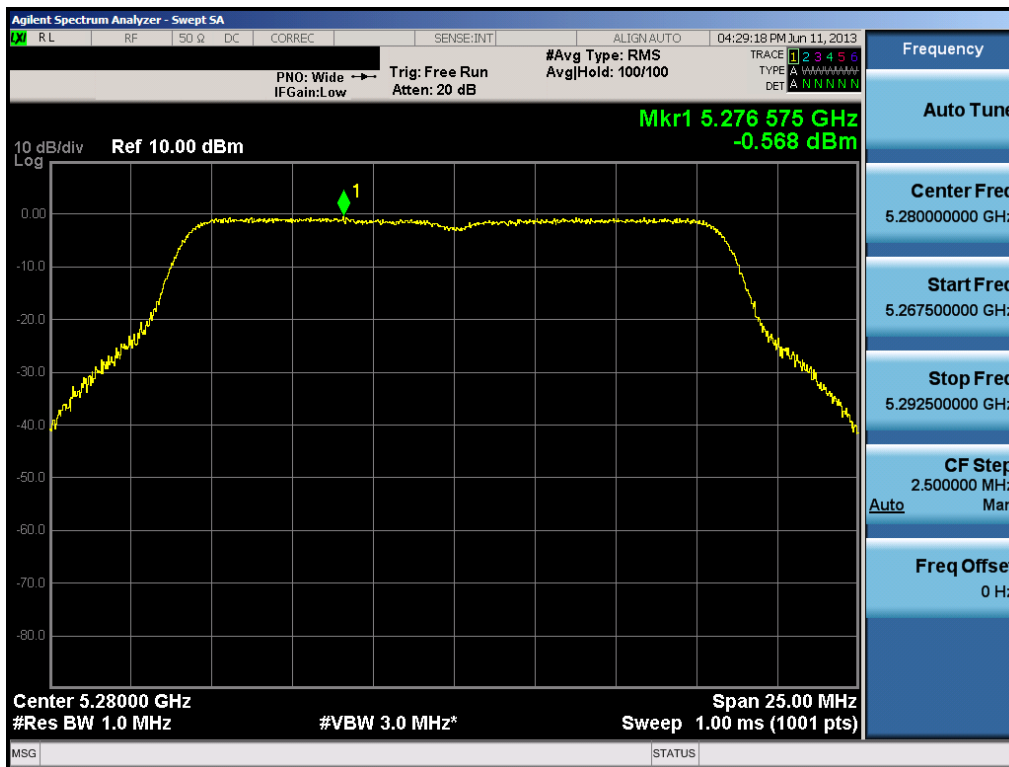
Plot 6-41. Peak Power Spectral Density Plot (802.11a (UNII Band 2) – Ch. 56)
