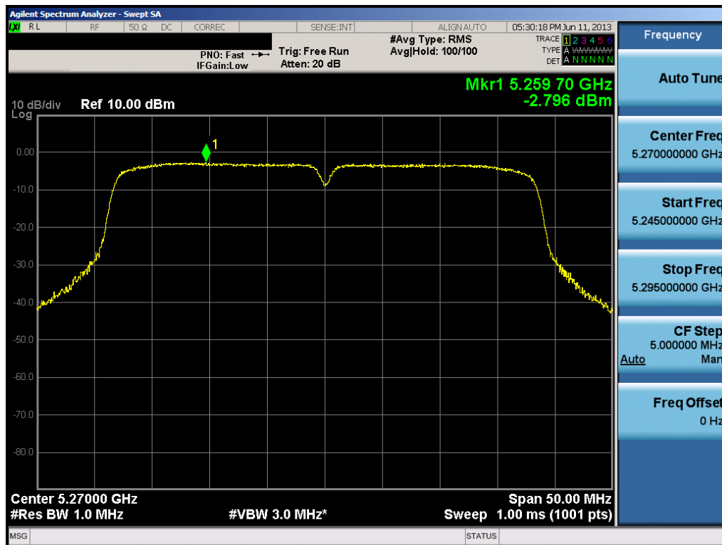
Plot 6-46. Peak Power Spectral Density Plot (40MHz BW 802.11n (UNII Band 2) – Ch. 54)
