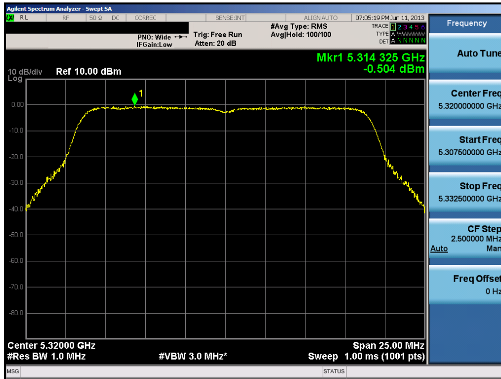
Plot 6-45. Peak Power Spectral Density Plot (20MHz BW 802.11n (UNII Band 2) – Ch. 64)
